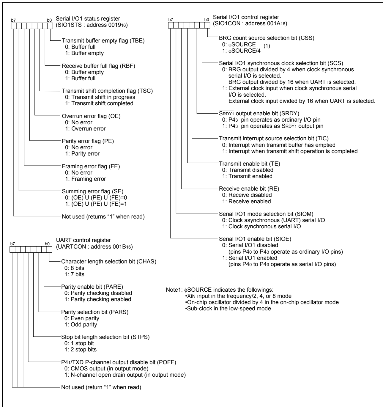
Fig. 37 Structure of serial I/O1 related registers
