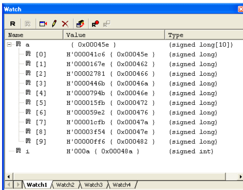
Figure 6.19 [Watch] Window (Displaying Array Elements)
