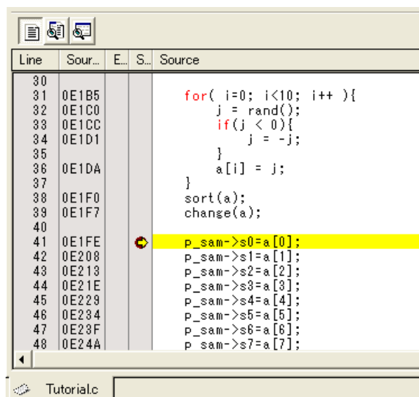
Figure 6.32 [Source] Window at Execution Stop (PC Break)
