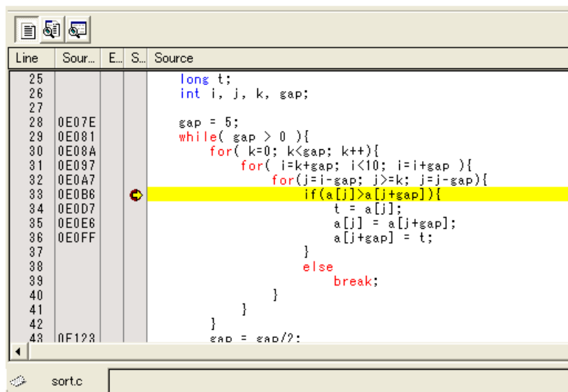
Figure 6.39 [Source] Window (PC Breakpoint Setting)
