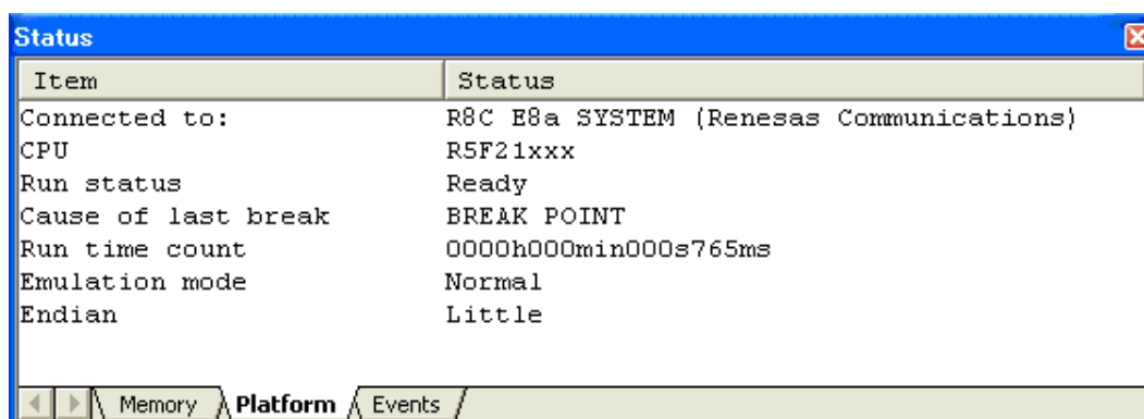
Figure 6.33 Displayed Contents of the [Status] Window (PC Break)
