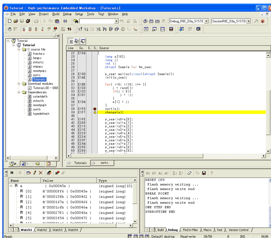
Figure 6.23 [High-performance Embedded Workshop] Window (Step Out)
