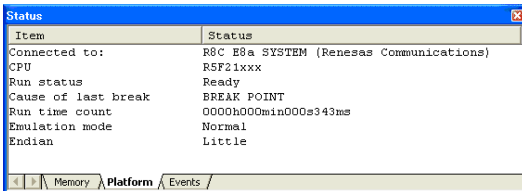
Figure 6.11 [Status] Window
