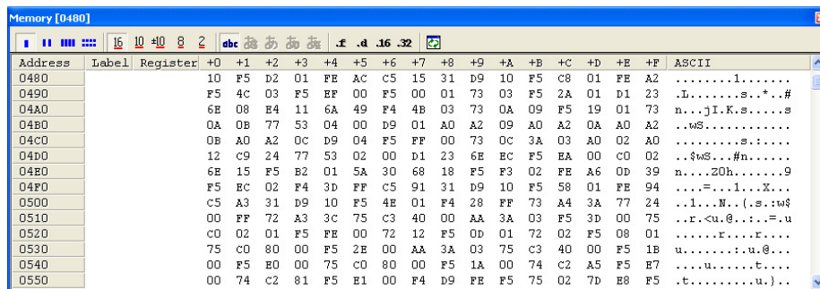
Figure 6.3 [Memory] Window
