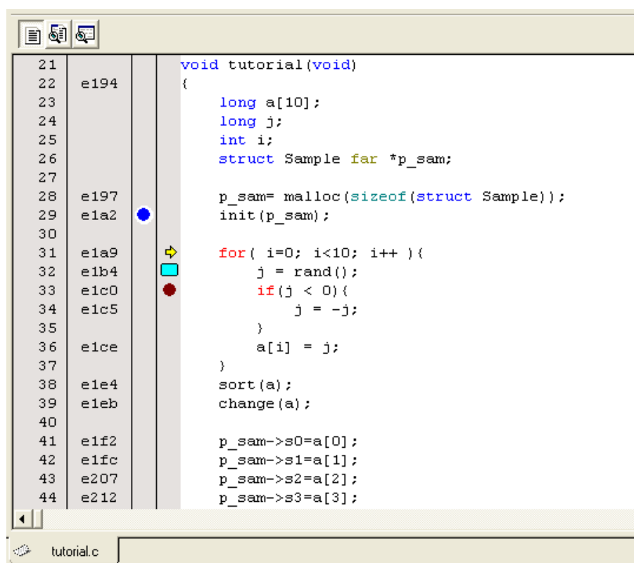
Figure 5.2 [Source] Window
