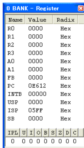
Figure 6.7 [Register] Window
