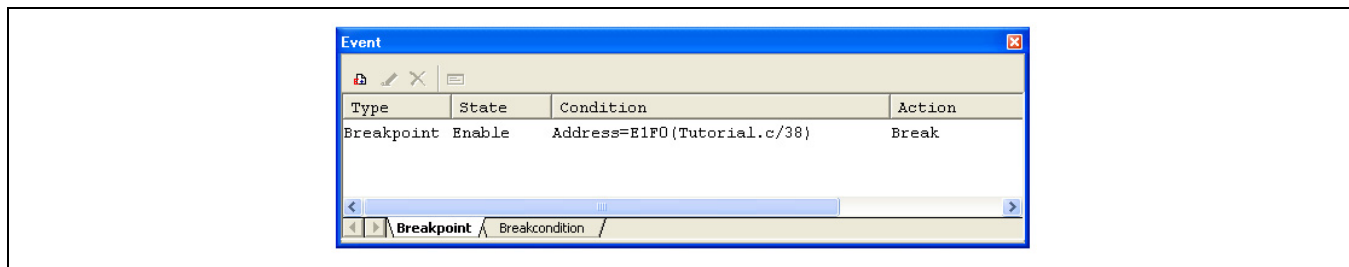
Figure 6.12 [Event] Window
