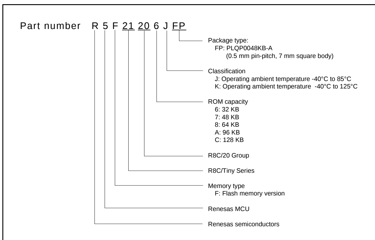
Figure 1.2 Type Number, Memory Size, and Package of R8C/20 Group
