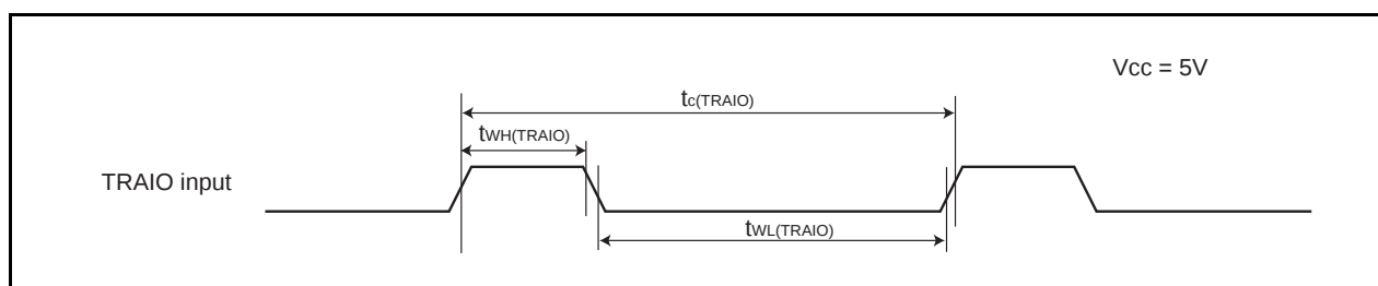
Figure 5.9 TRAIO Input and \overline{INT1} Input Timing Diagram when V_{CC} = 5\text{ V}
