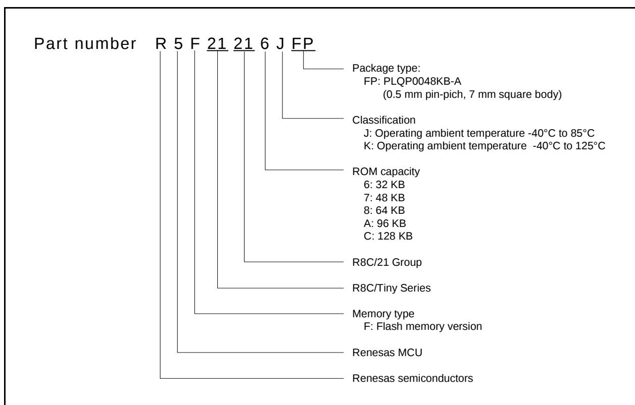
Figure 1.3 Type Number, Memory Size, and Package of R8C/21 Group
