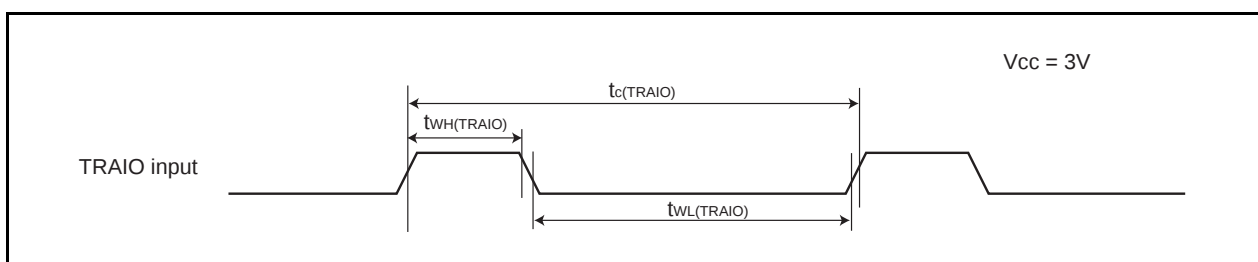
Figure 5.13 TRAIO Input and \overline{\text{INT1}} Input Timing Diagram when V_{CC} = 3\text{ V}
