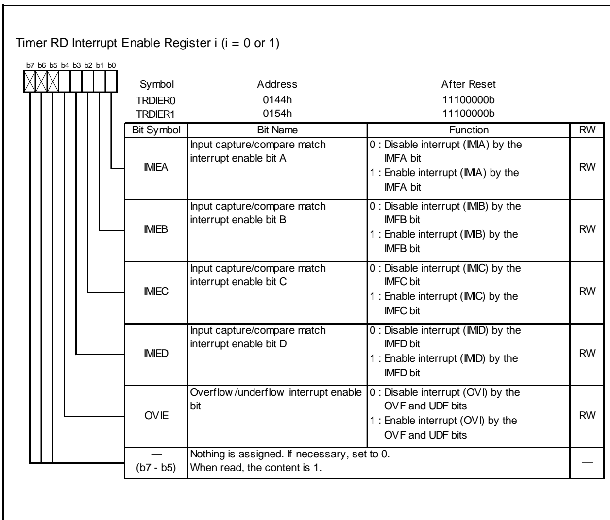
Figure 14.90 Registers TRDIER0 to TRDIER1 in Complementary PWM Mode
