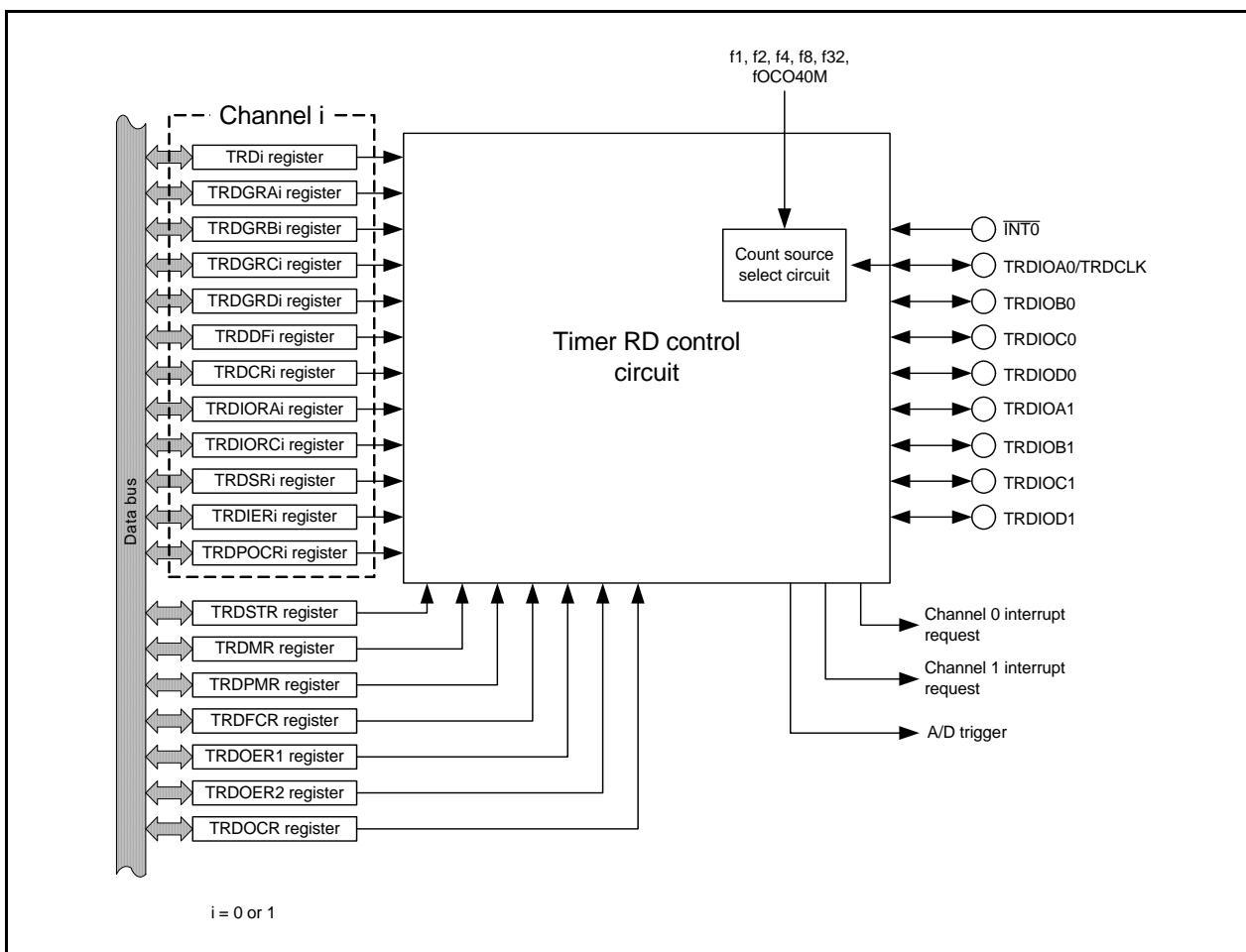
Figure 14.24 Block Diagram of Timer RD
