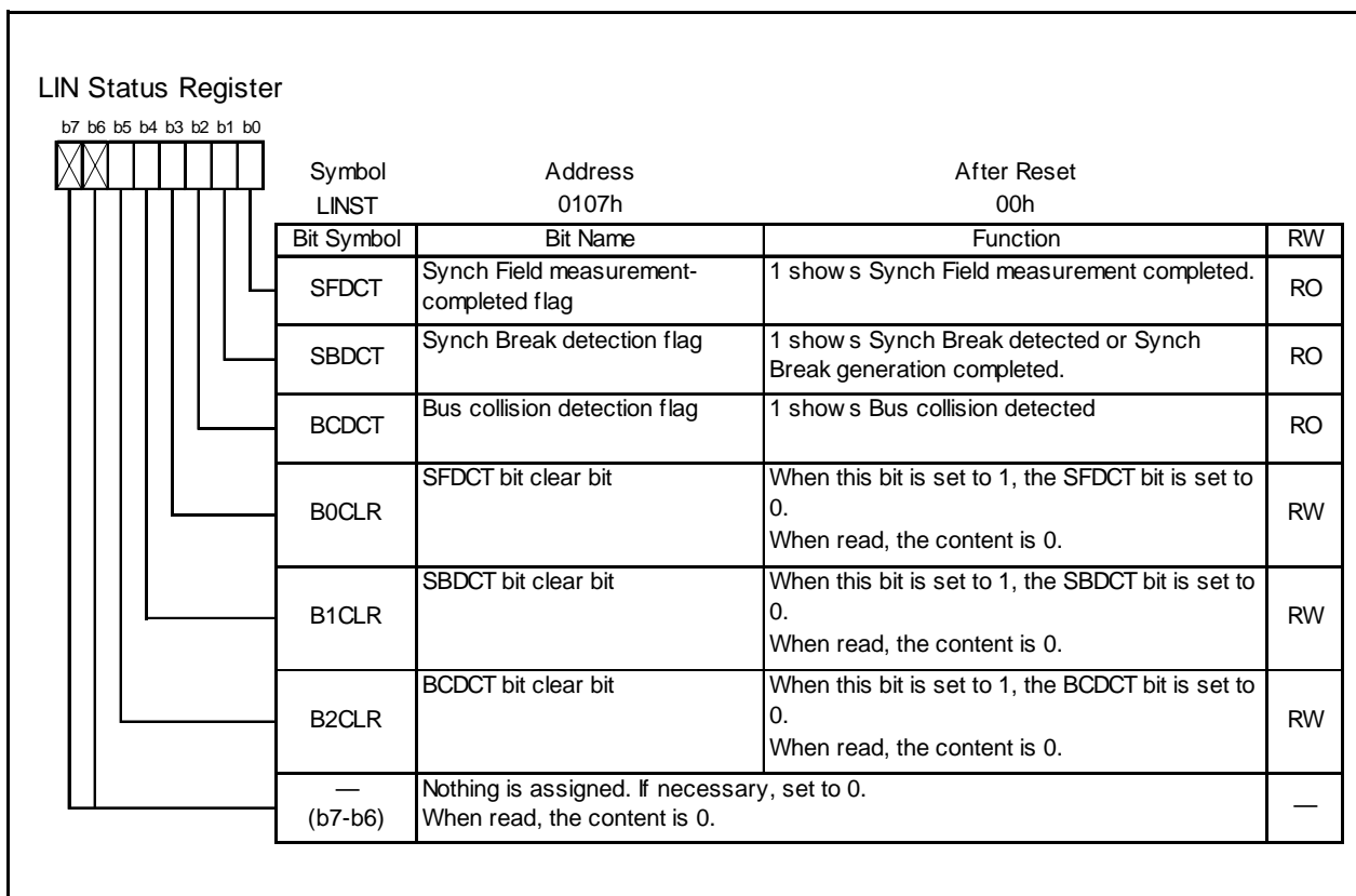
Figure 17.3 LINST Register
