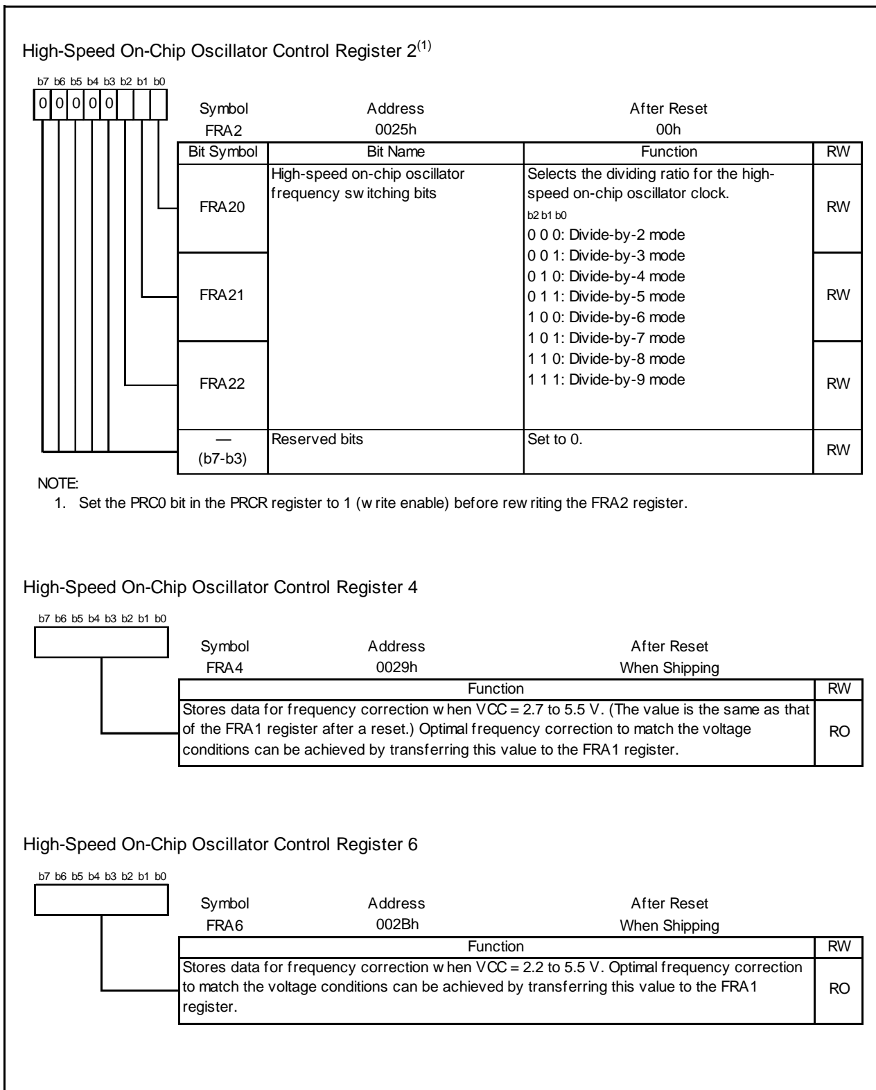
Figure 10.6 Registers FRA2, FRA4, and FRA6
