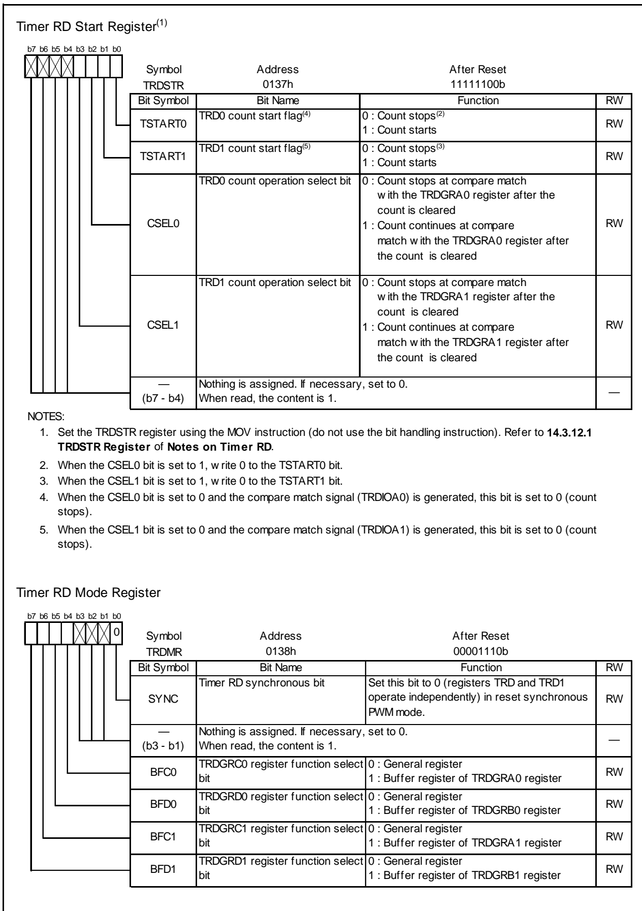
Figure 14.74 Registers TRDSTR and TRDMR in Reset Synchronous PWM Mode
