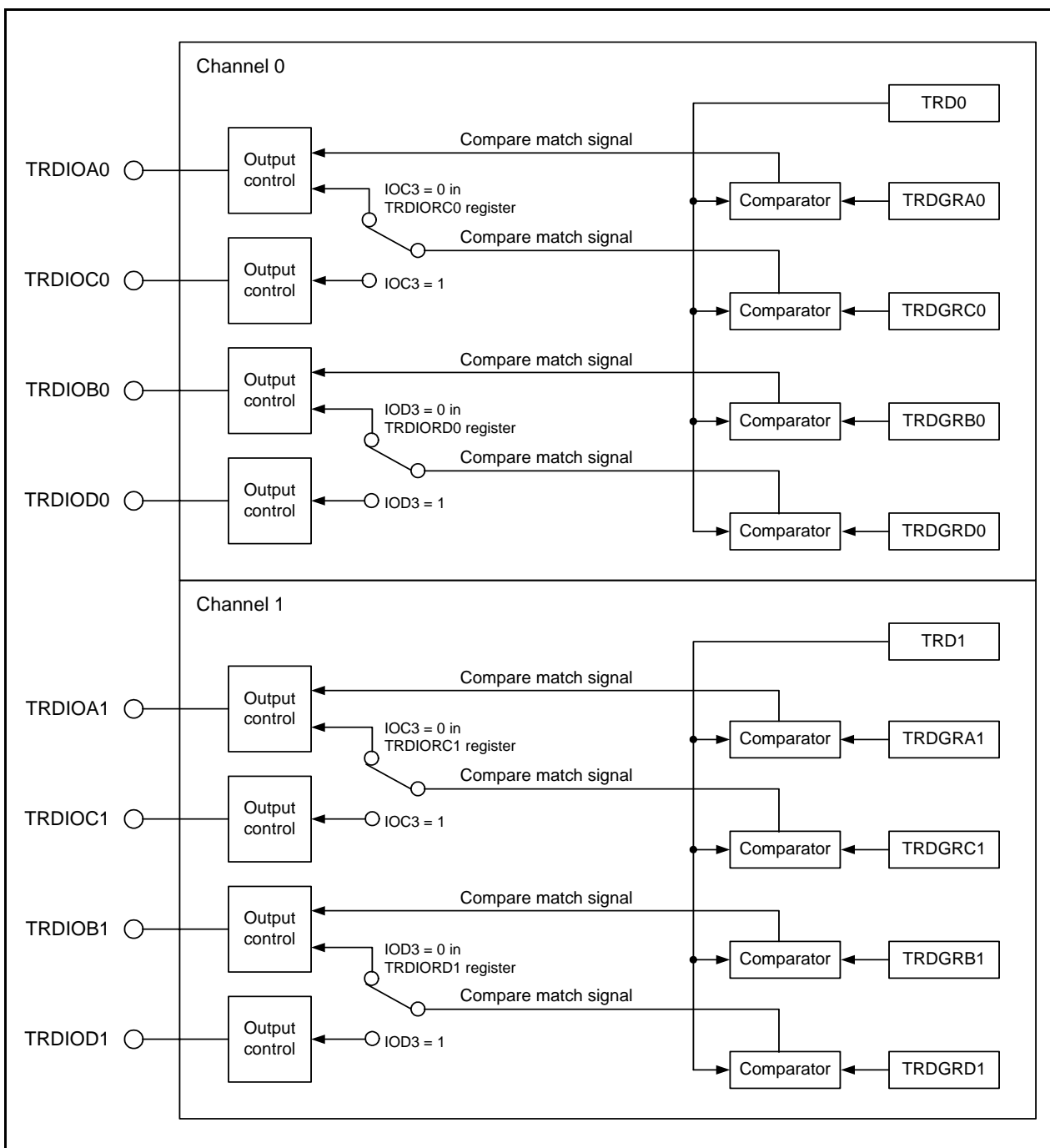
Figure 14.58 Changing Output Pins in Registers TRDGRCi and TRDGRDi
