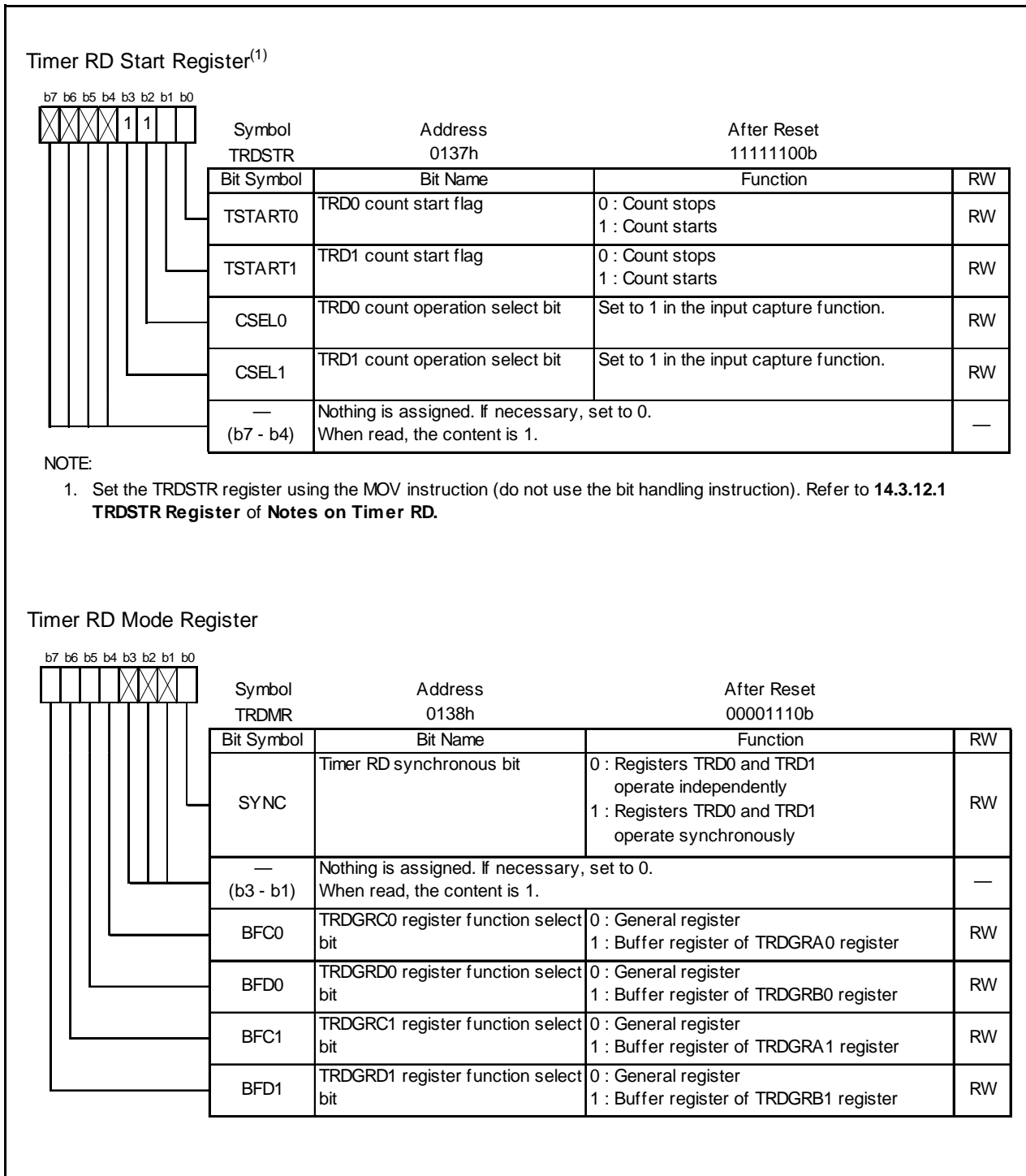
Figure 14.31 Registers TRDSTR and TRDMR in Input Capture Function
