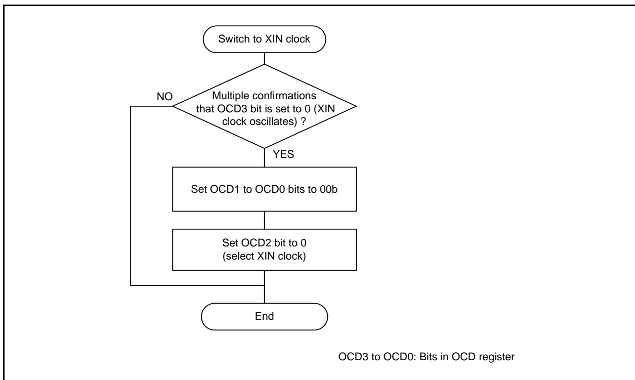
Figure 10.15 Procedure for Switching Clock Source from Low-Speed On-Chip Oscillator to XIN Clock
