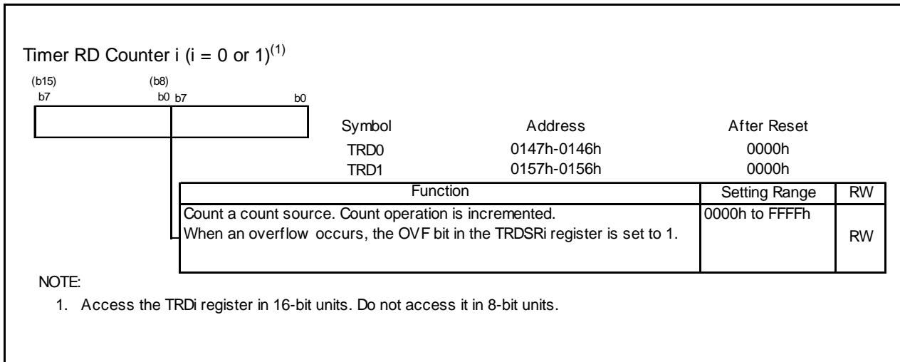
Figure 14.69 Registers TRD0 to TRD1 in PWM Mode
