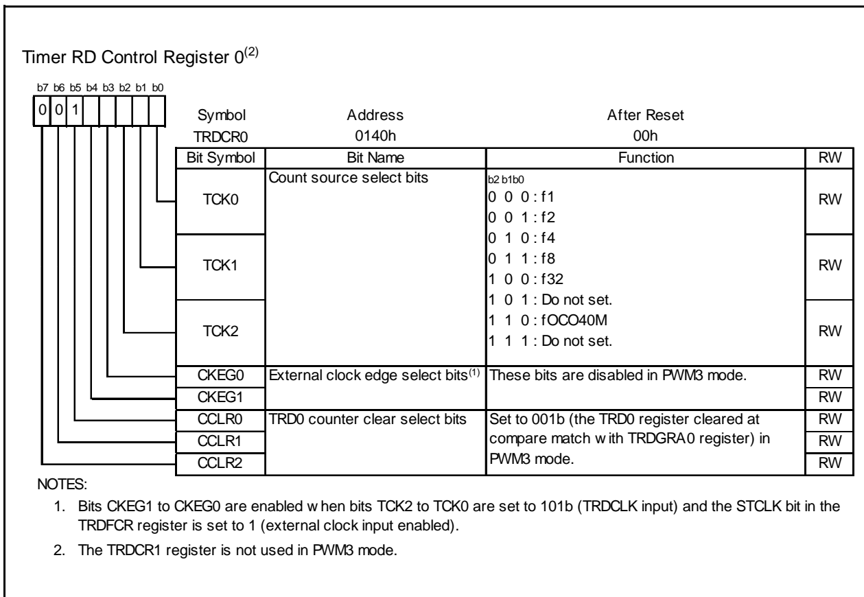
Figure 14.101 TRDCR0 Register in PWM3 Mode
