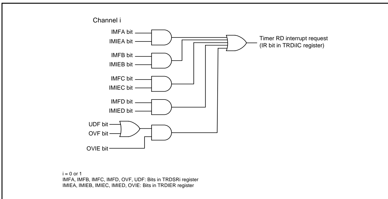
Figure 14.107 Block Diagram of Timer RD Interrupt
