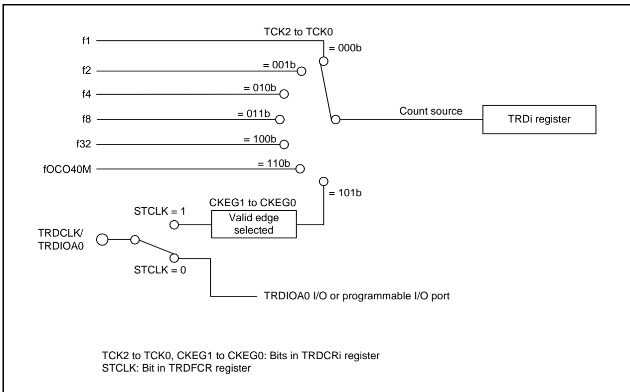
Figure 14.25 Block Diagram of Count Source
