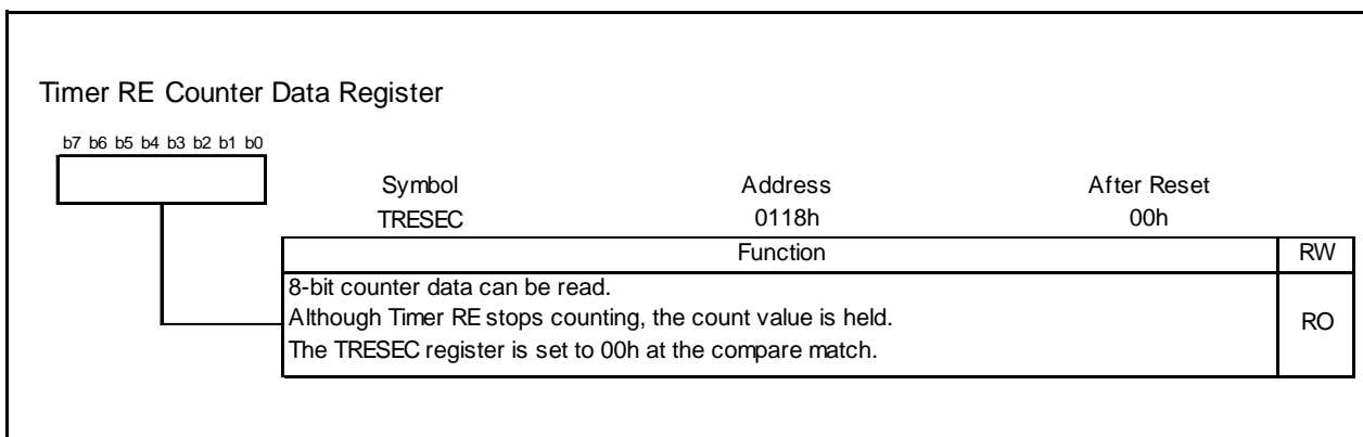
Figure 14.123 TRESEC Register in Output Compare Mode
