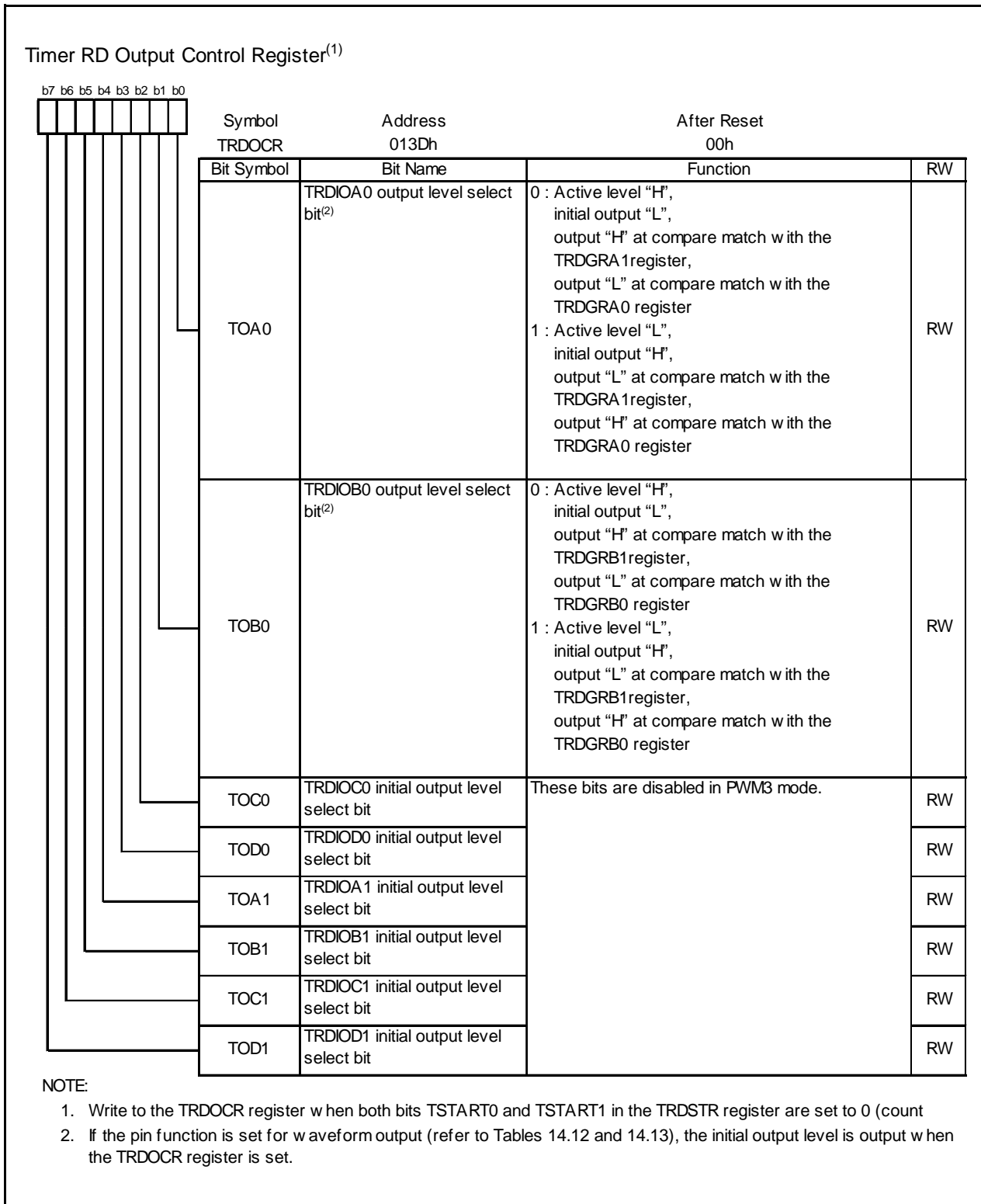
Figure 14.100 TRDOCR Register in PWM3 Mode
