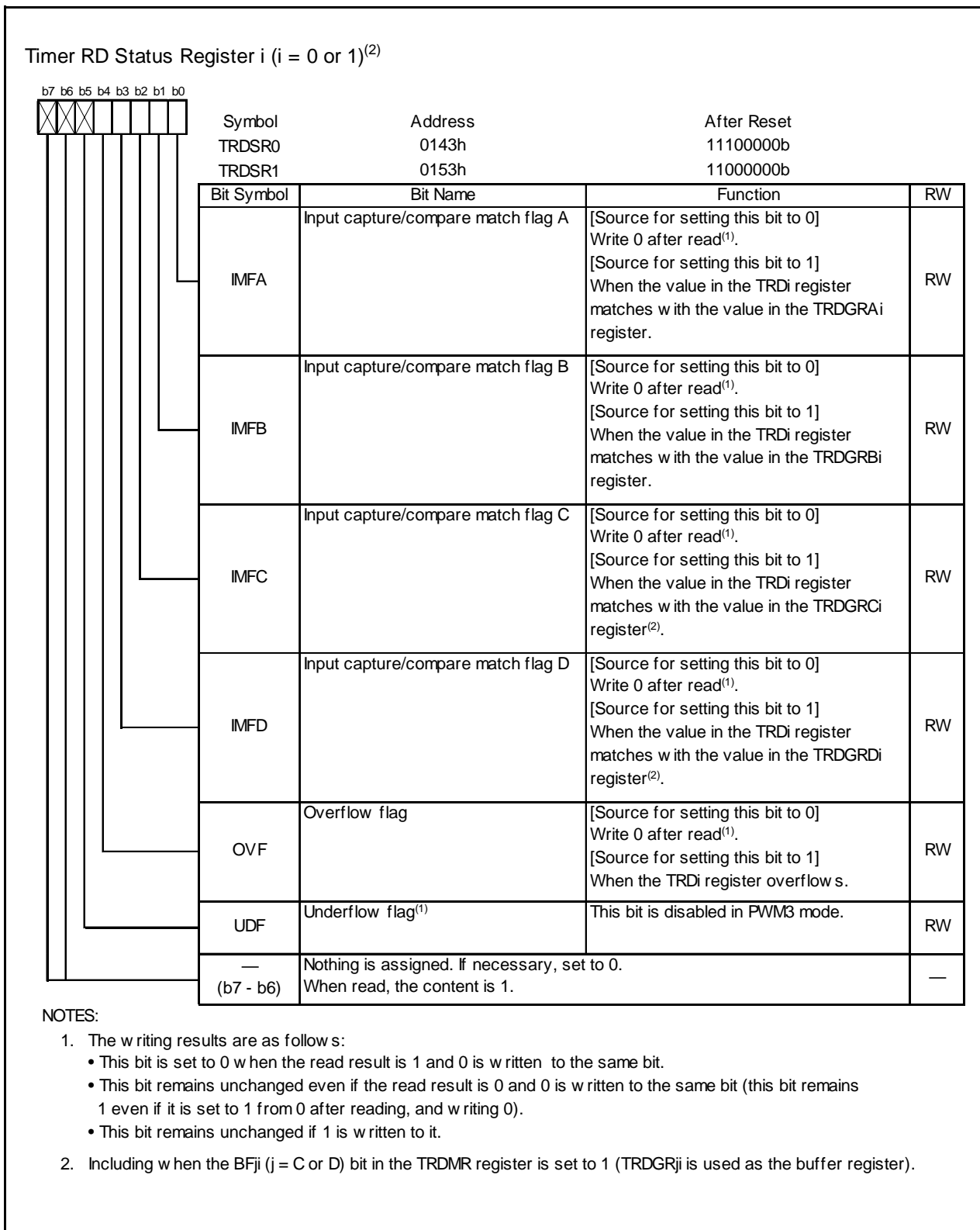
Figure 14.102 Registers TRDSR0 to TRDSR1 in PWM3 Mode
