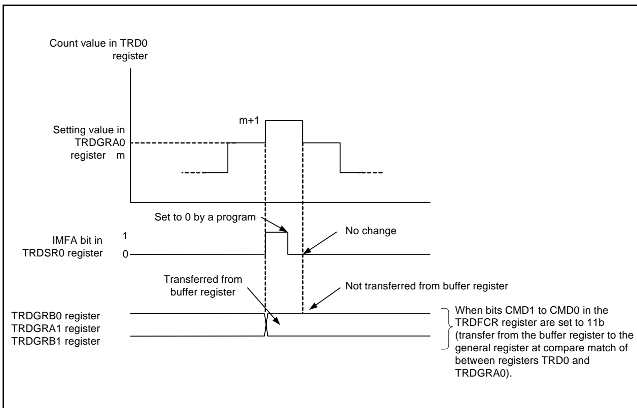
Figure 14.108 Operation at Compare Match between Registers TRD0 and TRDGRA0 in Complementary PWM Mode
