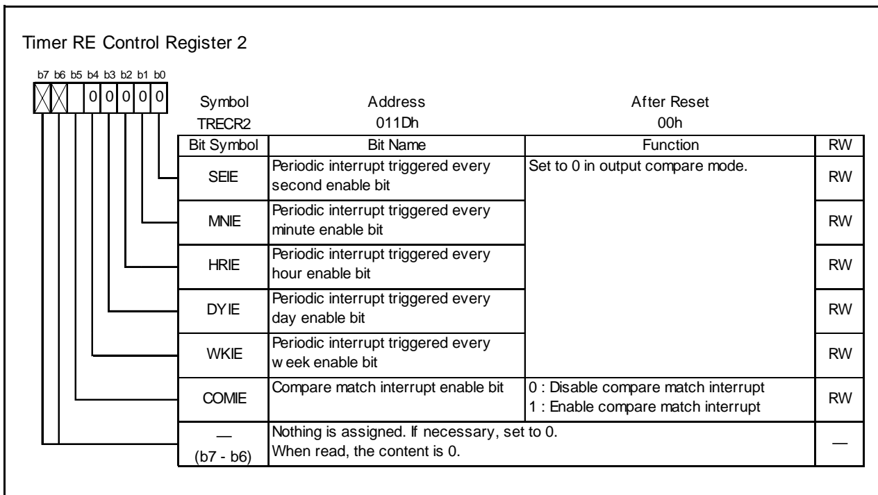
Figure 14.126 TREC2 Register in Output Compare Mode
