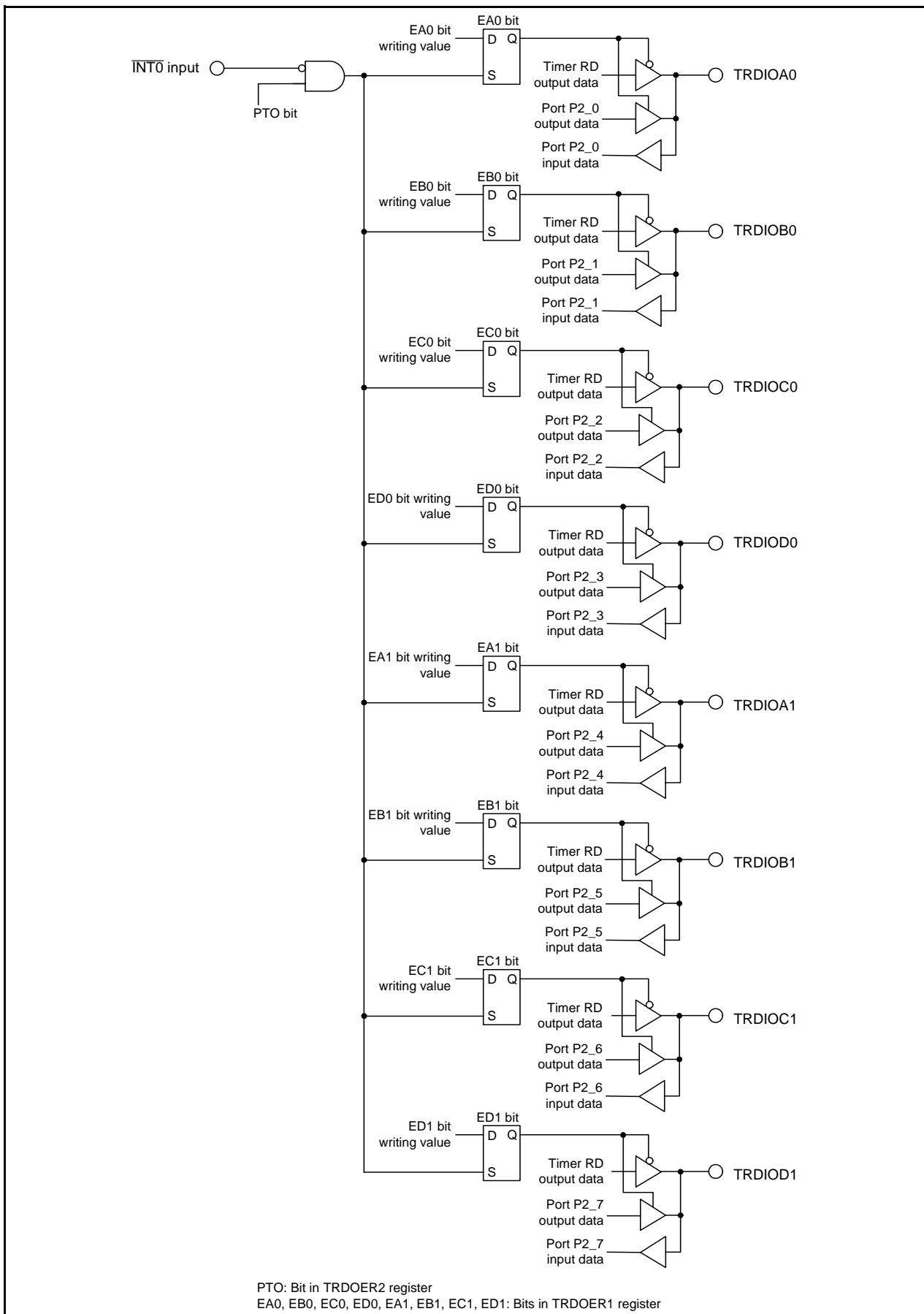
Figure 14.29 Pulse Output Forced Cutoff
