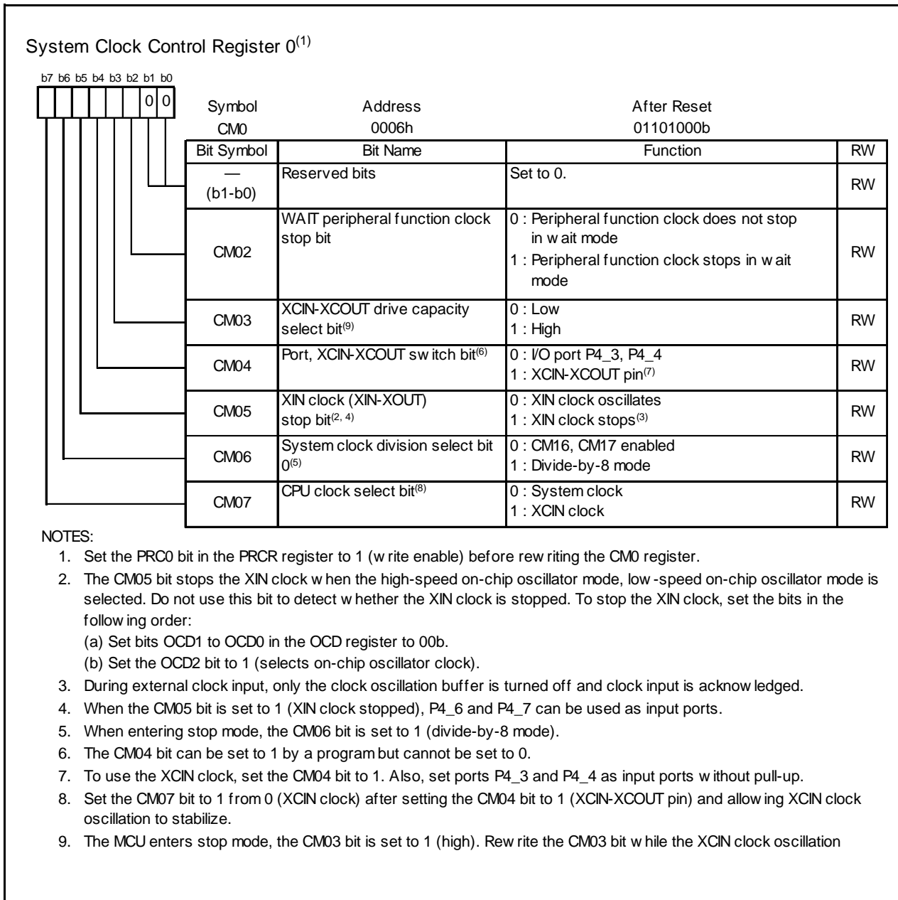
Figure 10.2 CM0 Register
