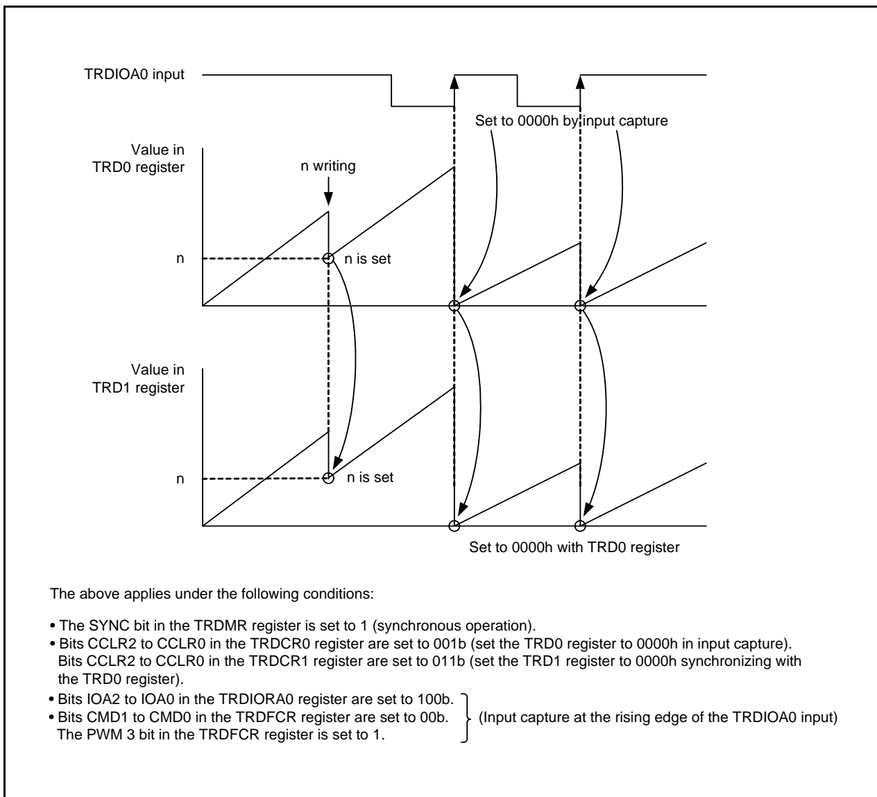
Figure 14.28 Synchronous Operation
