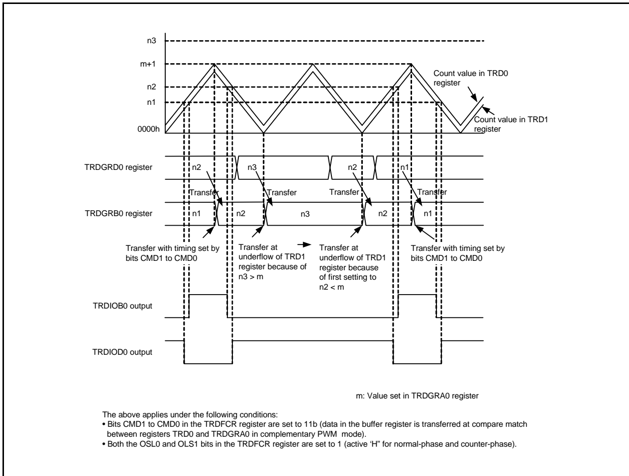
Figure 21.4 Operation when Value in Buffer Register \geq Value in TRDGRA0 Register in Complementary PWM Mode
