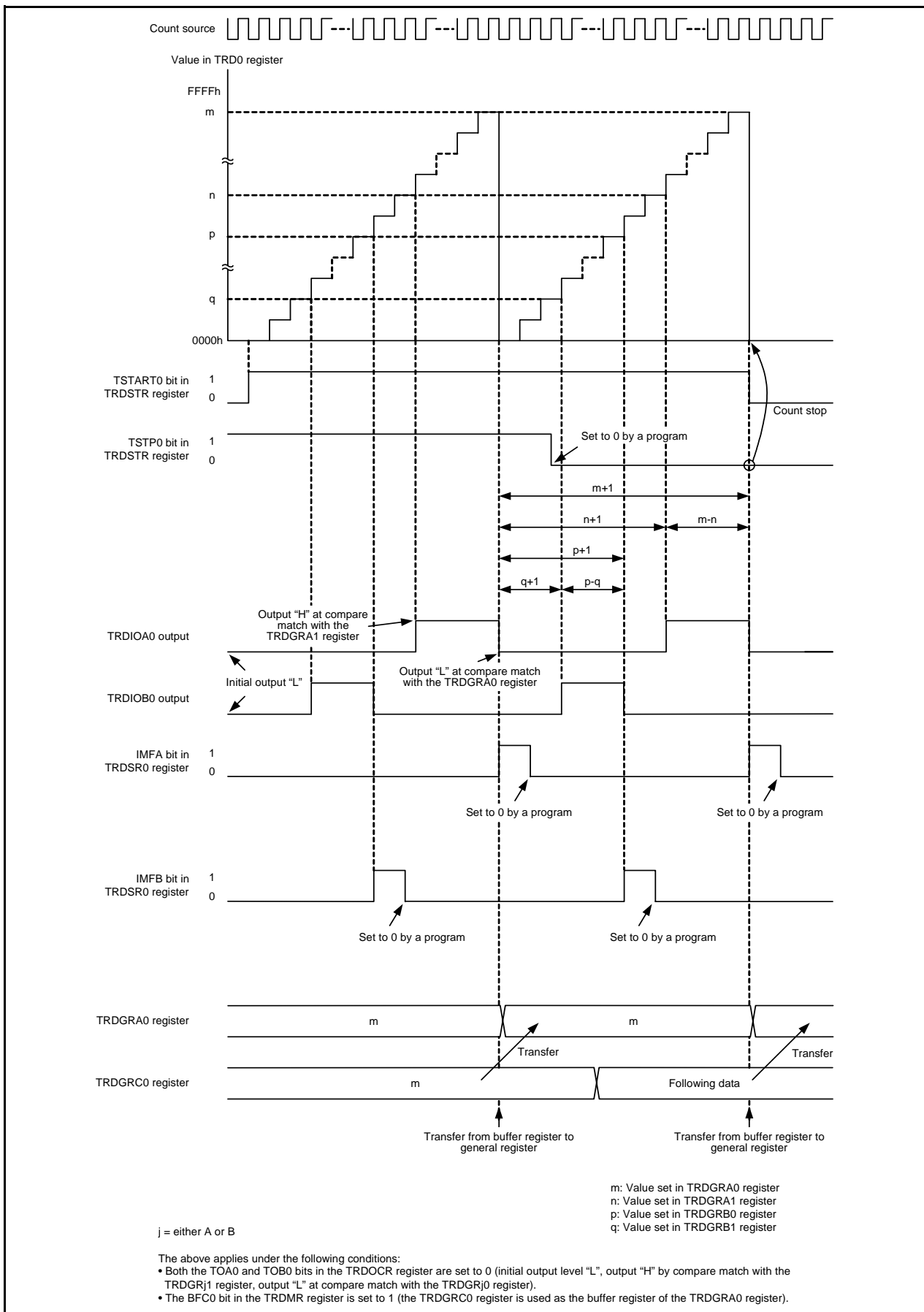
Figure 14.106 Operating Example of PWM3 Mode
