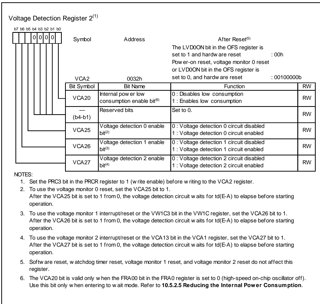
Figure 10.8 VCA2 Register
