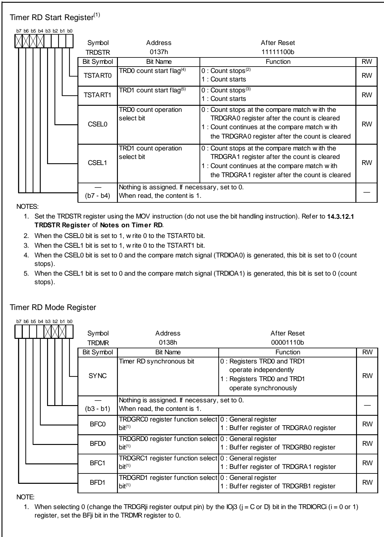
Figure 14.45 Registers TRDSTR and TRDMR in Output Compare Function
