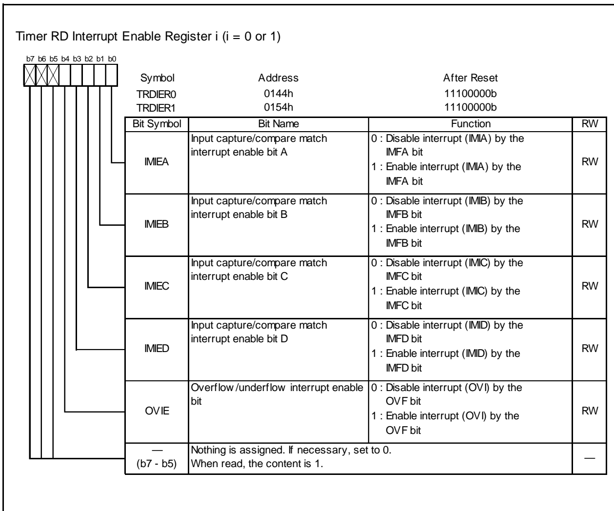
Figure 14.54 Registers TRDIER0 to TRDIER1 in Output Compare Function
