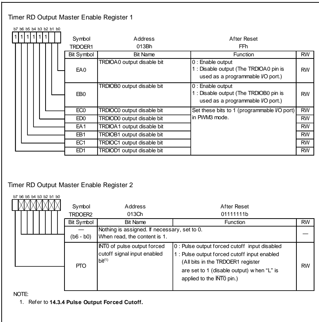
Figure 14.99 Registers TRDOER1 to TRDOER2 in PWM3 Mode
