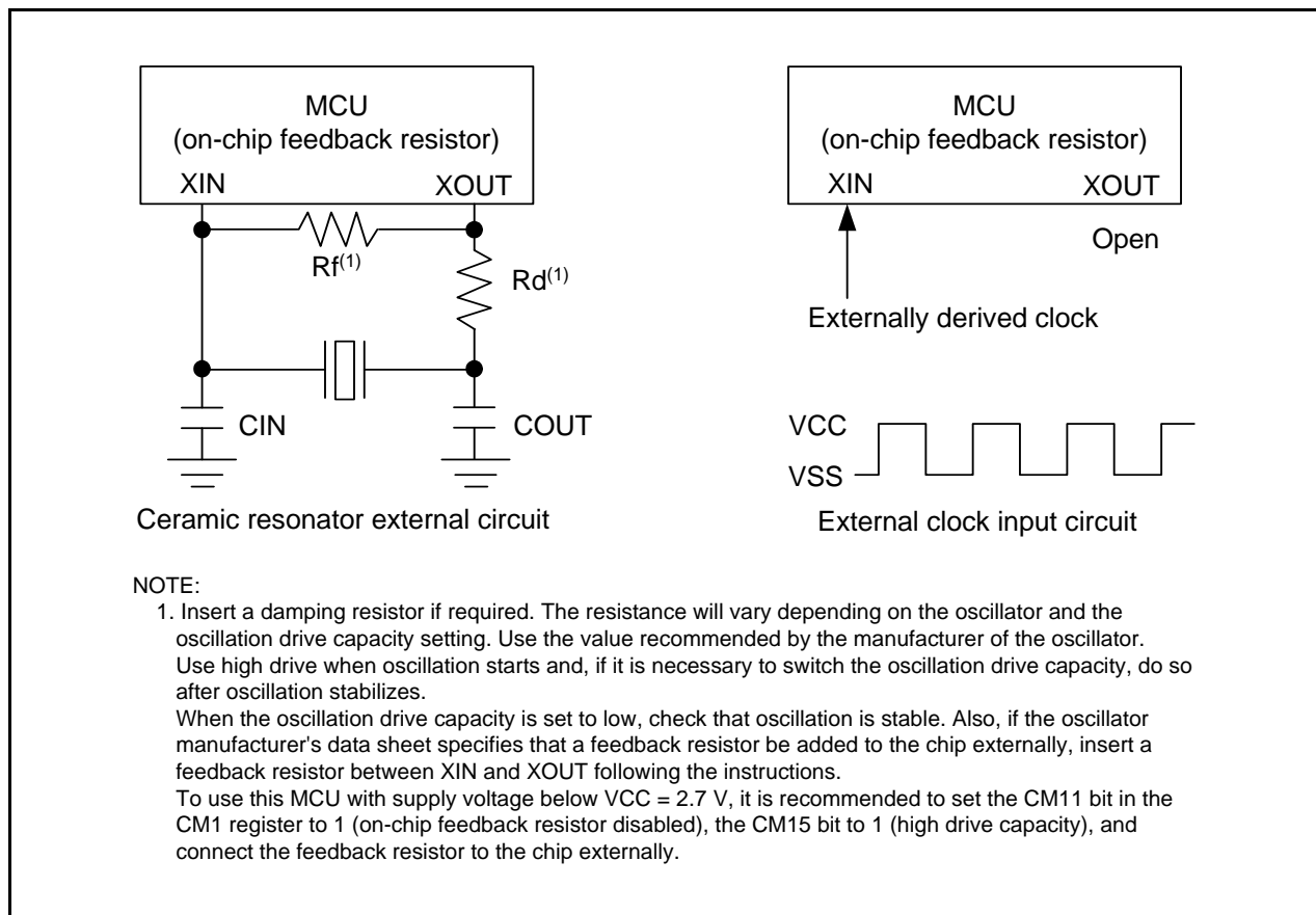
Figure 10.9 Examples of XIN Clock Connection Circuit
