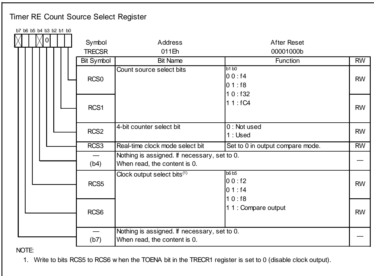
Figure 14.127 TRECSR Register in Output Compare Mode
