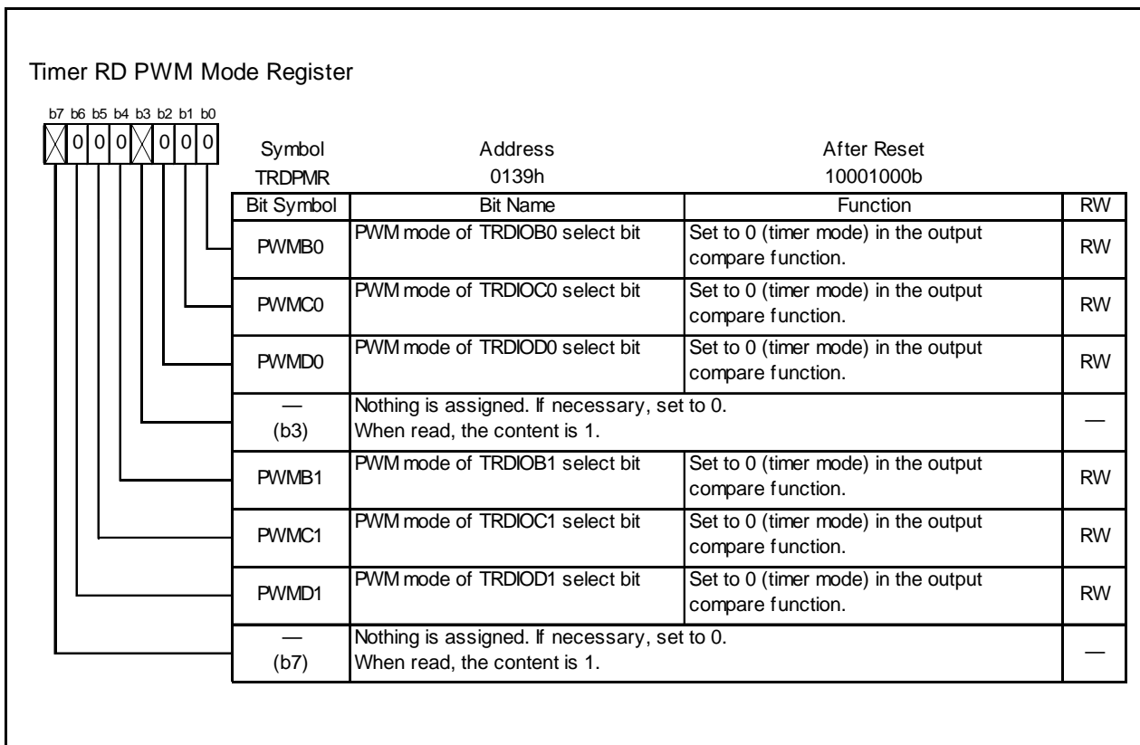
Figure 14.46 TRDPMR Register in Output Compare Function
