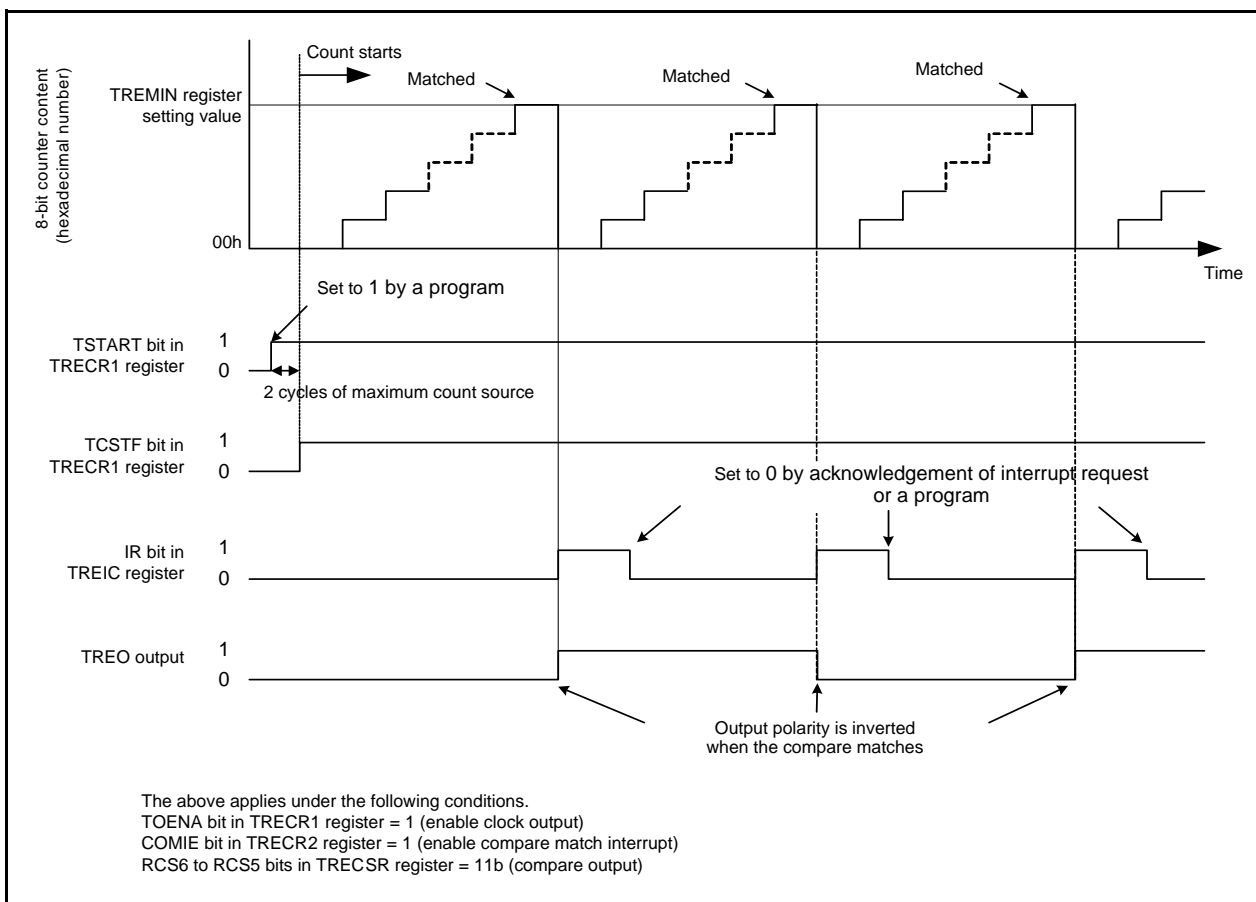
Figure 14.128 Operating Example in Output Compare Mode
