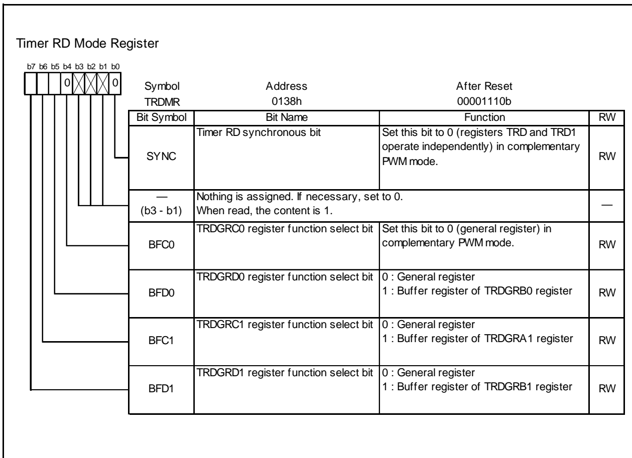
Figure 14.85 TRDMR Register in Complementary PWM Mode
