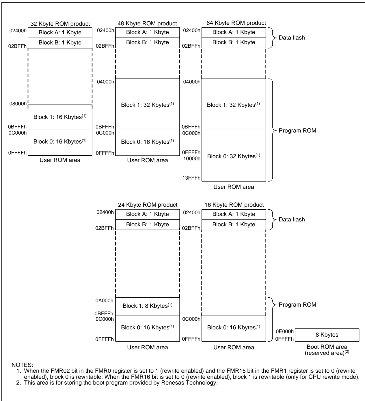
Figure 19.2 Flash Memory Block Diagram for R8C/25 Group
