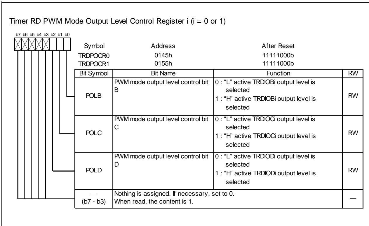
Figure 14.68 Registers TRDPOCR0 to TRDPOCR1 in PWM Mode
