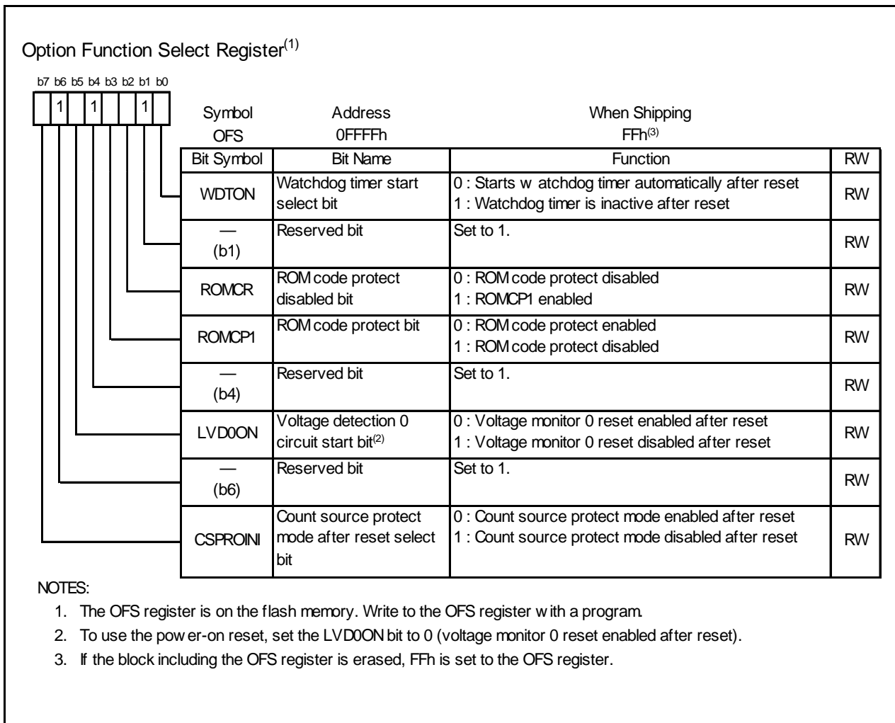
Figure 19.4 OFS Register
