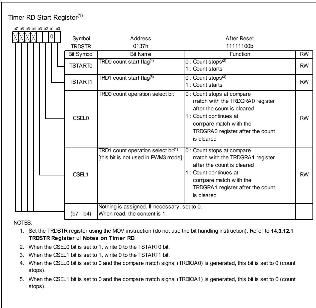
Figure 14.96 TRDSTR Register in PWM3 Mode
