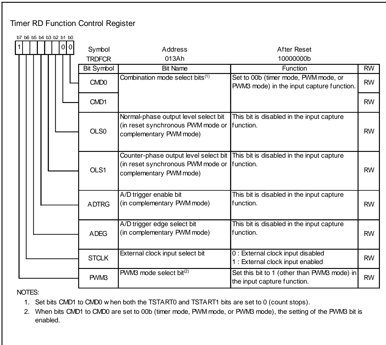
Figure 14.33 TRDFCR Register in Input Capture Function
