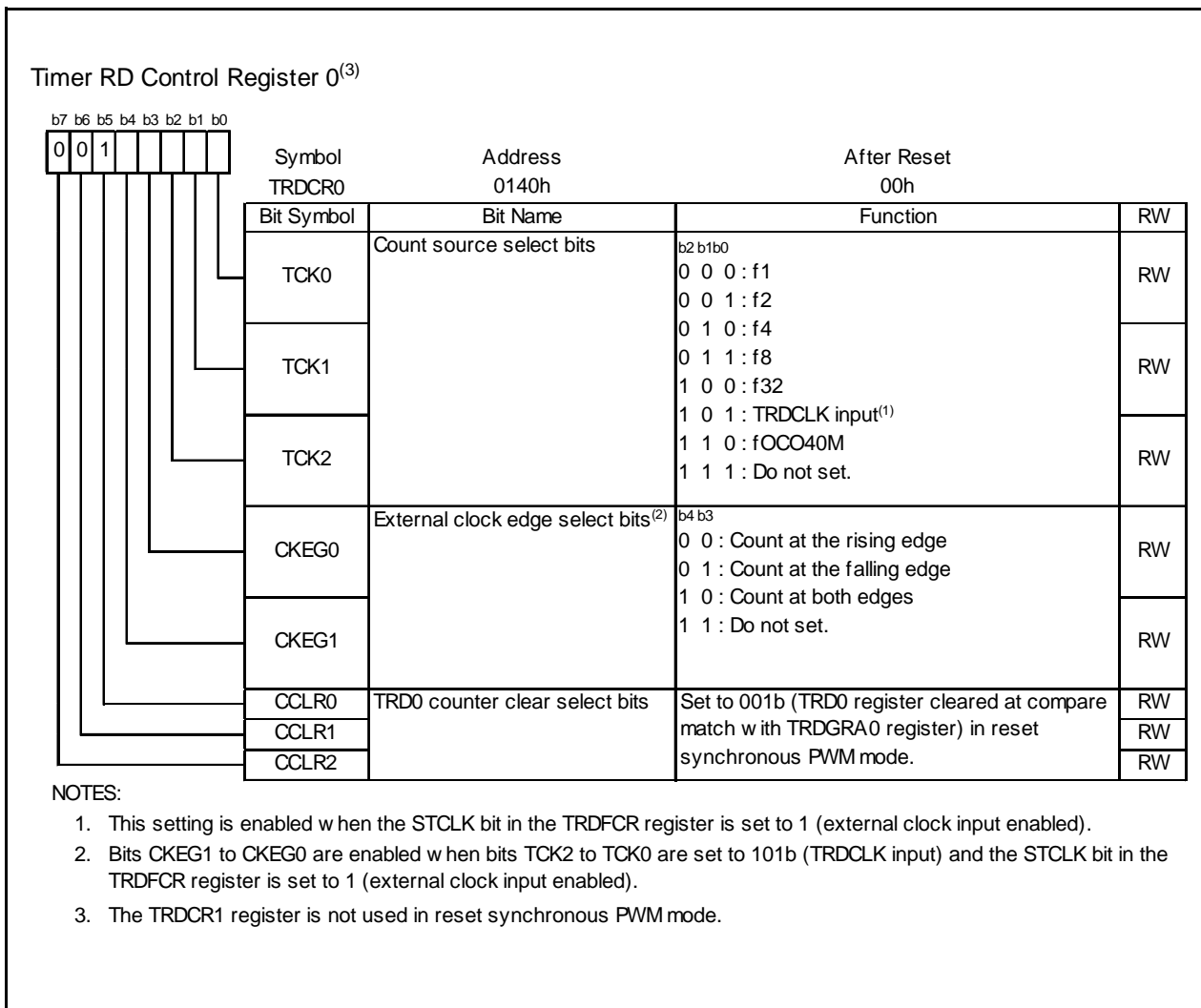
Figure 14.77 TRDCR0 Register in Reset Synchronous PWM Mode
