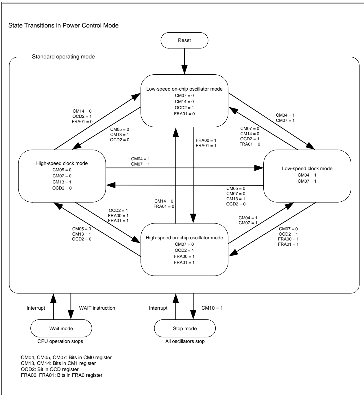
Figure 10.14 State Transitions in Power Control Mode
