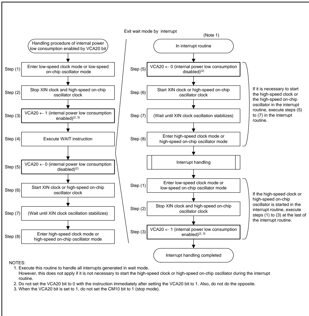
Figure 10.12 Procedure for Enabling Reduced Internal Power Consumption Using VCA20 bit
