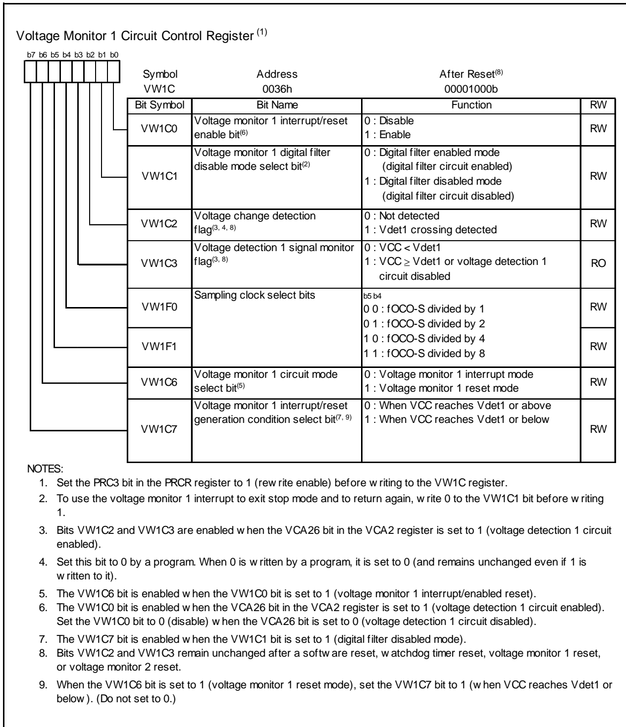
Figure 6.7 VW1C Register
