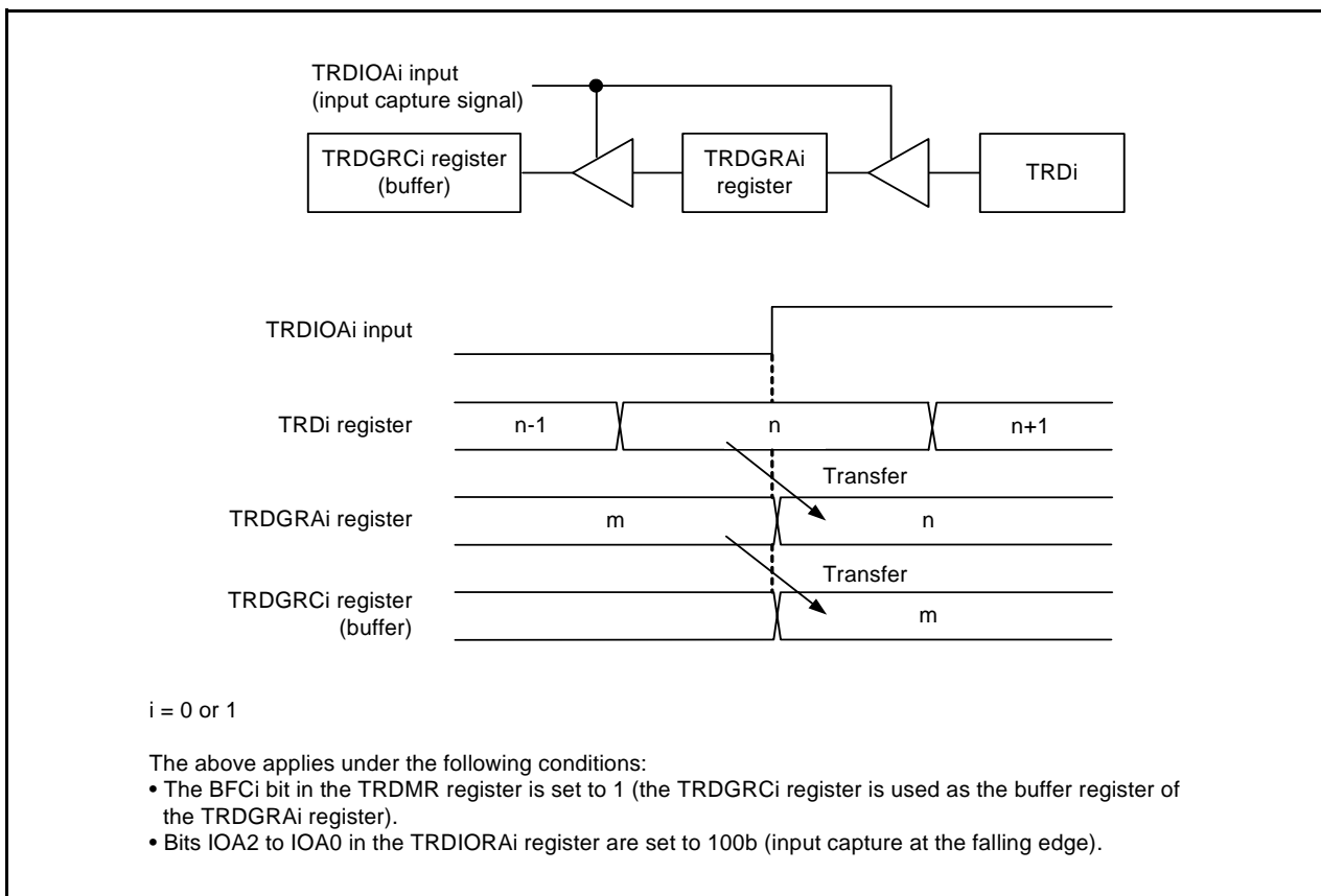
Figure 14.26 Buffer Operation in Input Capture Function
