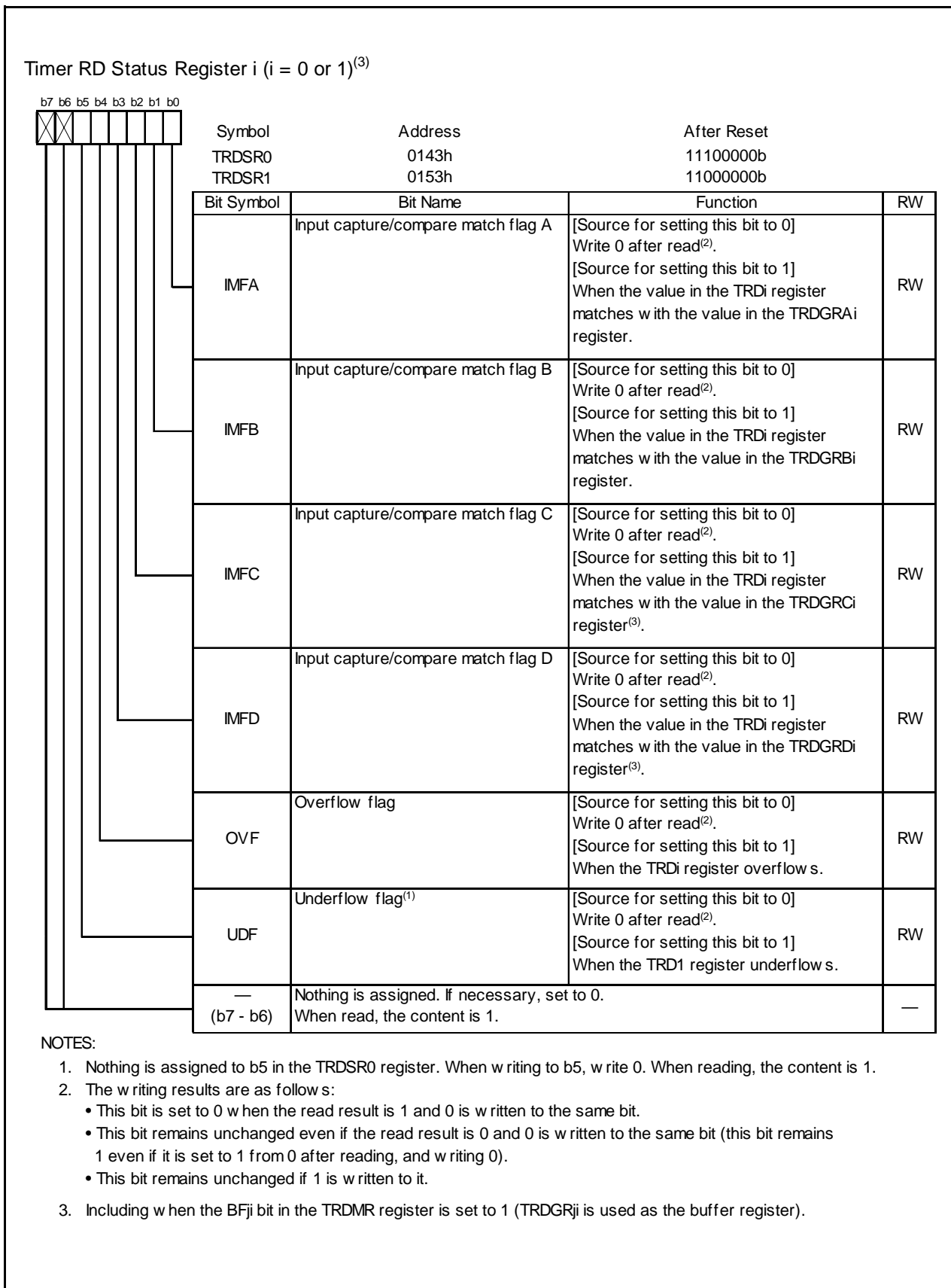
Figure 14.89 Registers TRDSR0 to TRDSR1 in Complementary PWM Mode
