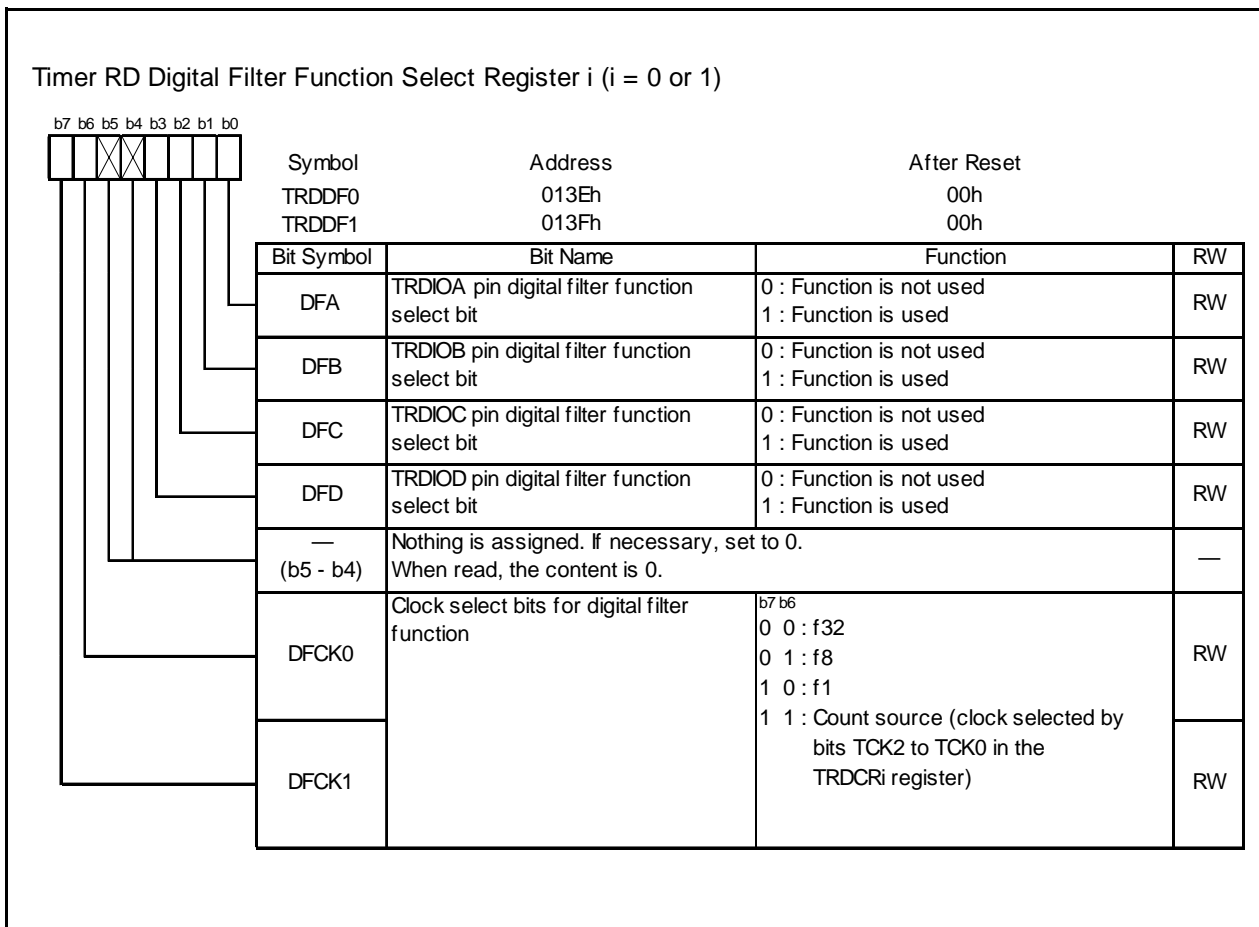
Figure 14.34 Registers TRDDF0 to TRDDF1 in Input Capture Function
