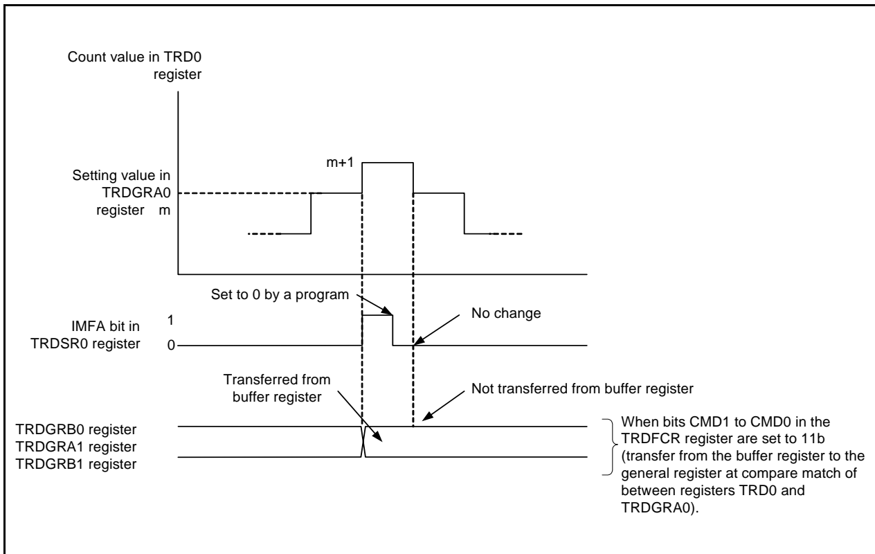
Figure 21.2 Operation at Compare Match between Registers TRD0 and TRDGRA0 in Complementary PWM Mode
