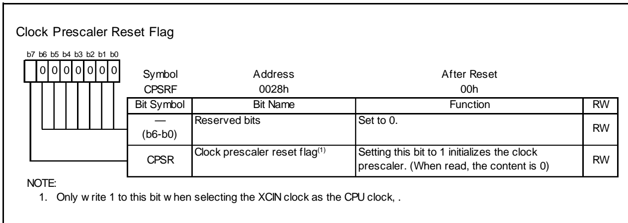
Figure 10.7 CPSRF Register
