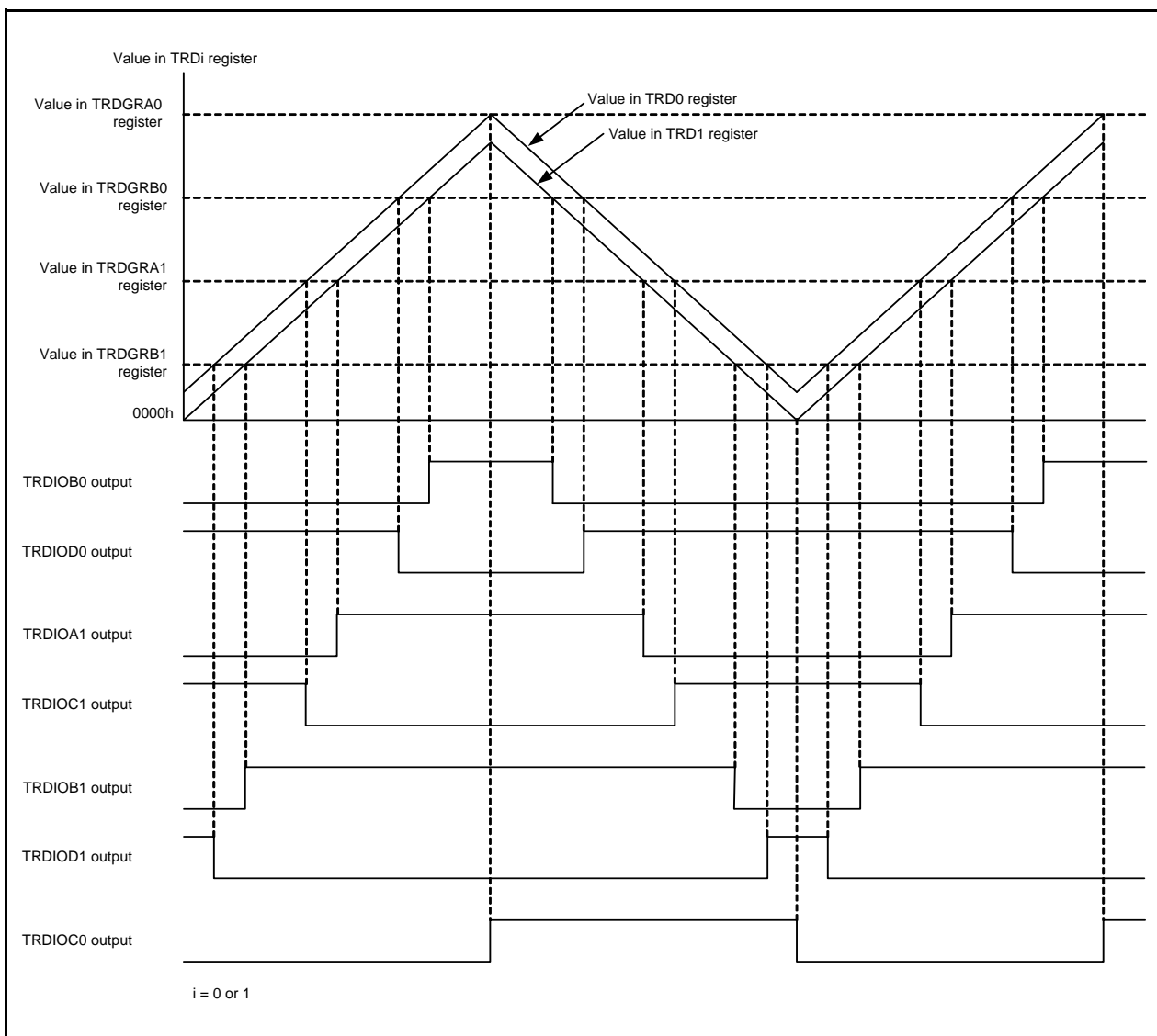
Figure 14.93 Output Model of Complementary PWM Mode
