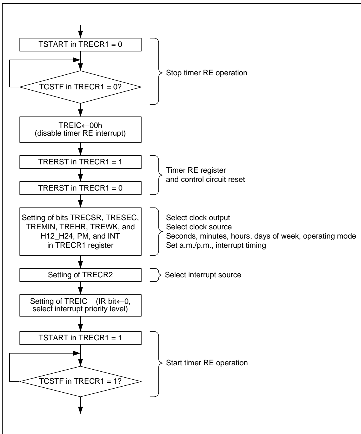
Figure 21.6 Setting Example in Real-Time Clock Mode
