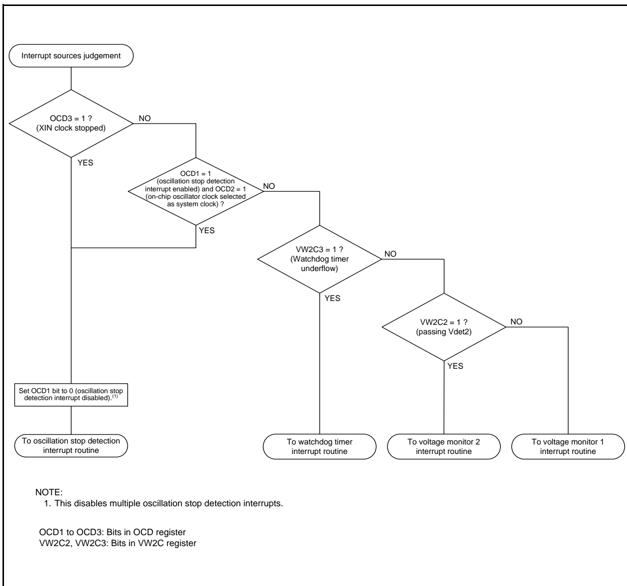
Figure 10.16 Example of Determining Interrupt Source for Oscillation Stop Detection, Watchdog Timer, Voltage Monitor 1, or Voltage Monitor 2 Interrupt
