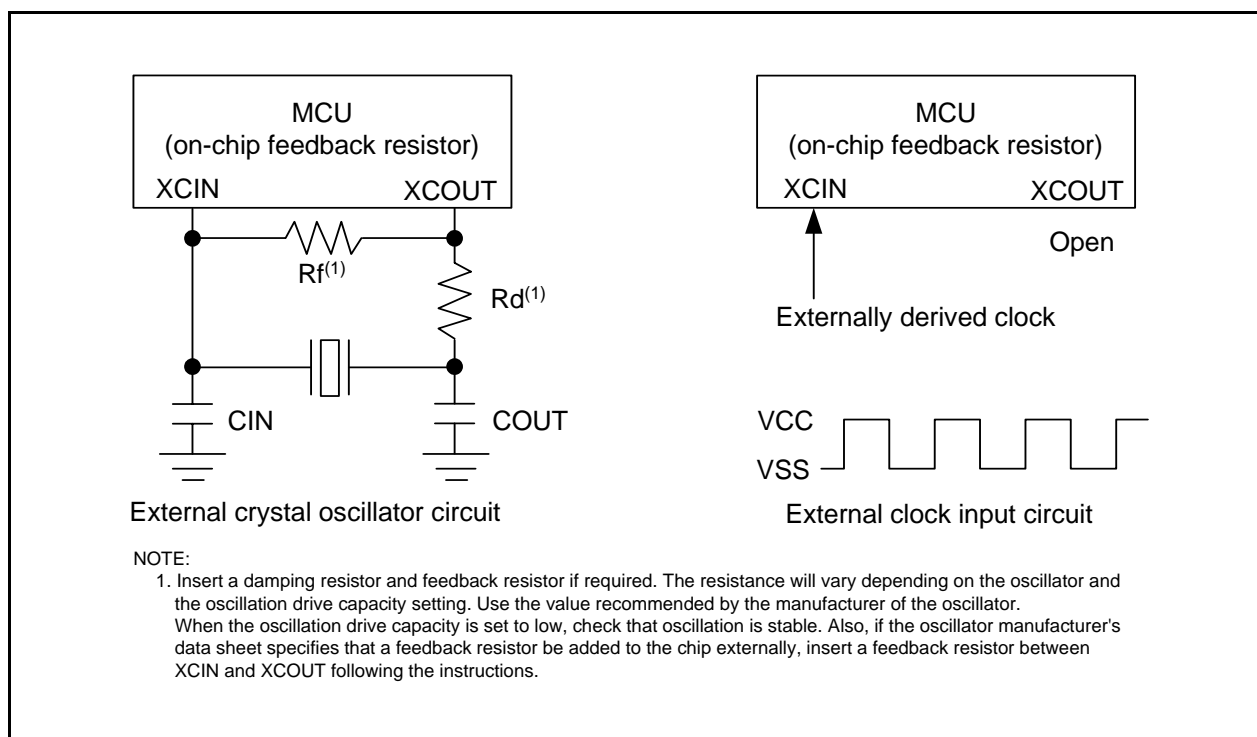
Figure 10.10 Examples of XCIN Clock Connection Circuits
