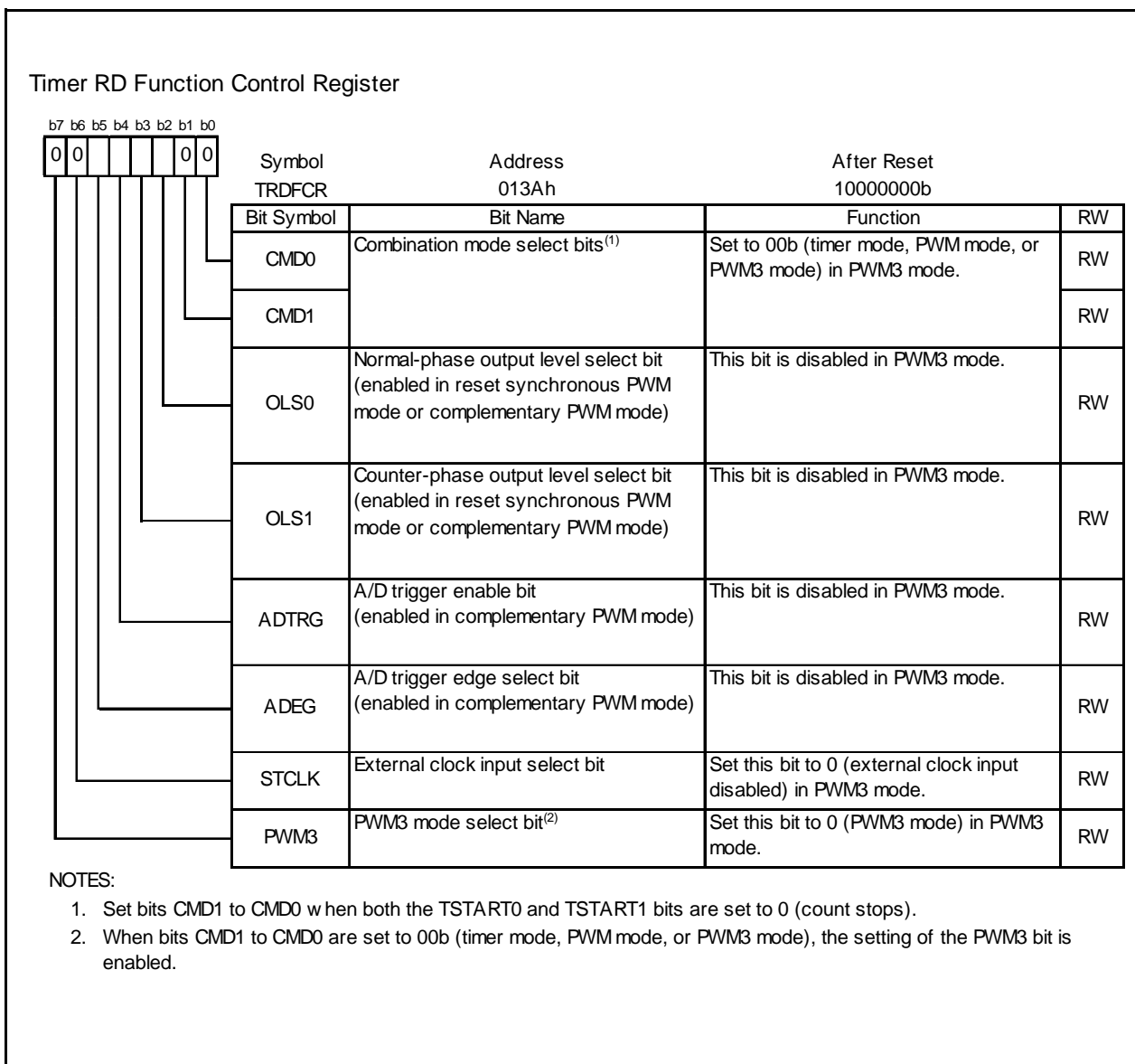
Figure 14.98 TRDFCR Register in PWM3 Mode
