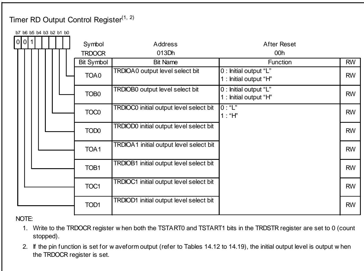
Figure 14.49 TRDOCR Register in Output Compare Function
