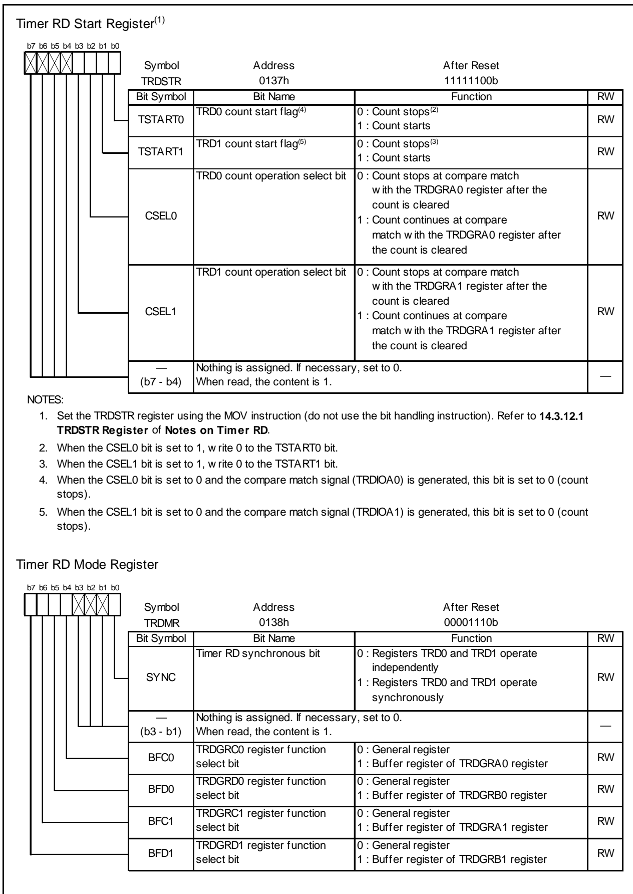
Figure 14.61 Registers TRDSTR and TRDMR in PWM Mode
