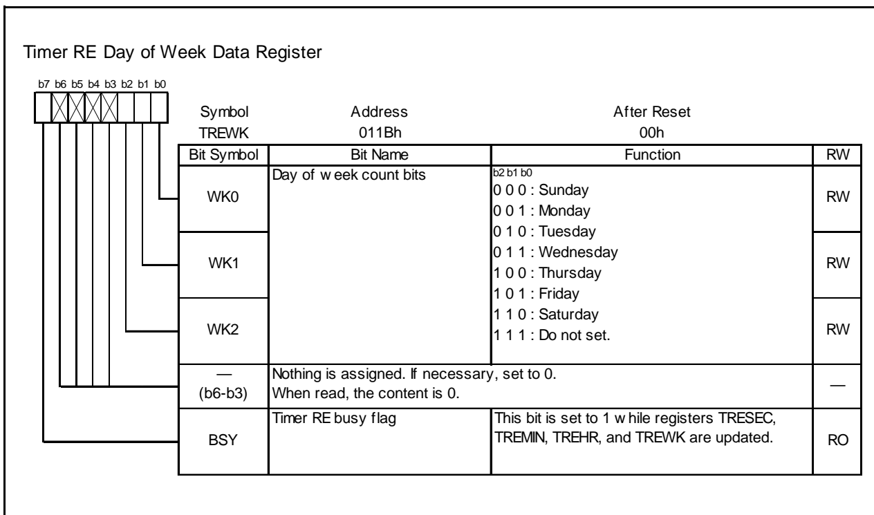
Figure 14.116 TREWK Register in Real-Time Clock Mode
