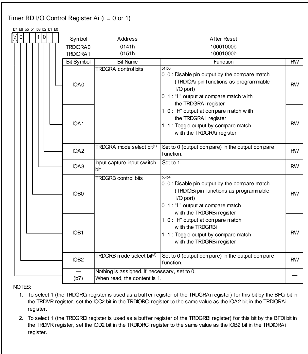
Figure 14.51 Registers TRDIORA0 to TRDIORA1 in Output Compare Function
