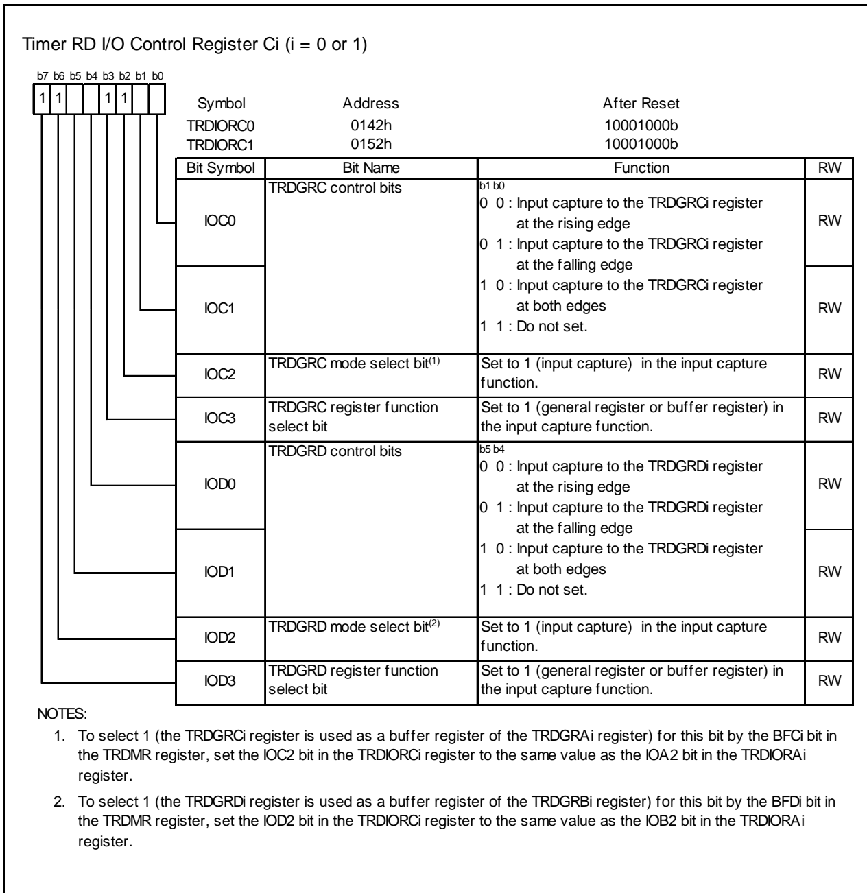
Figure 14.37 Registers TRDIORC0 to TRDIORC1 in Input Capture Function
