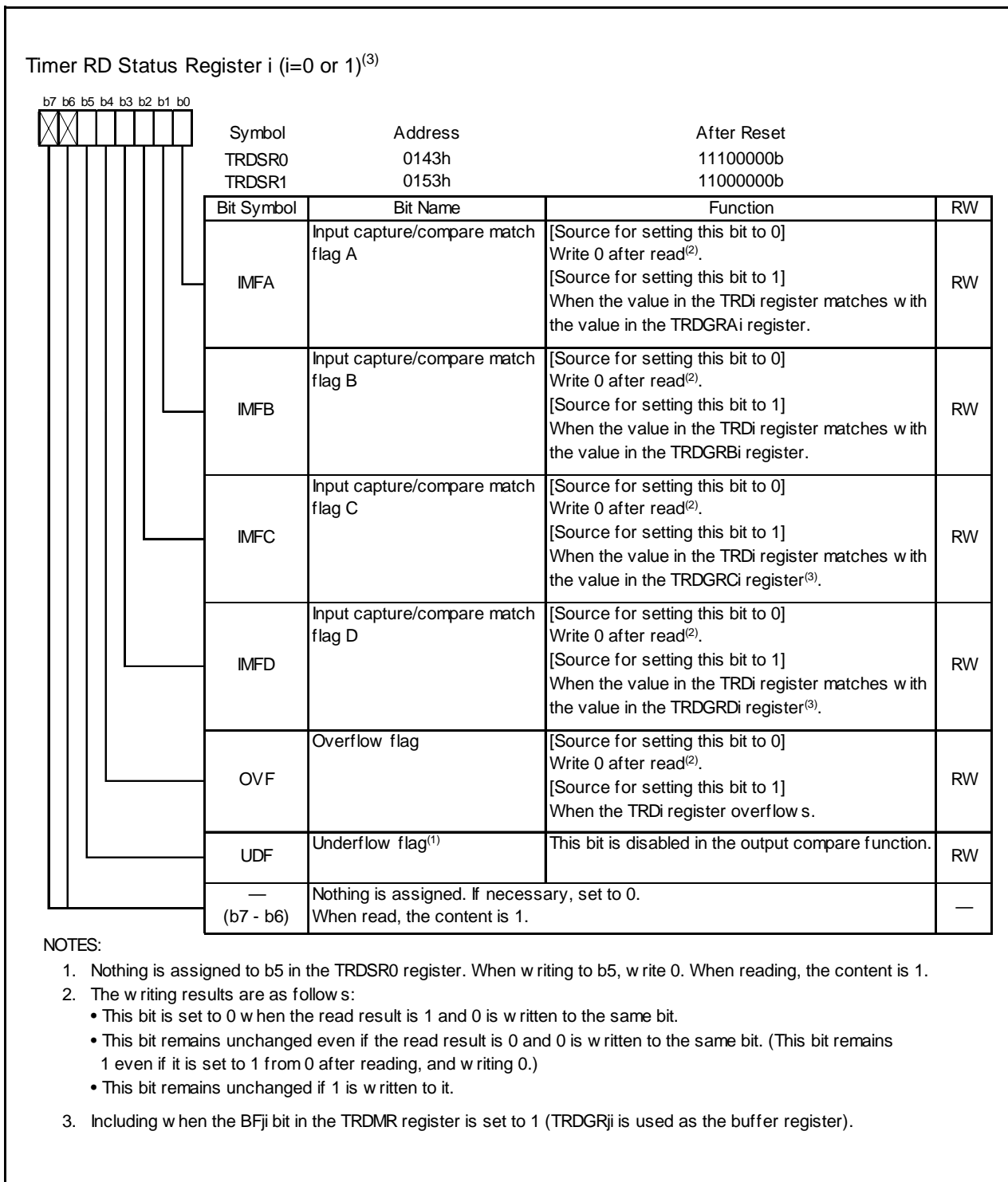
Figure 14.53 Registers TRDSR0 to TRDSR1 in Output Compare Function
