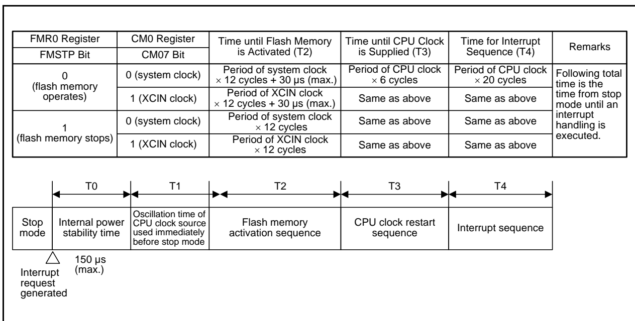
Figure 10.13 Time from Stop Mode to Interrupt Routine Execution
