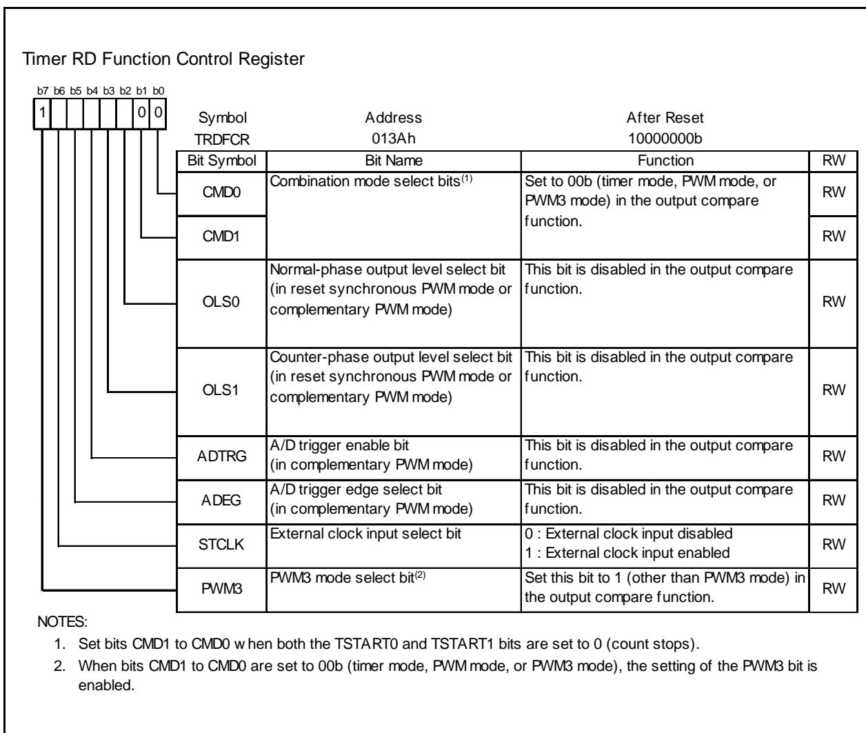
Figure 14.47 TRDFCR Register in Output Compare Function
