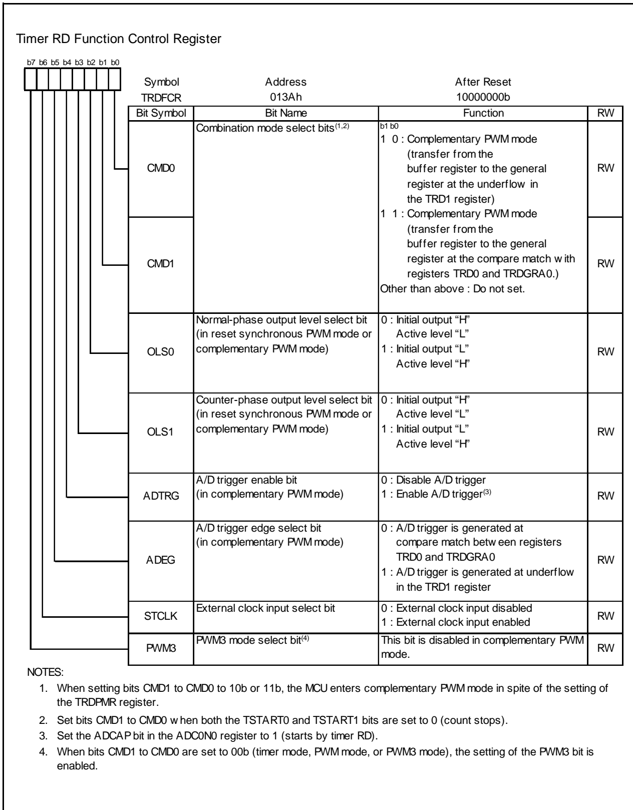
Figure 14.86 TRDFCR Register in Complementary PWM Mode
