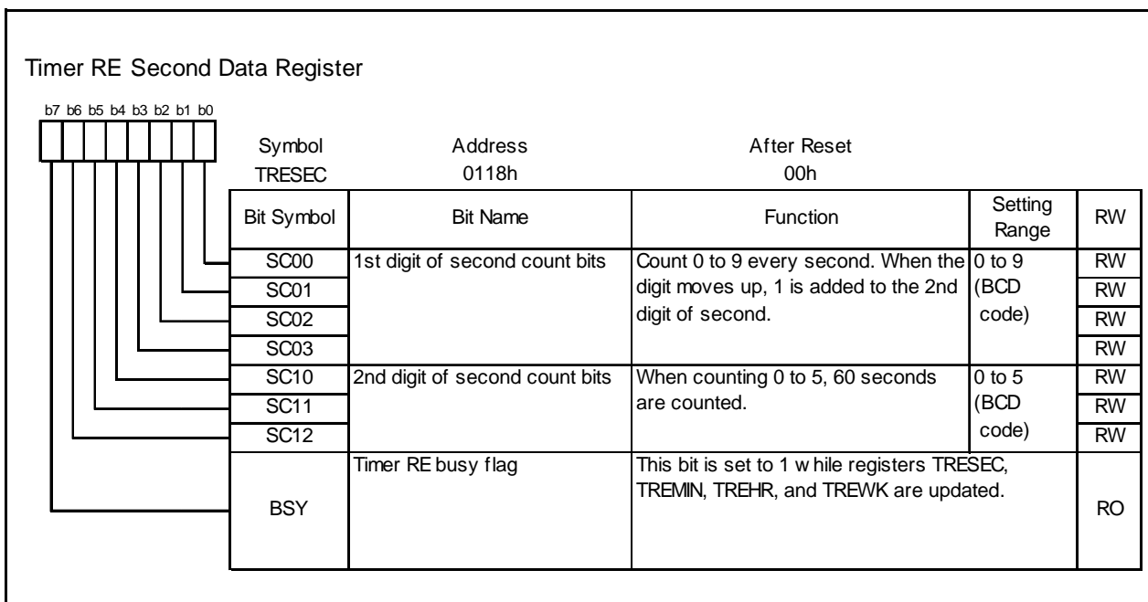
Figure 14.113 TRESEC Register in Real-Time Clock Mode
