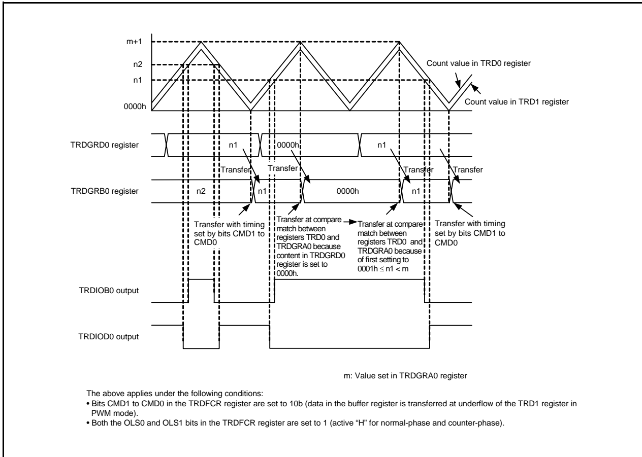
Figure 21.5 Operation when Value in Buffer Register Is Set to 0000h in Complementary PWM Mode
