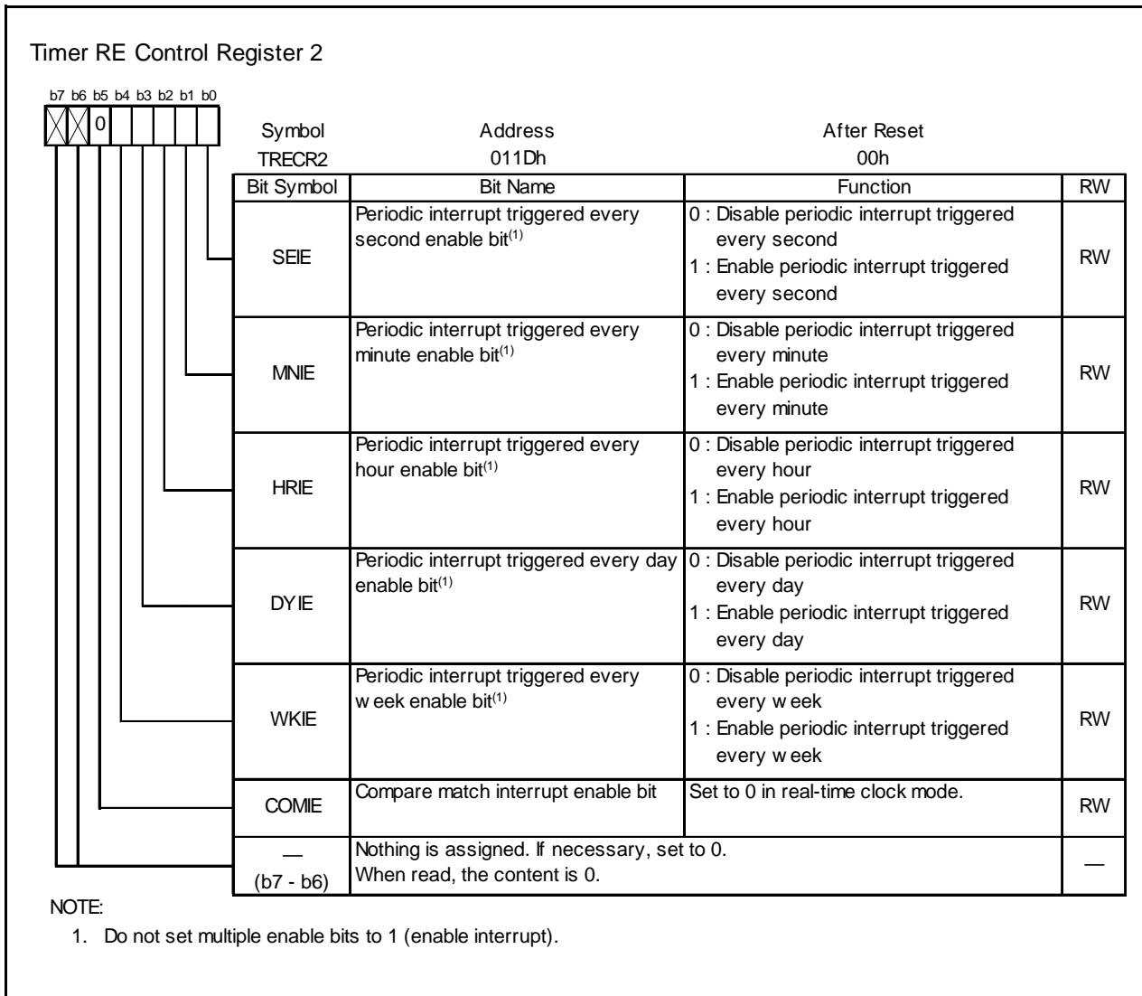
Figure 14.119 TRECR2 Register in Real-Time Clock Mode
