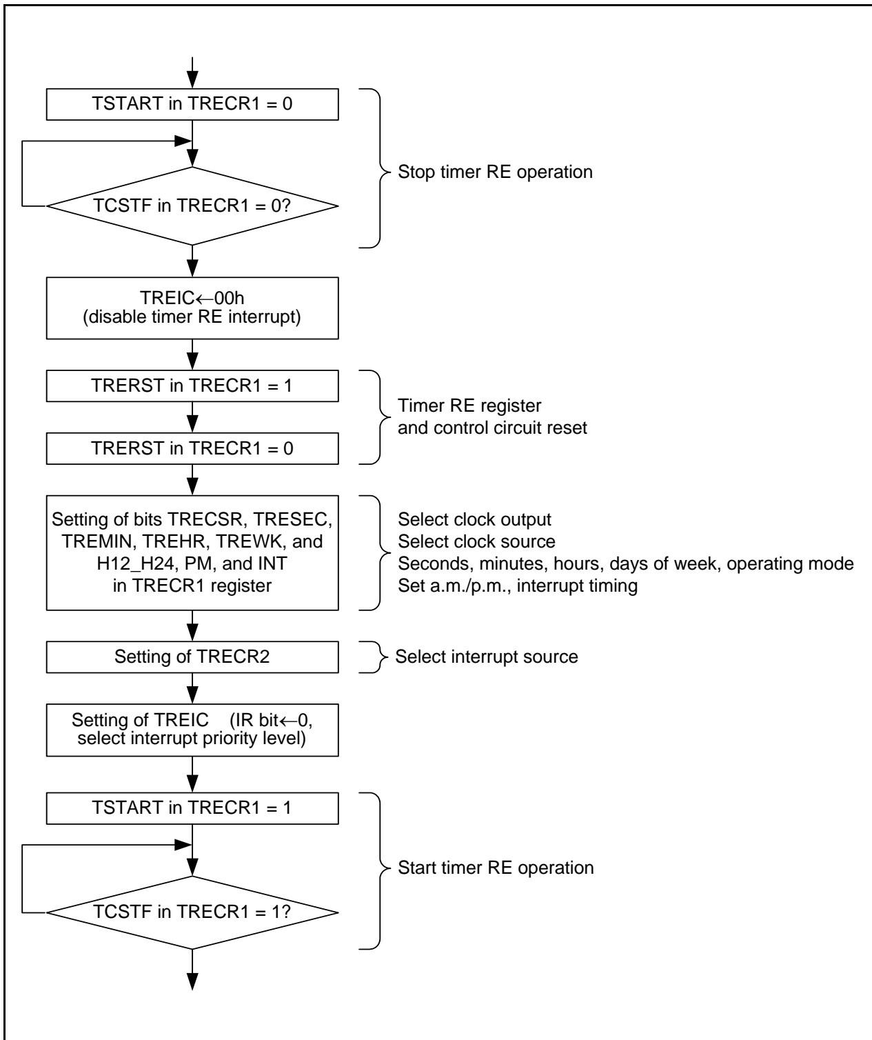
Figure 14.129 Setting Example in Real-Time Clock Mode
