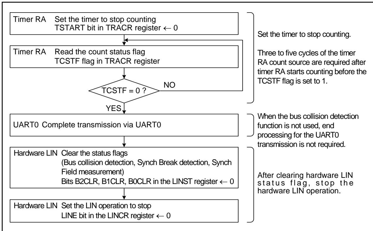
Figure 17.12 Example of Hardware LIN Communication Completion Flowchart
