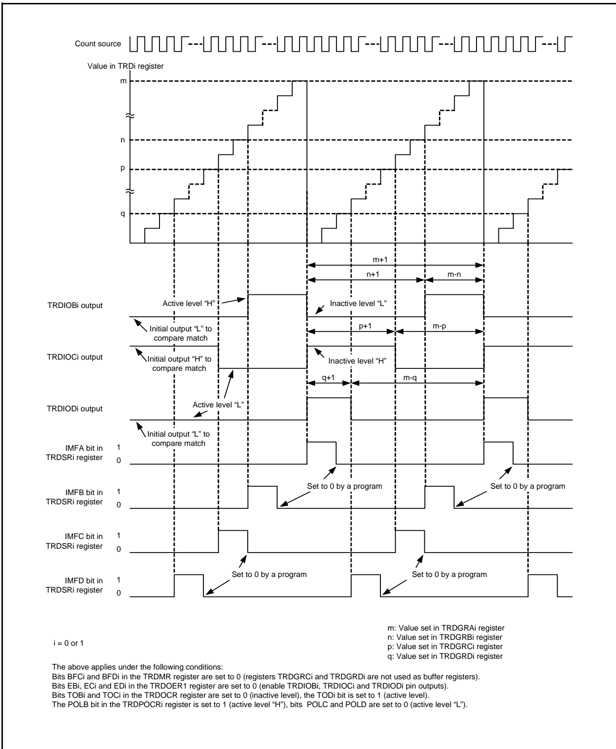
Figure 14.71 Operating Example of PWM Mode
