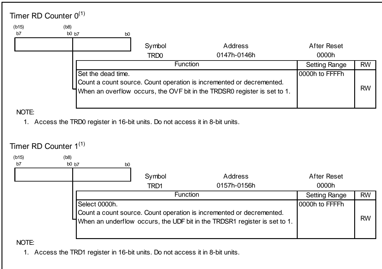
Figure 14.91 Registers TRD0 to TRD1 in Complementary PWM Mode
