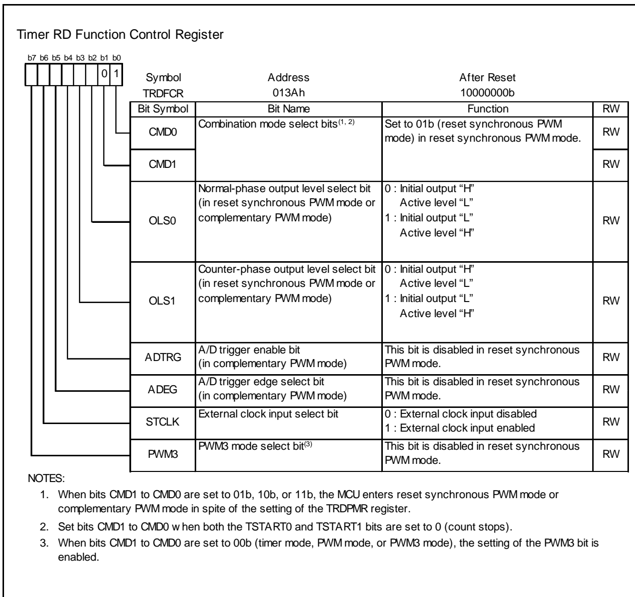
Figure 14.75 TRDFCR Register in Reset Synchronous PWM Mode
