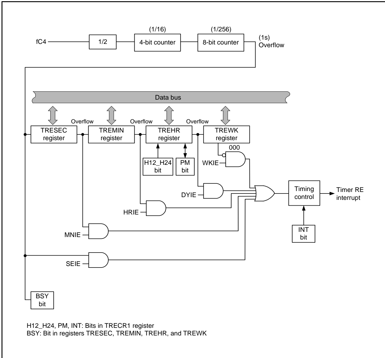
Figure 14.112 Block Diagram of Real-Time Clock Mode
