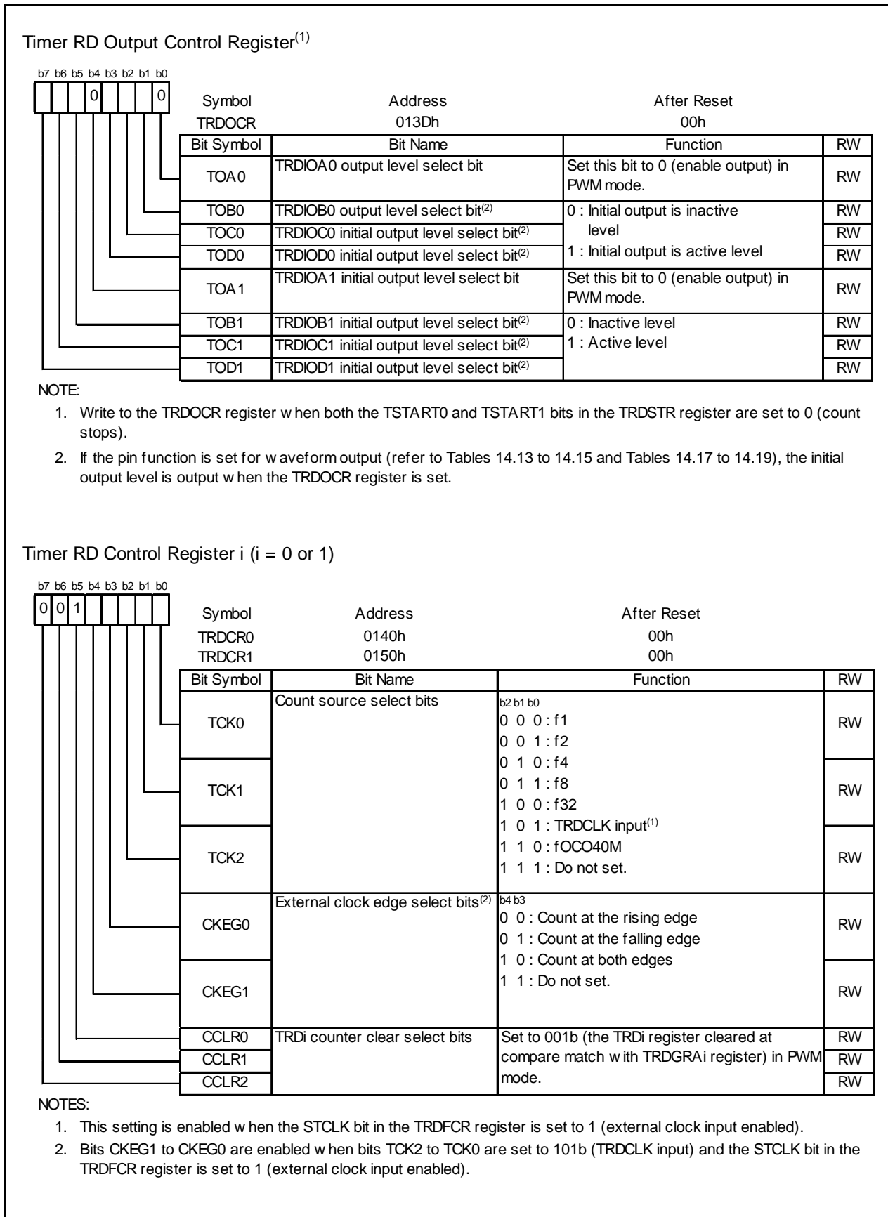
Figure 14.65 Registers TRDOCR and TRDCR0 to TRDCR1 in PWM Mode
