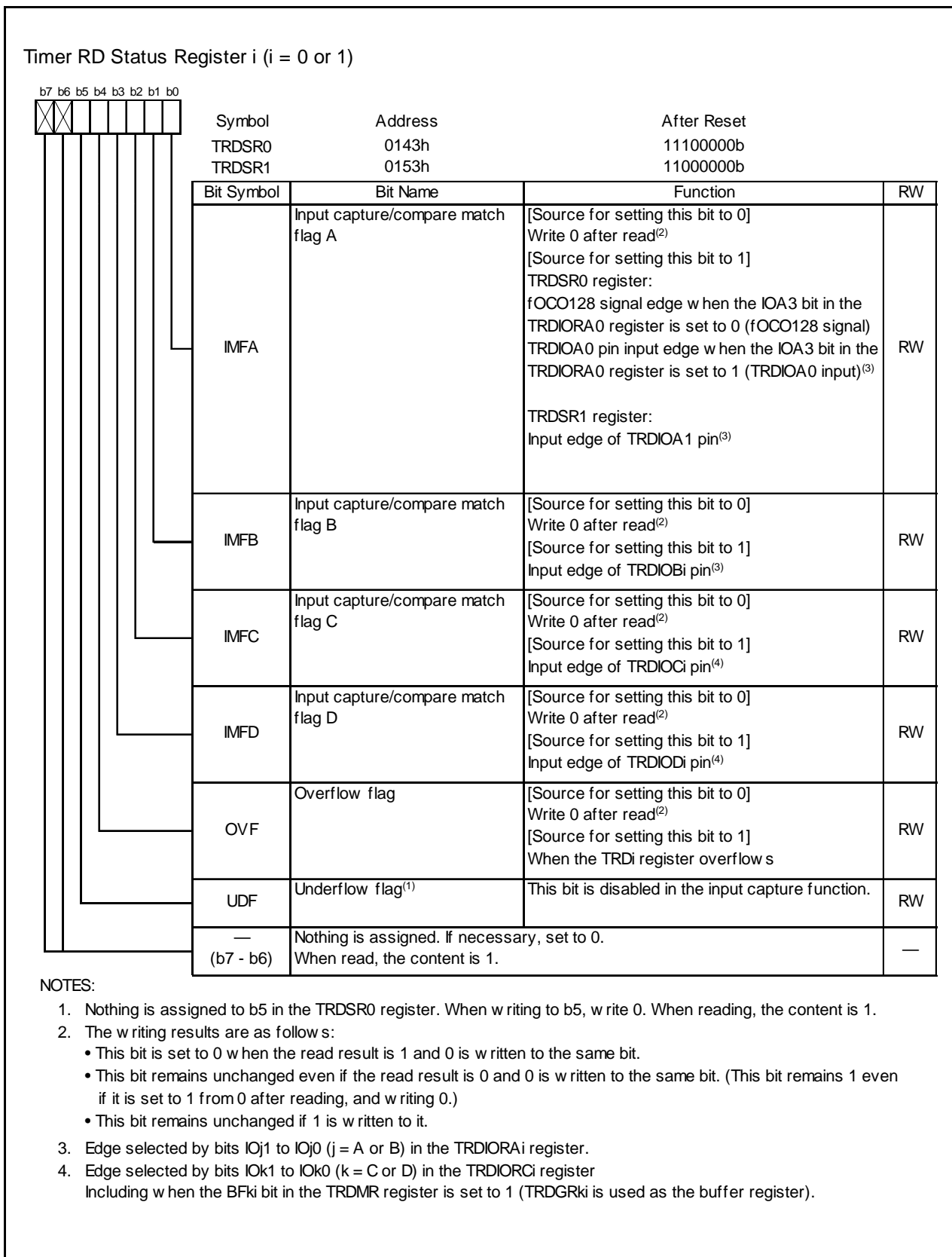
Figure 14.38 Registers TRDSR0 to TRDSR1 in Input Capture Function
