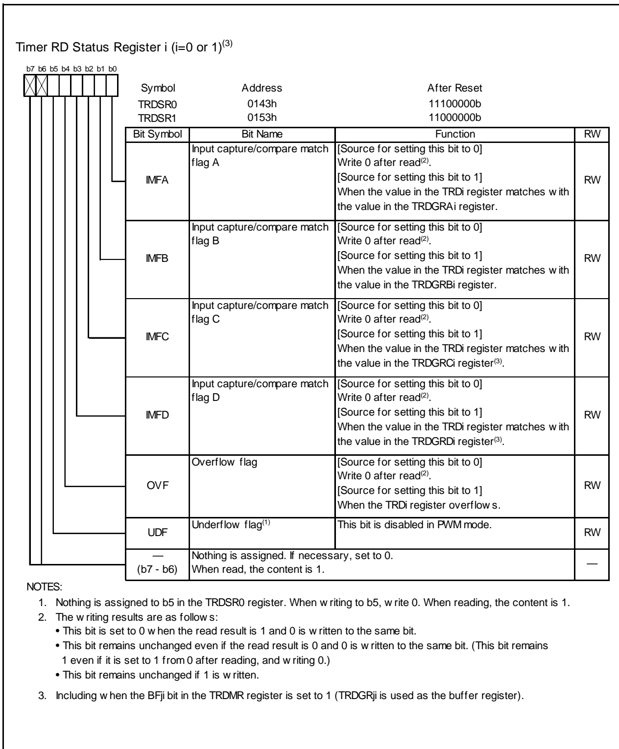
Figure 14.66 Registers TRDSR0 to TRDSR1 in PWM Mode
