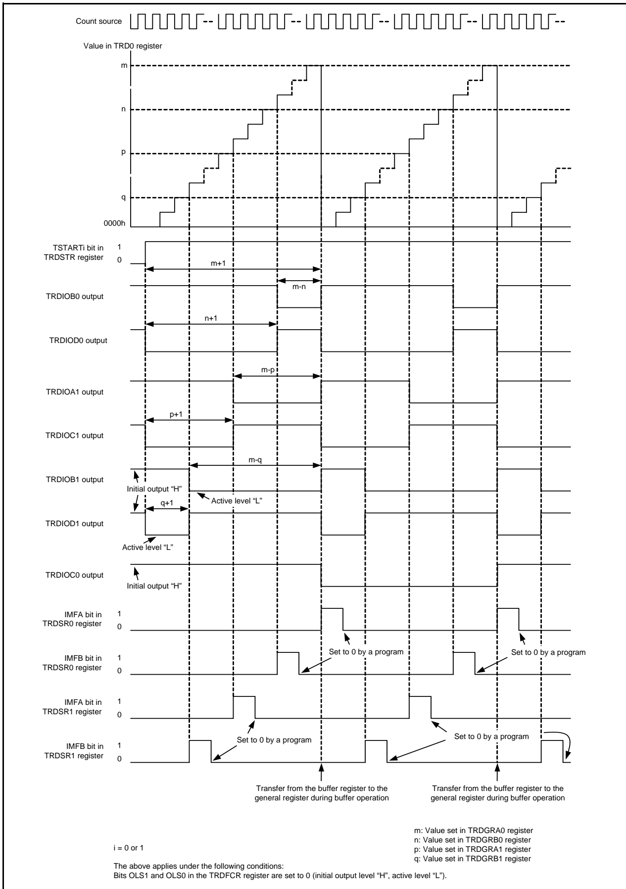
Figure 14.82 Operating Example of Reset Synchronous PWM Mode
