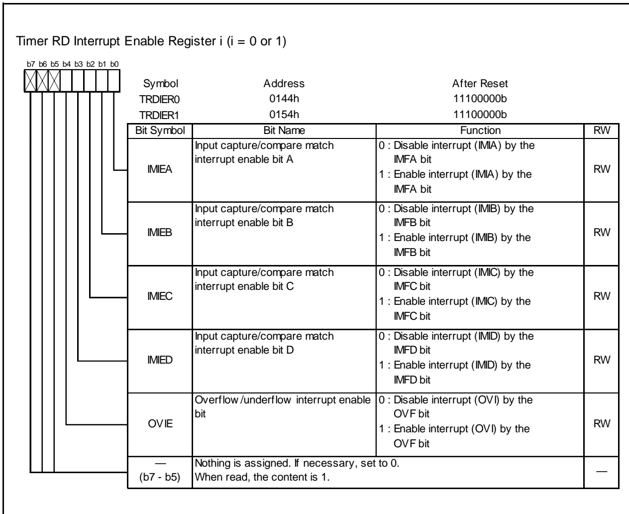
Figure 14.103 Registers TRDIER0 to TRDIER1 in PWM3 Mode
