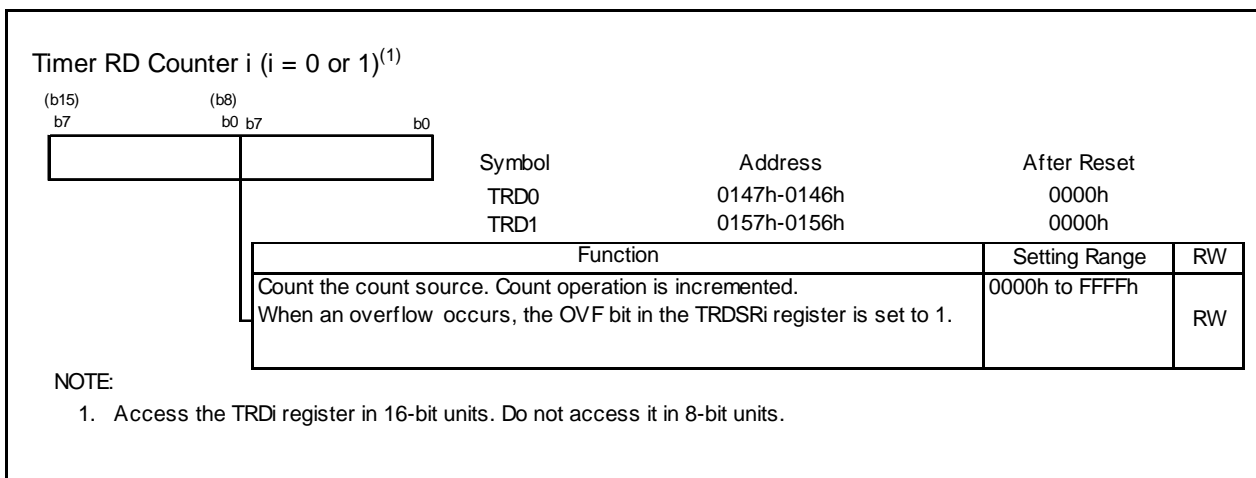
Figure 14.40 Registers TRD0 to TRD1 in Input Capture Function
