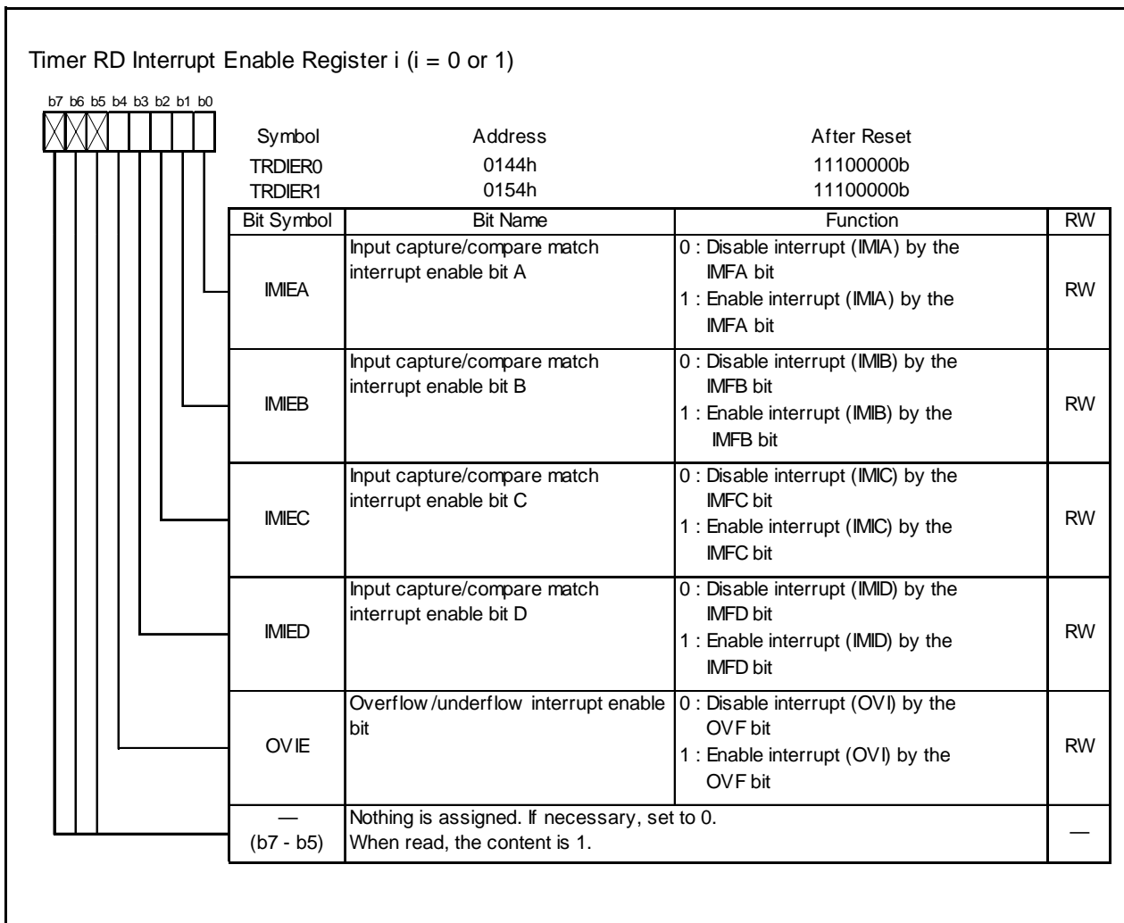
Figure 14.67 Registers TRDIER0 to TRDIER1 in PWM Mode
