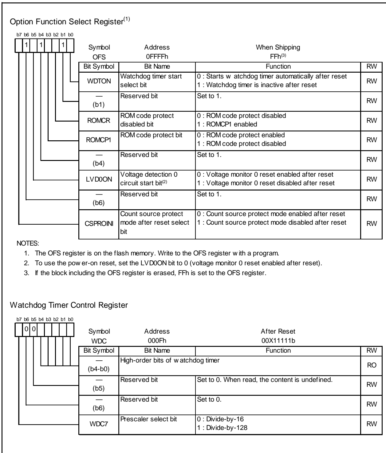
Figure 13.2 Registers OFS and WDC
