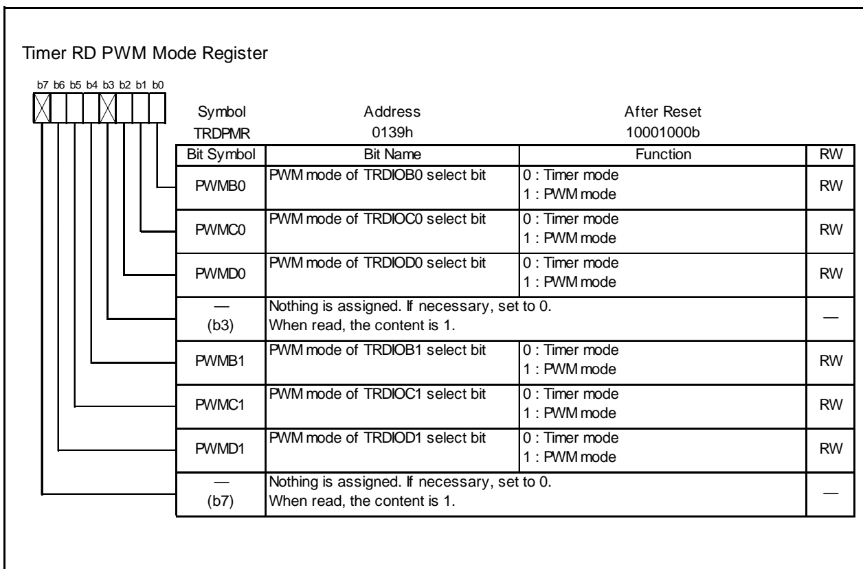
Figure 14.62 TRDPMR Register in PWM Mode
