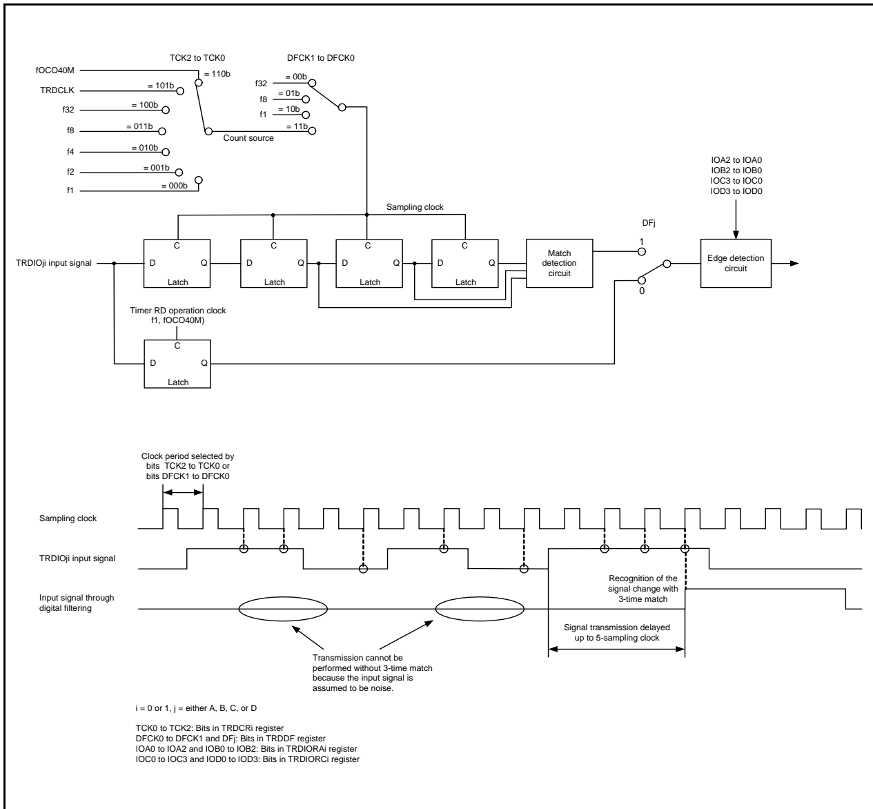
Figure 14.43 Block Diagram of Digital Filter
