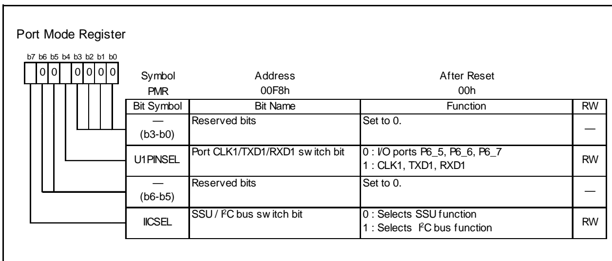
Figure 7.12 PMR Register
