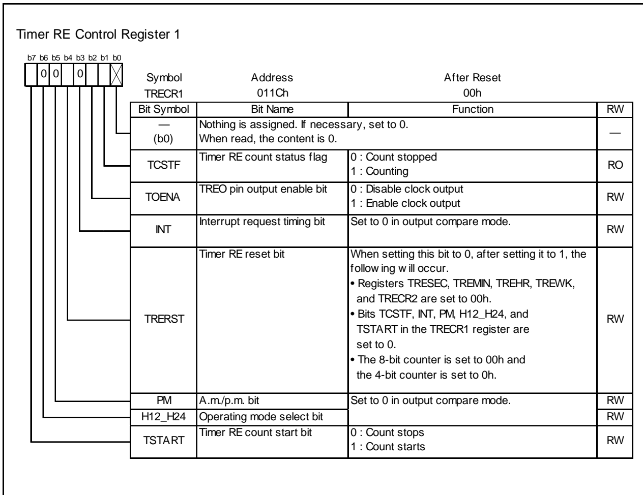
Figure 14.125 TREC1 Register in Output Compare Mode
