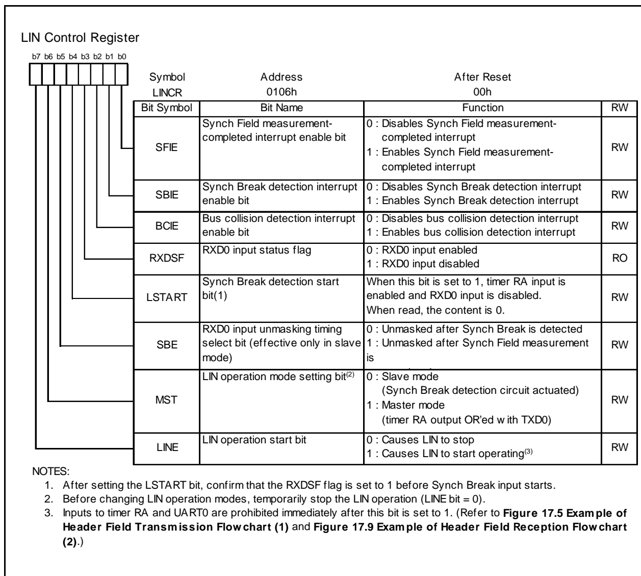
Figure 17.2 LINCR Register
