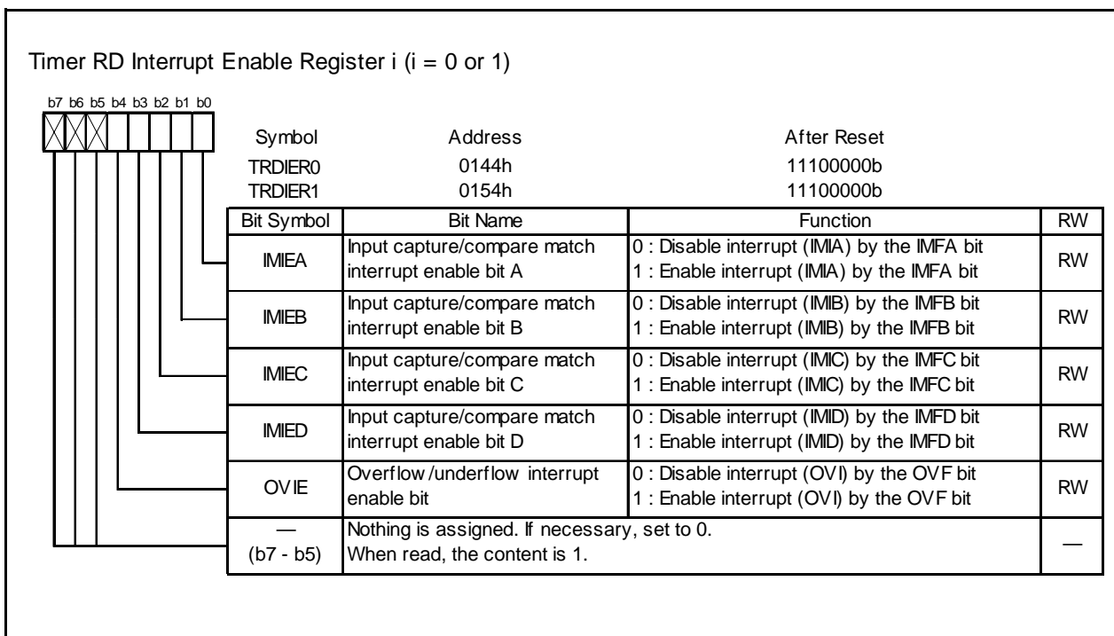
Figure 14.39 Registers TRDIER0 to TRDIER1 in Input Capture Function
