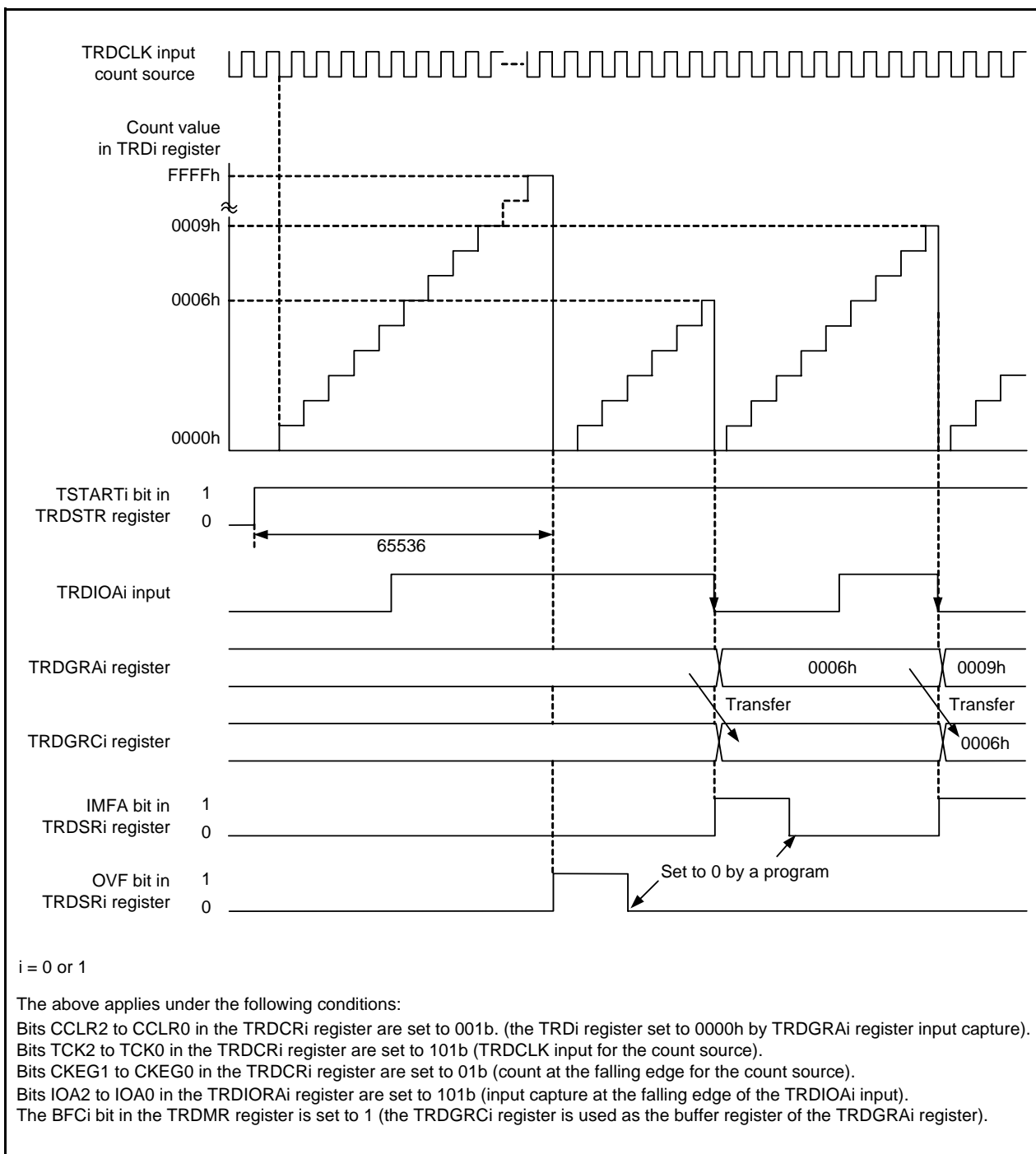
Figure 14.42 Operating Example of Input Capture Function
