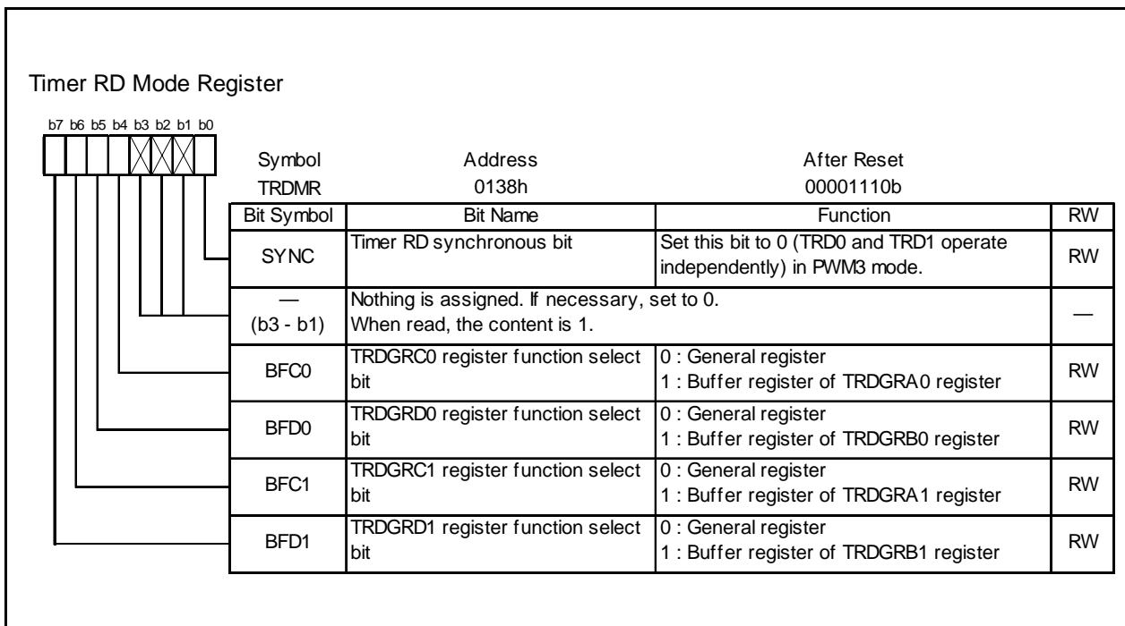
Figure 14.97 TRDMR Register in PWM3 Mode
