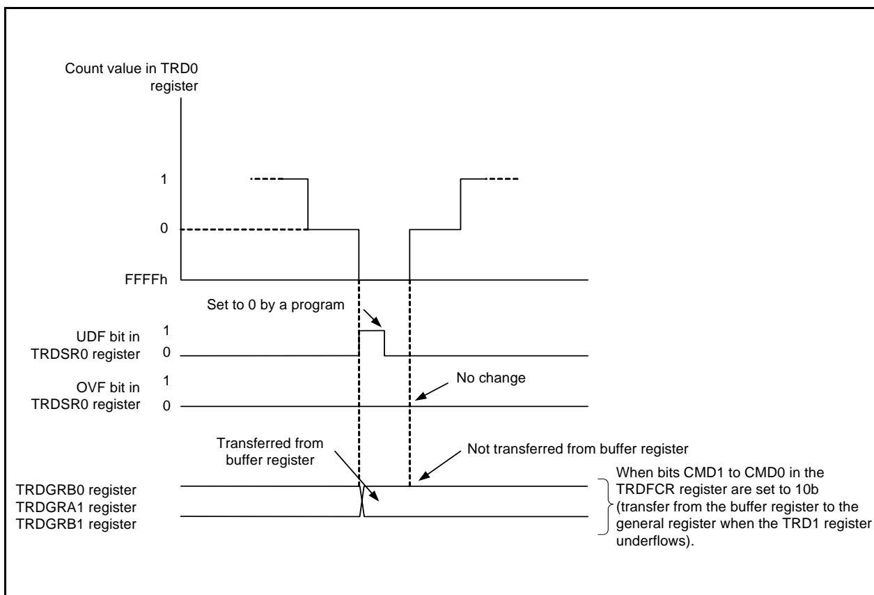
Figure 21.3 Operation when TRD1 Register Underflows in Complementary PWM Mode
