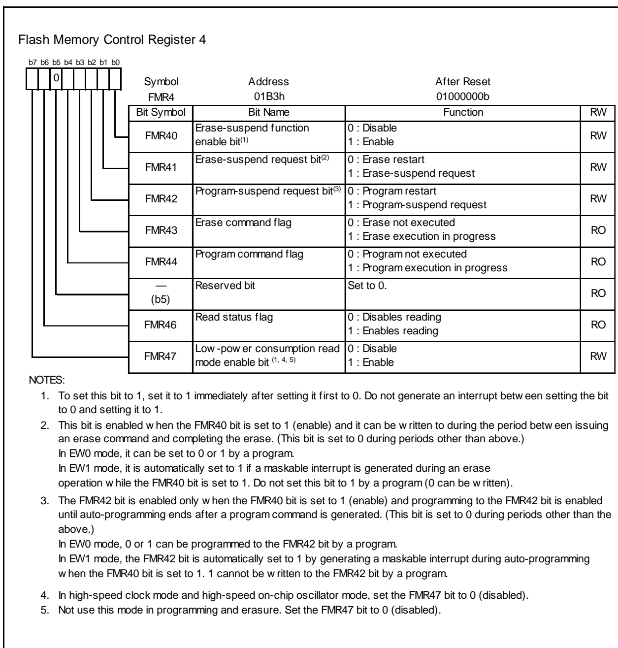
Figure 19.7 FMR4 Register
