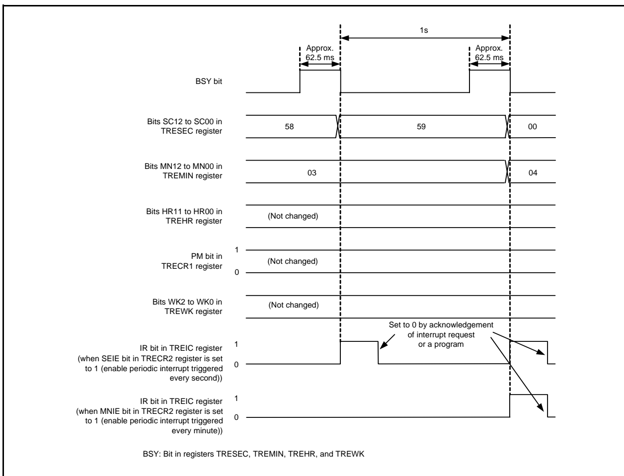
Figure 14.121 Operating Example in Real-Time Clock Mode
