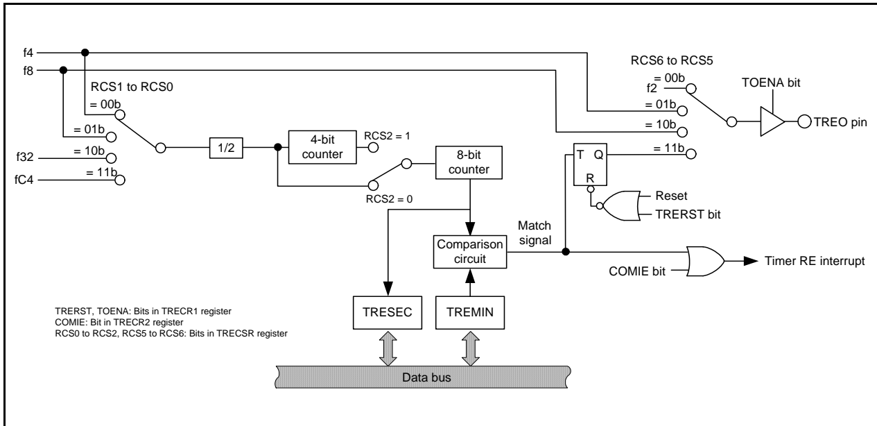
Figure 14.122 Block Diagram of Output Compare Mode
