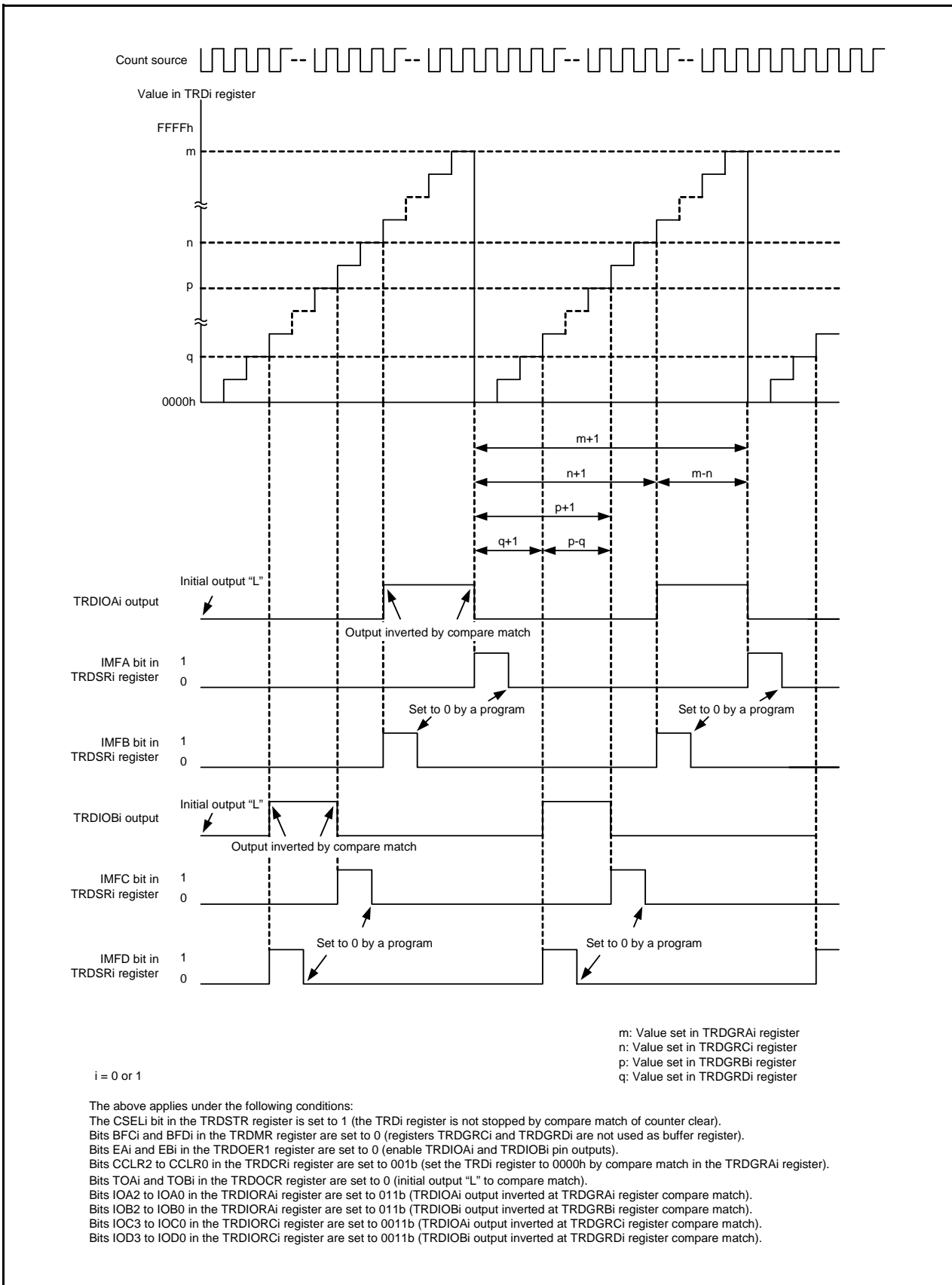
Figure 14.59 Operating Example When TRDGRCi Register is Used for Output Control of TRDIOAi Pin and TRDGRDi Register is Used for Output Control of TRDIOBi Pin
