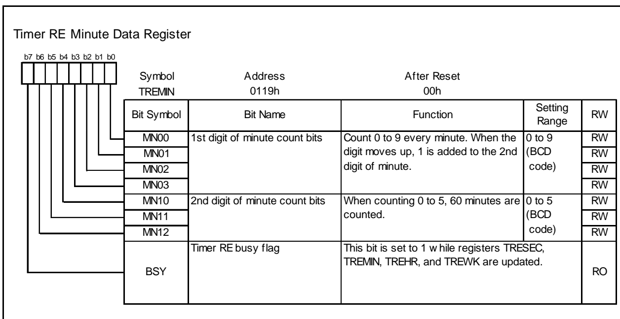
Figure 14.114 TREMIN Register in Real-Time Clock Mode
