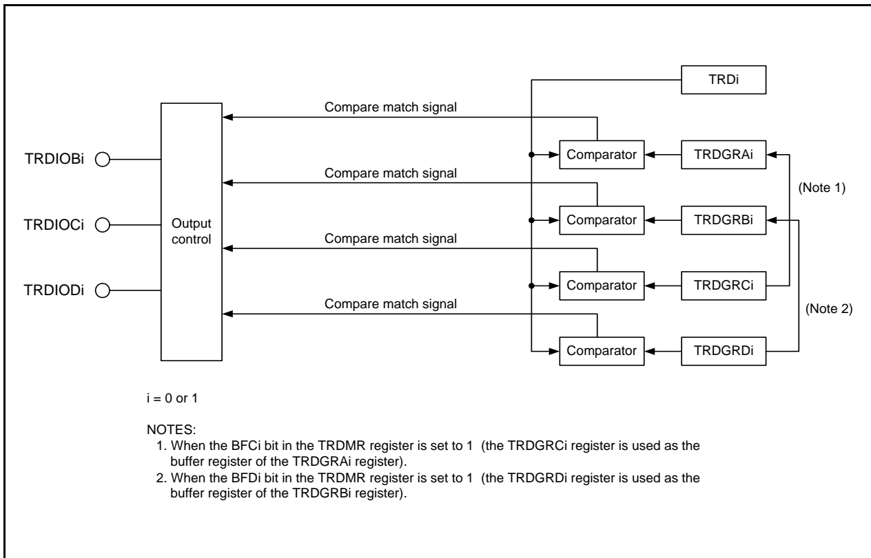
Figure 14.60 Block Diagram of PWM Mode
