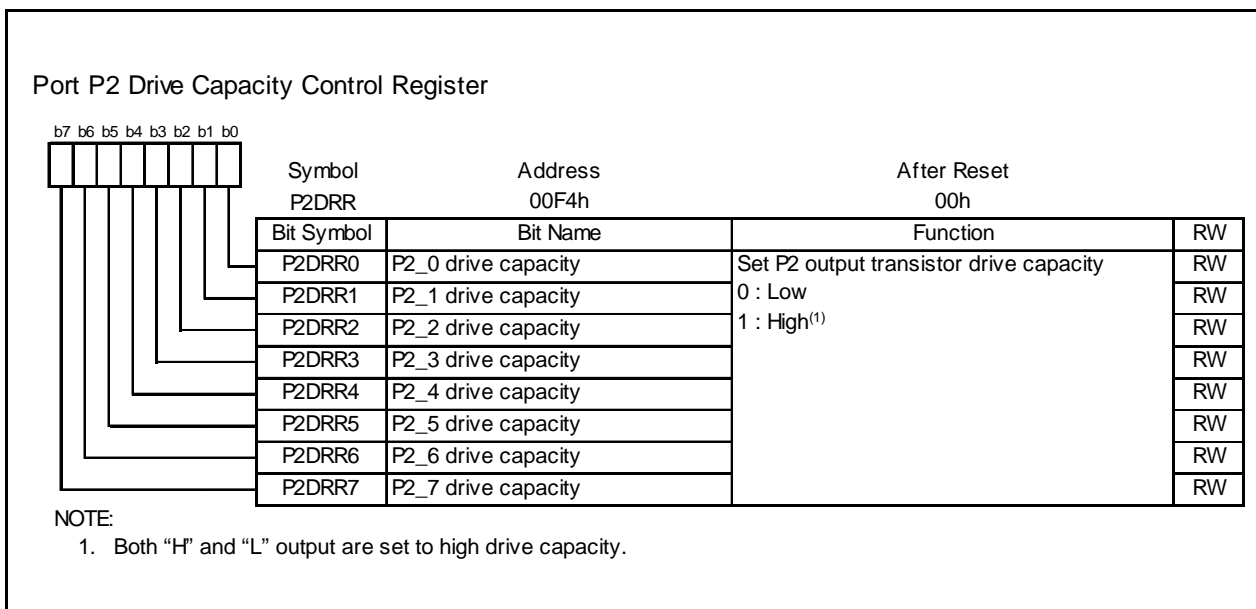
Figure 7.13 P2DRR Register
