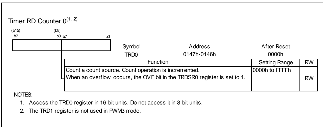
Figure 14.104 TRD0 Register in PWM3 Mode
