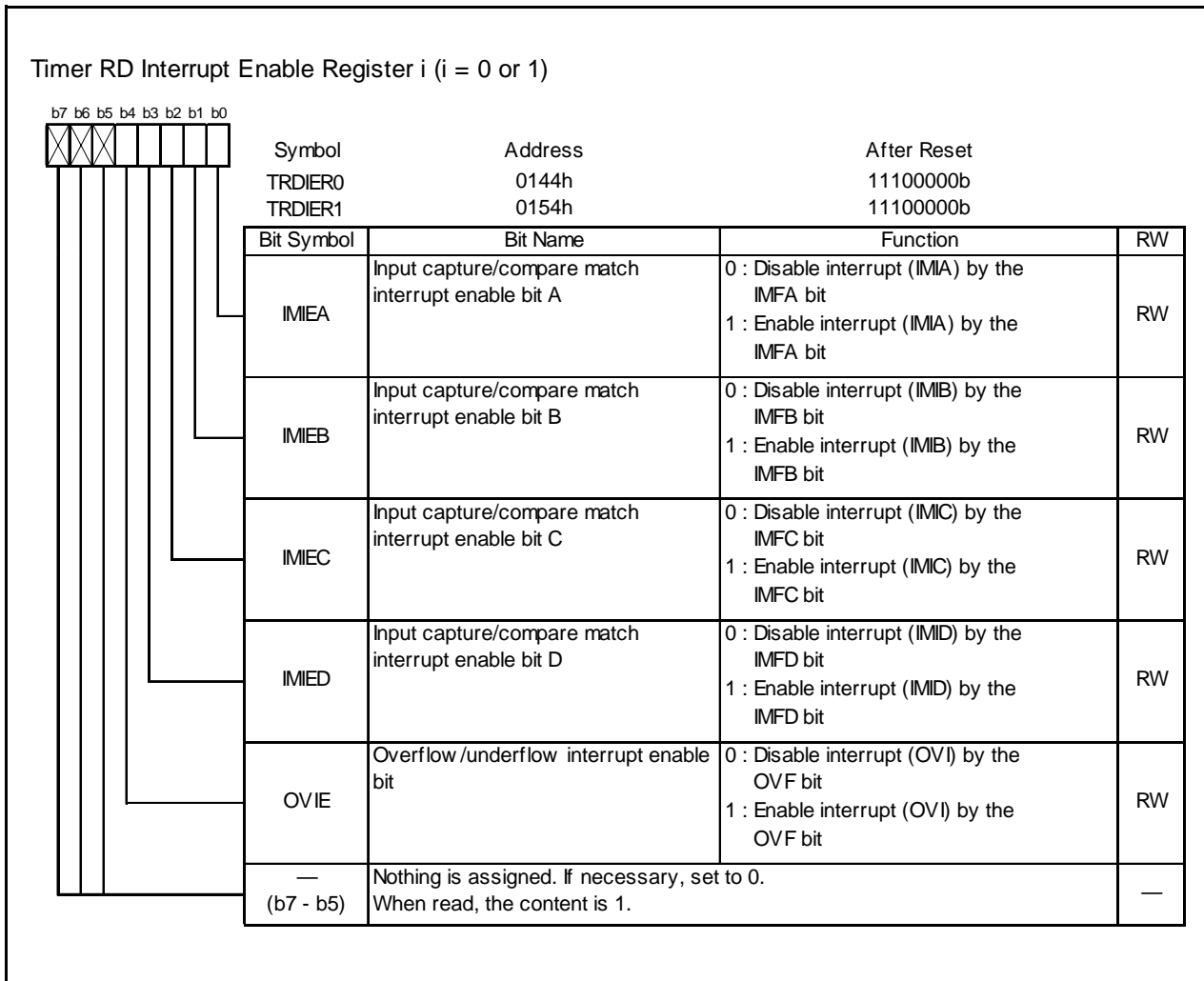
Figure 14.79 Registers TRDIER0 to TRDIER1 in Reset Synchronous PWM Mode
