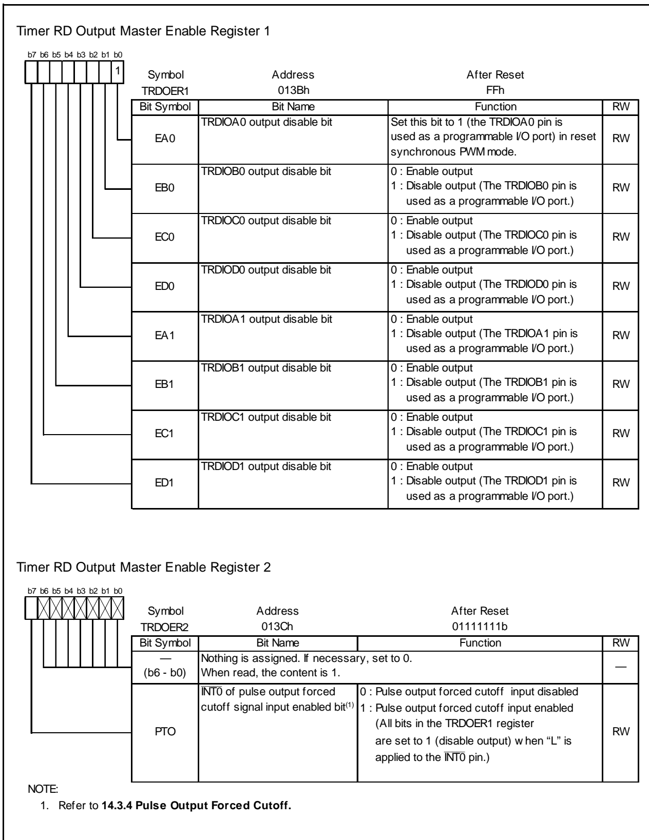
Figure 14.76 Registers TRDOER1 to TRDOER2 in Reset Synchronous PWM Mode
