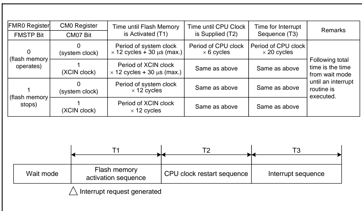
Figure 10.11 Time from Wait Mode to Interrupt Routine Execution
