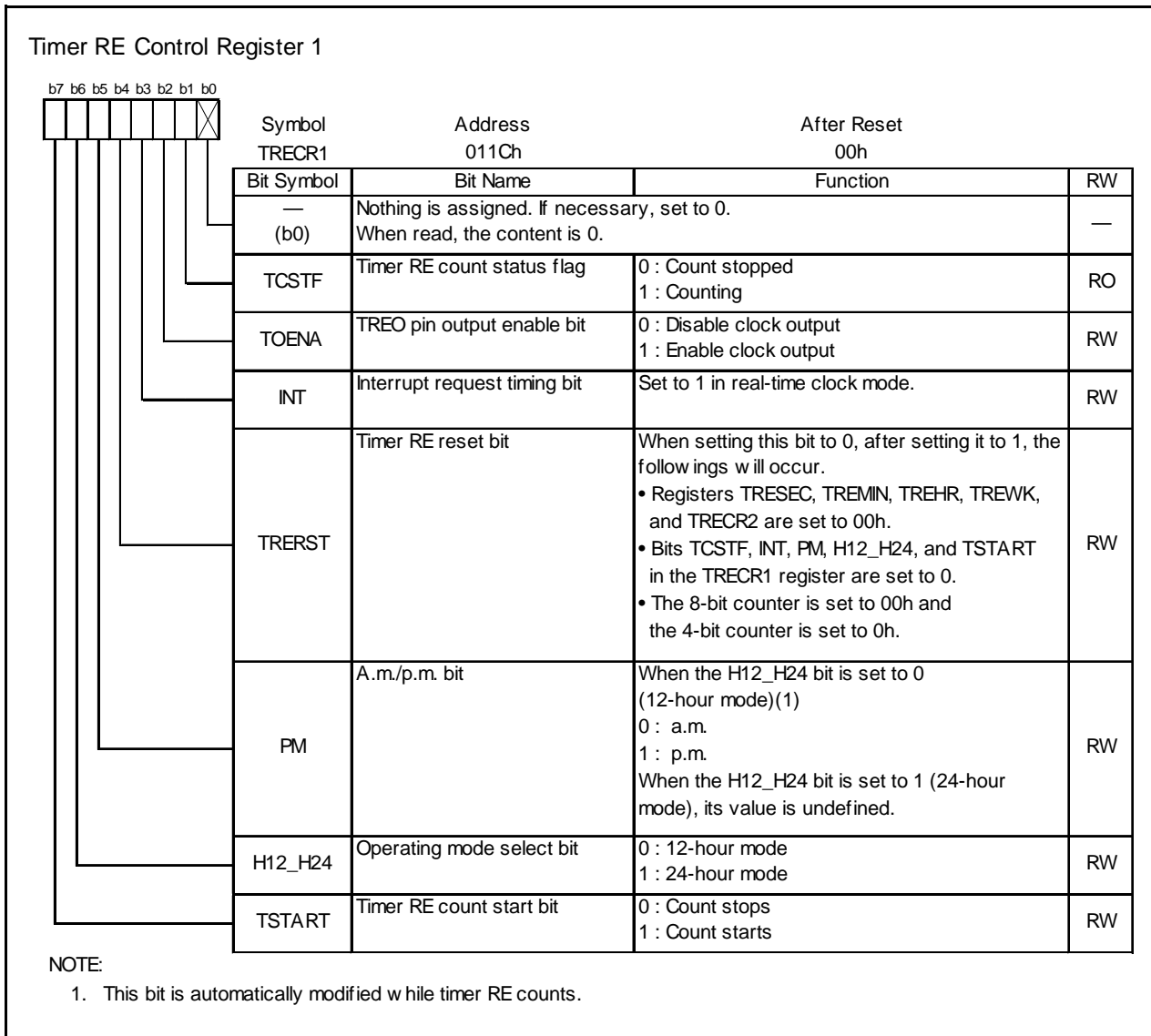
Figure 14.117 TRECR1 Register in Real-Time Clock Mode
