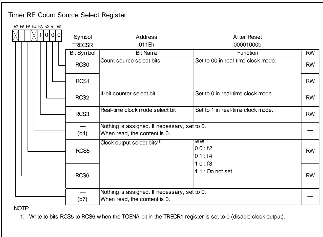
Figure 14.120 TRECSR Register in Real-Time Clock Mode
