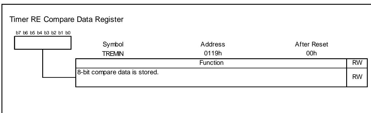
Figure 14.124 TREMIN Register in Output Compare Mode
