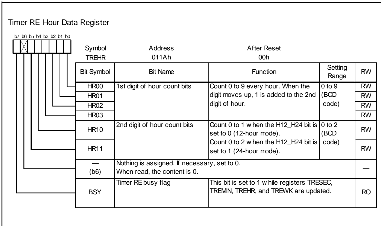
Figure 14.115 TREHR Register in Real-Time Clock Mode
