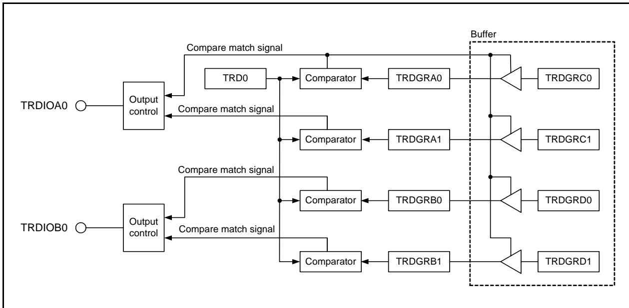
Figure 14.95 Block Diagram of PWM3 Mode
