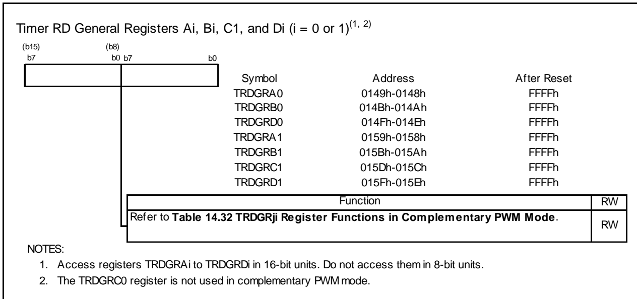
Figure 14.92 Registers TRDGRAi, TRDGRBi, TRDGRC1, and TRDGRDi in Complementary PWM Mode
