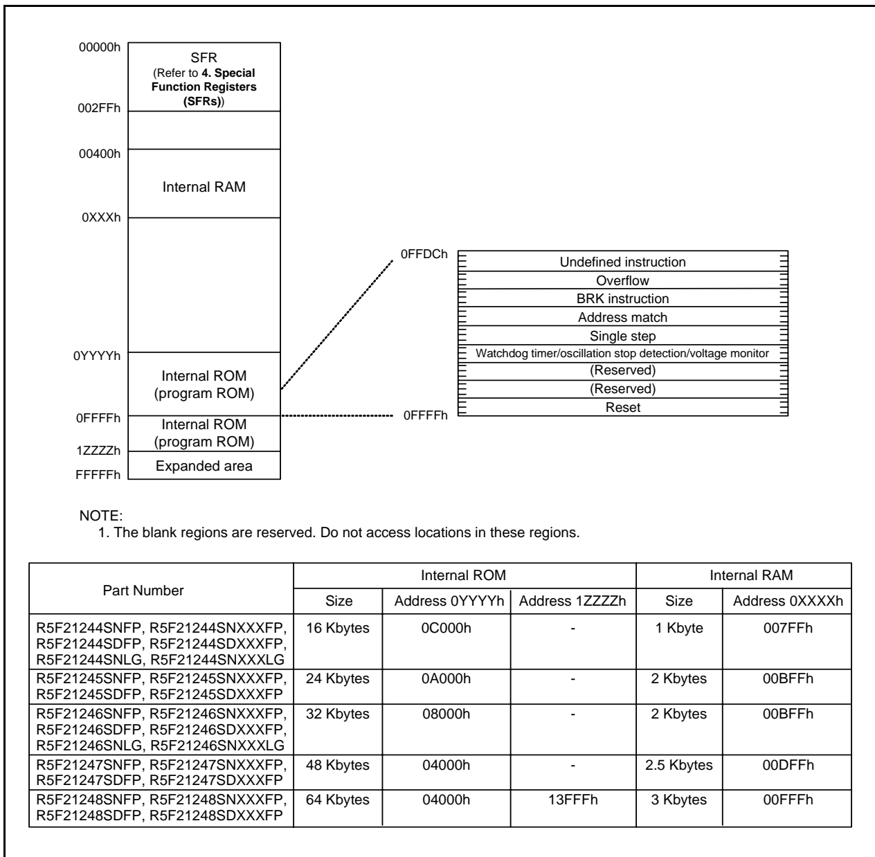
Figure 3.1 Memory Map of R8C/24 Group
