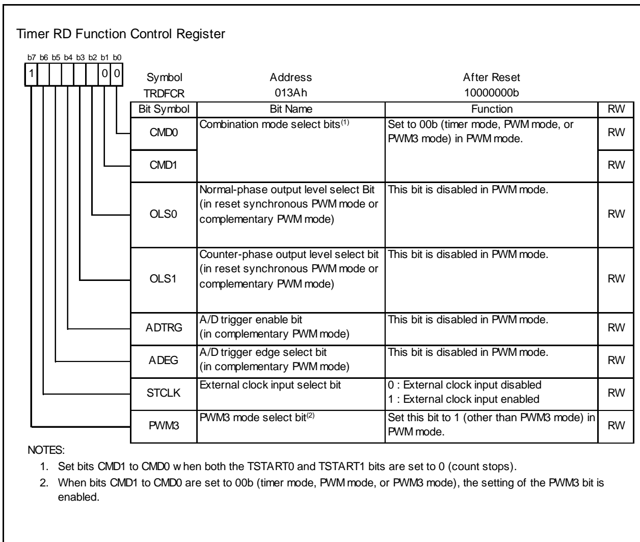
Figure 14.63 TRDFCR Register in PWM Mode
