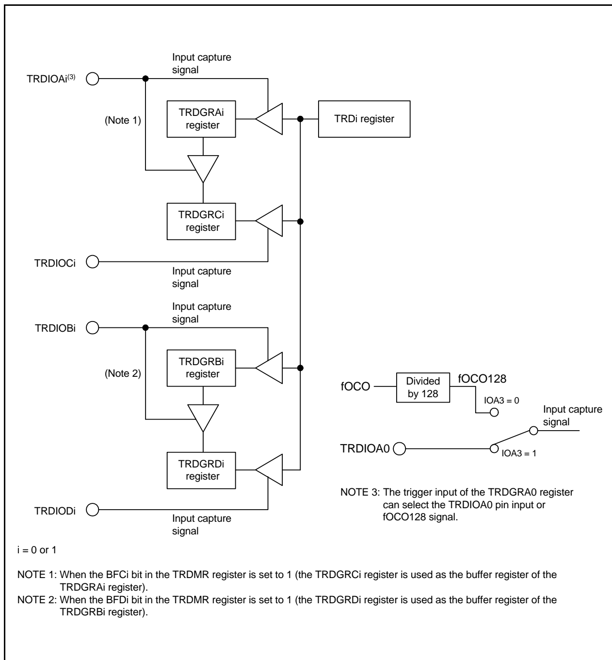
Figure 14.30 Block Diagram of Input Capture Function
