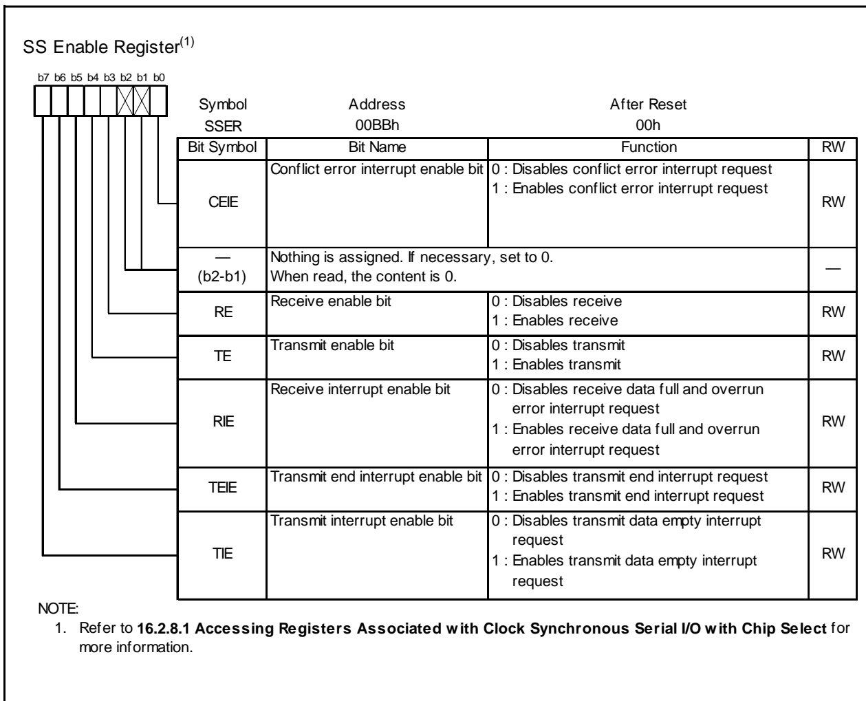
Figure 16.5 SSER Register
