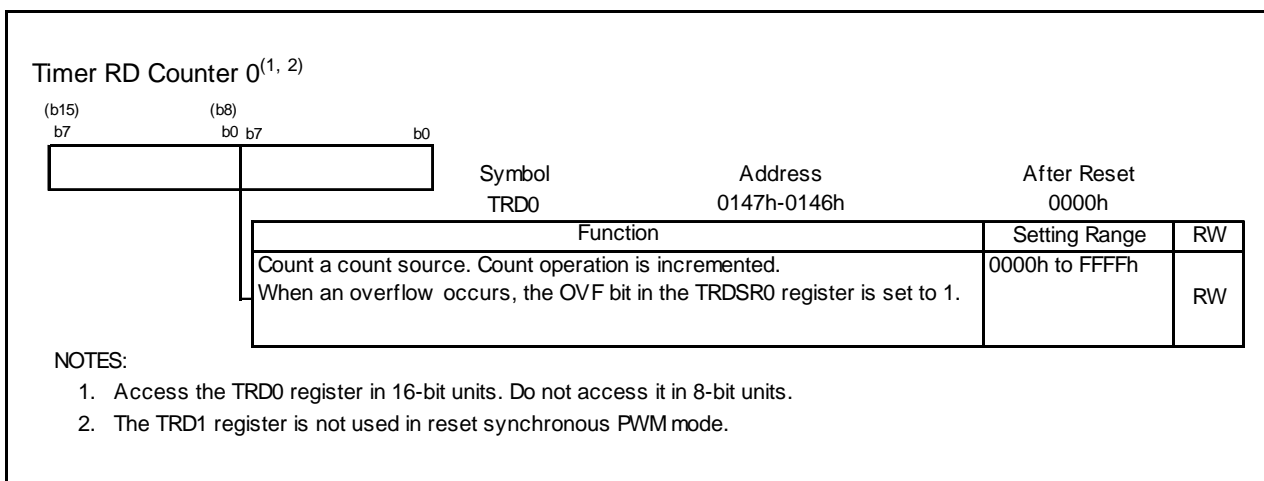
Figure 14.80 TRD0 Registrar in Reset Synchronous PWM Mode
