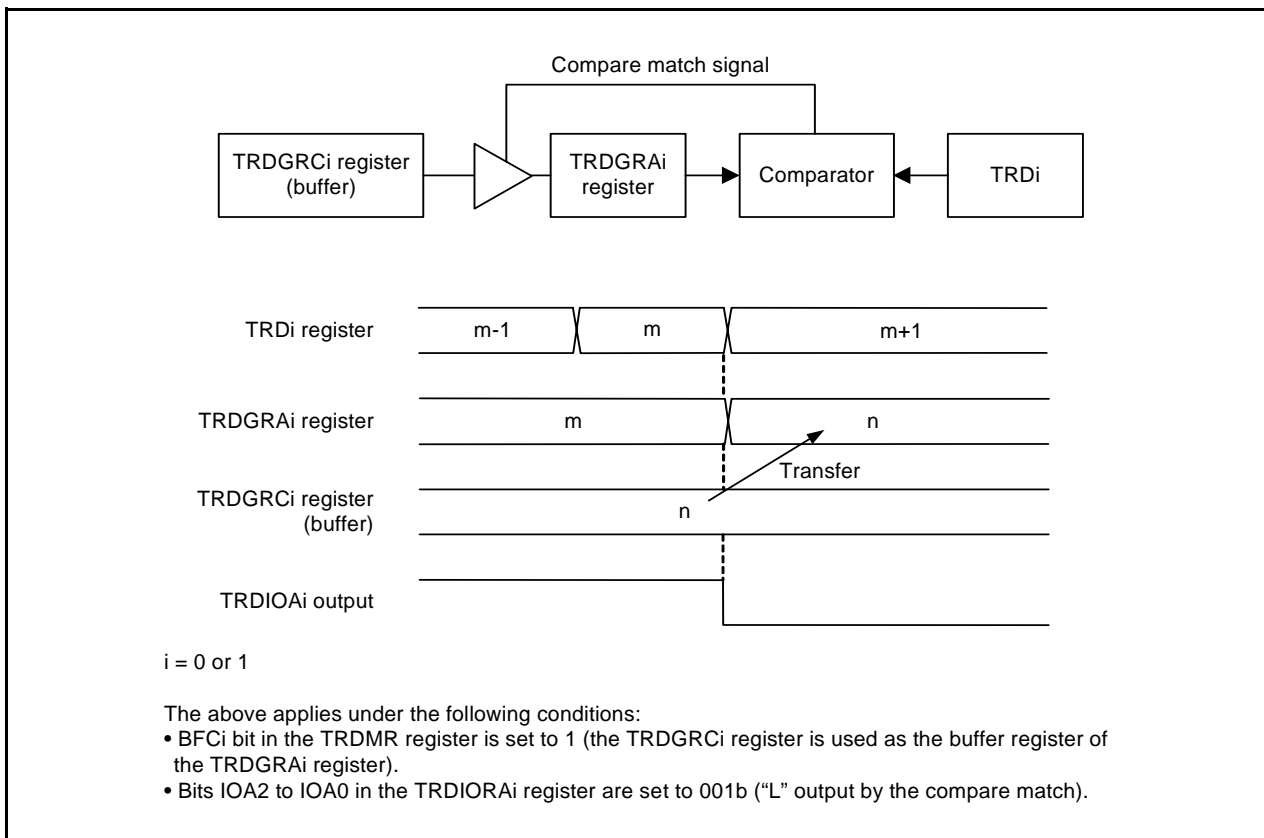
Figure 14.27 Buffer Operation in Output Compare Function
