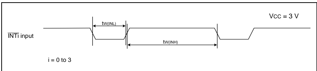
Figure 20.15 External Interrupt INT i Input Timing Diagram when Vcc = 3 V
