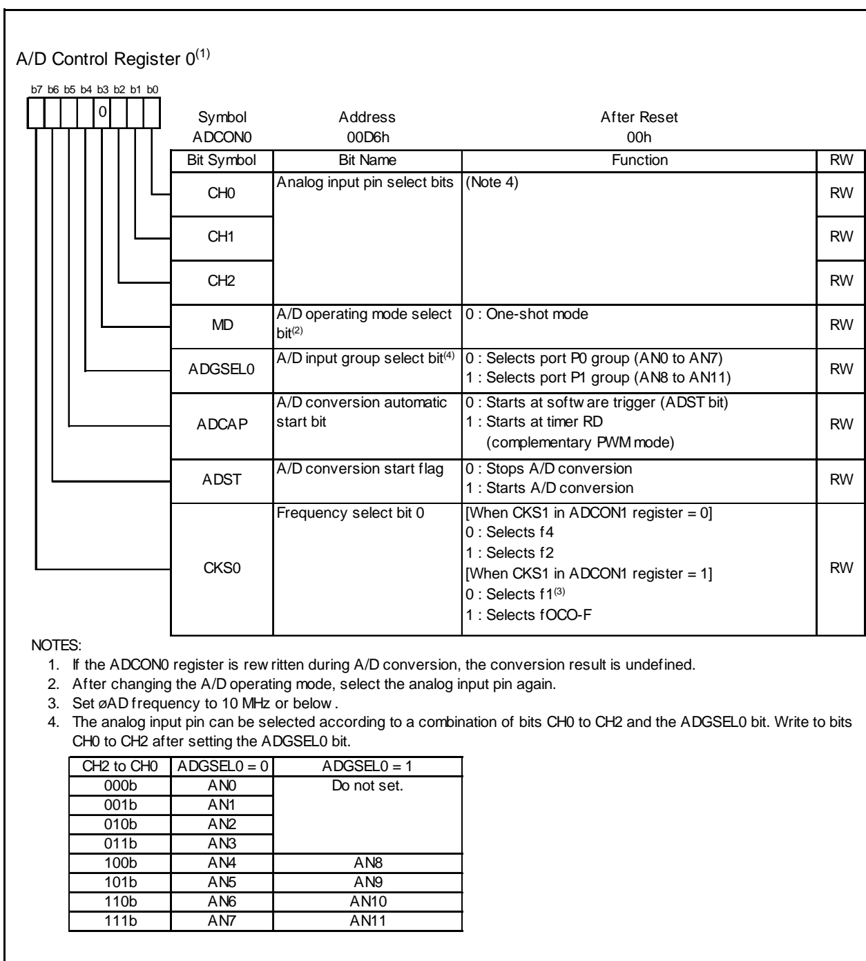
Figure 18.4 ADCON0 Register in One-Shot Mode
