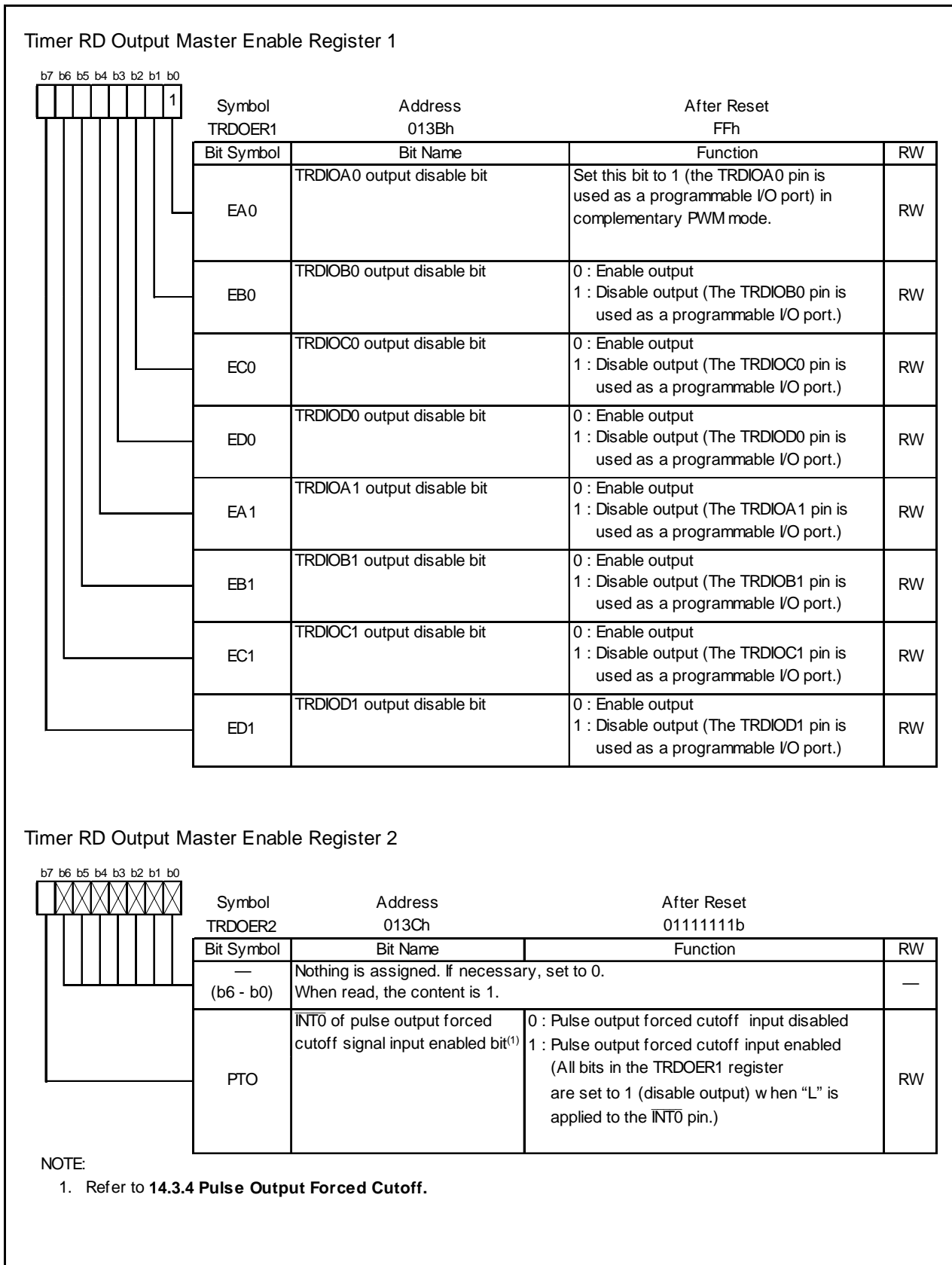
Figure 14.87 Registers TRDOER1 to TRDOER2 in Complementary PWM Mode
