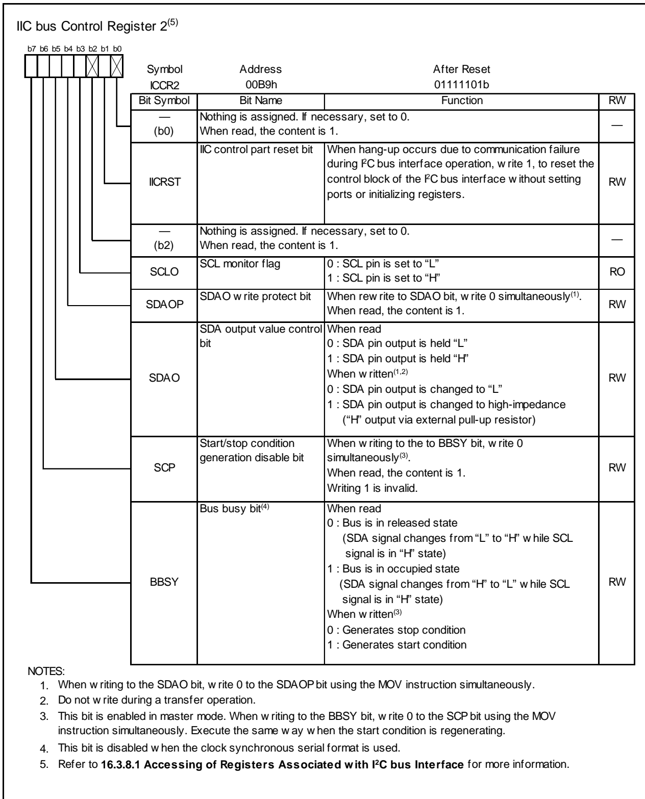
Figure 16.25 ICCR2 Register
