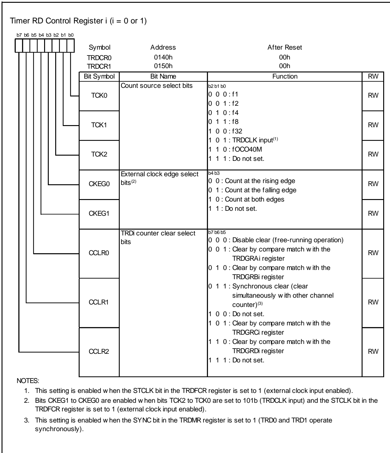
Figure 14.50 Registers TRDCR0 to TRDCR1 in Output Compare Function
