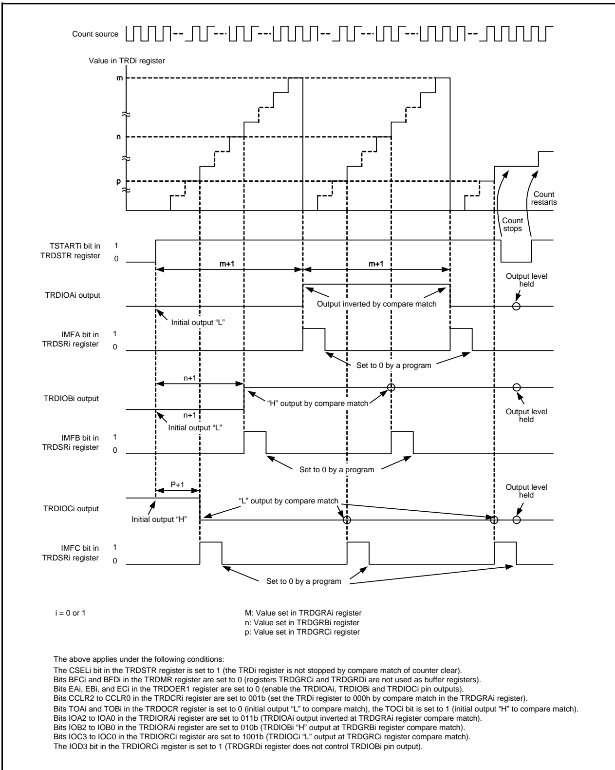
Figure 14.57 Operating Example of Output Compare Function
