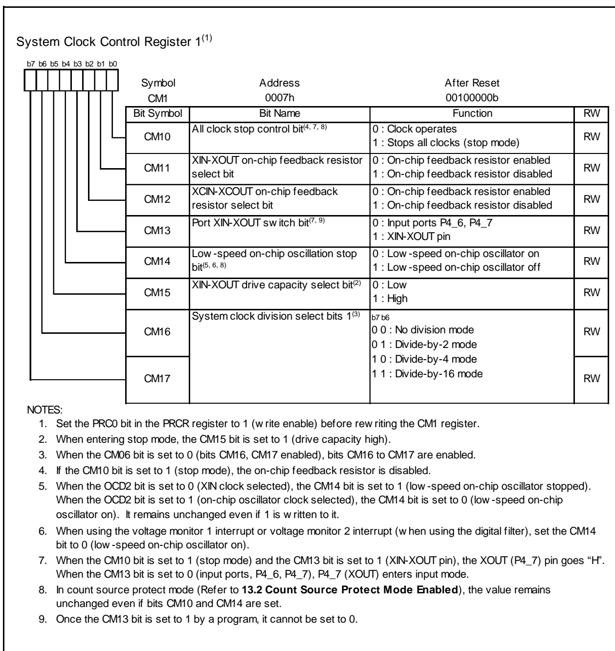
Figure 10.3 CM1 Register
