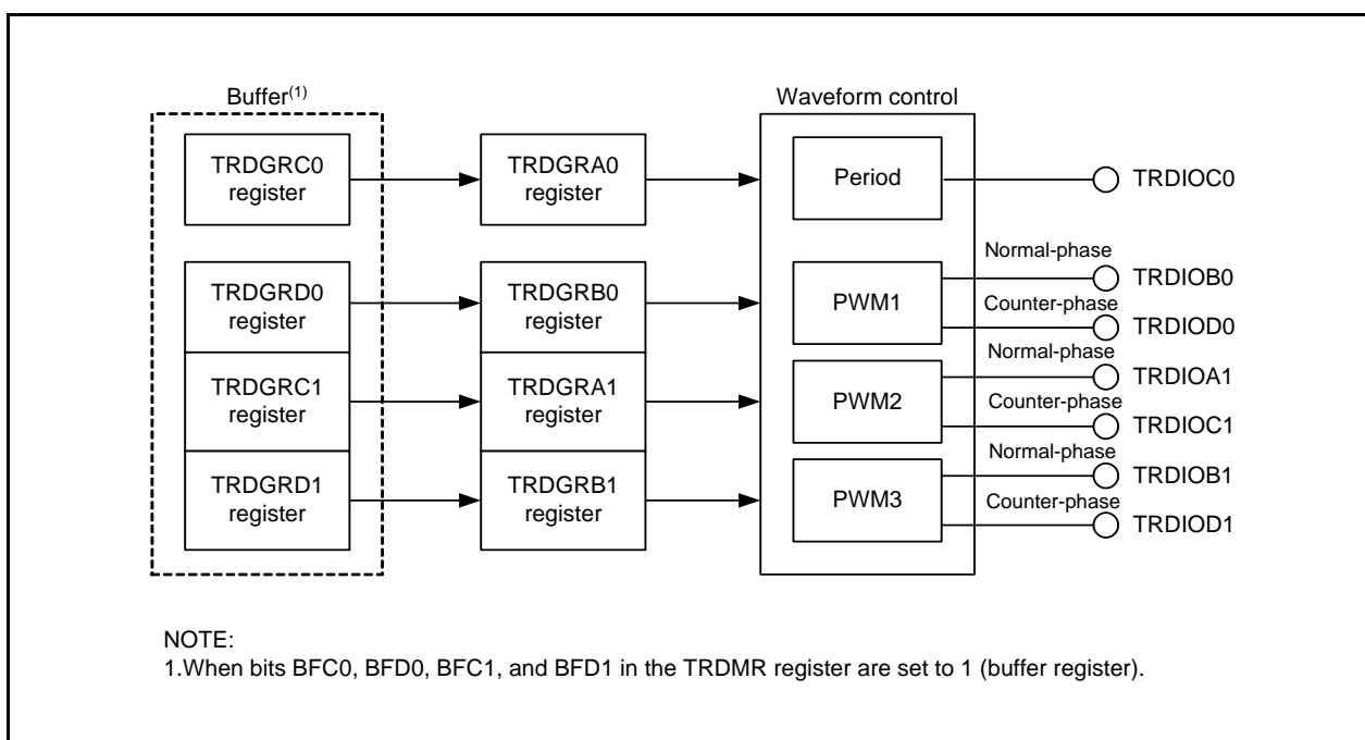
Figure 14.73 Block Diagram of Reset Synchronous PWM Mode
