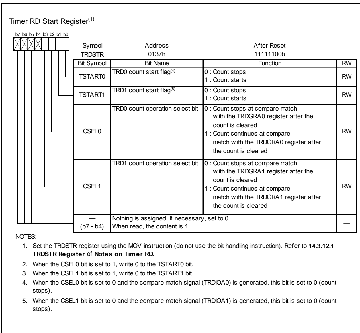
Figure 14.84 TRDSTR Register in Complementary PWM Mode
