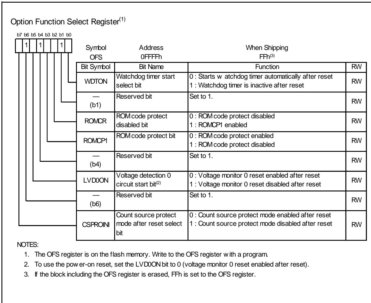
Figure 5.4 OFS Register
