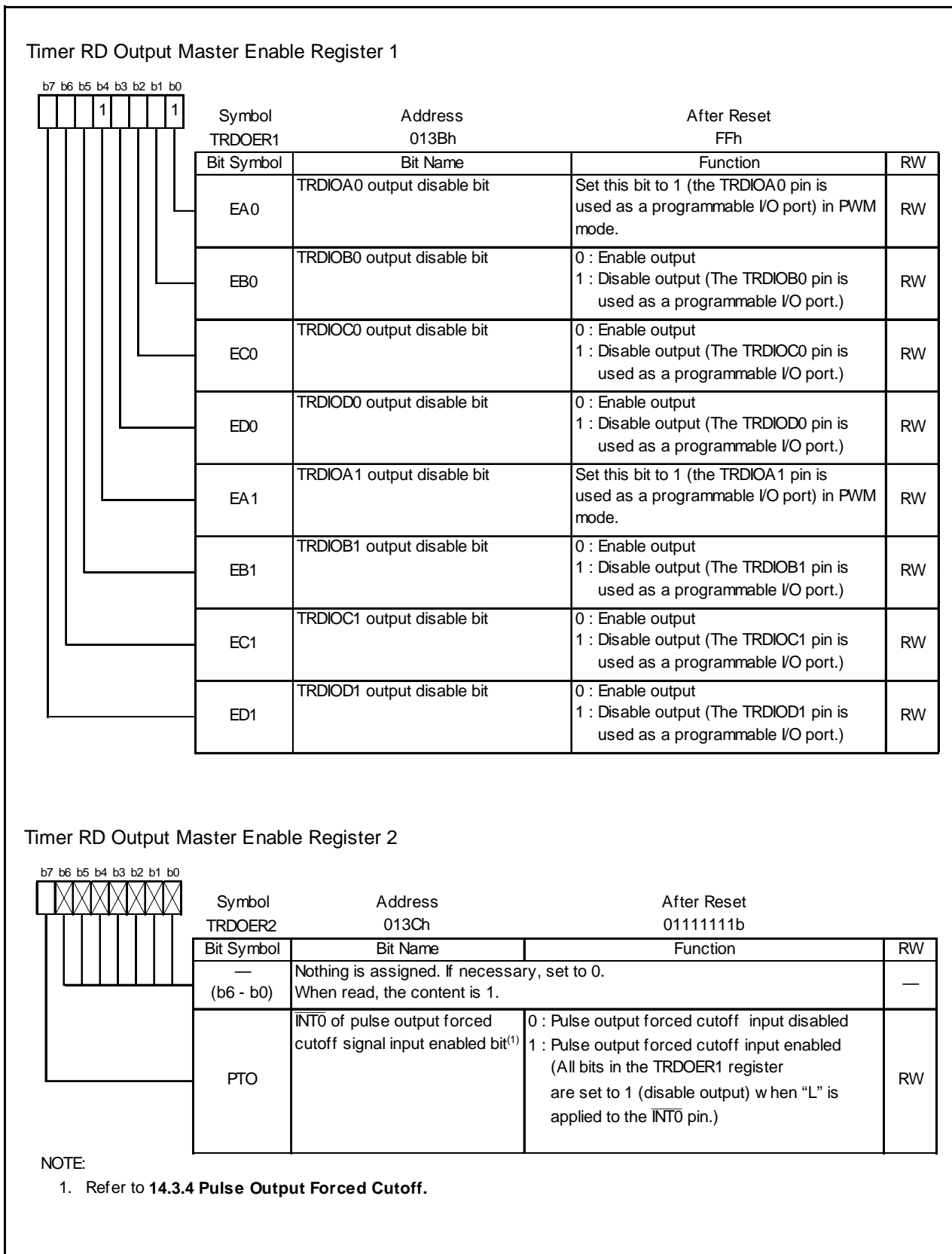
Figure 14.64 Registers TRDOER1 to TRDOER2 in PWM Mode
