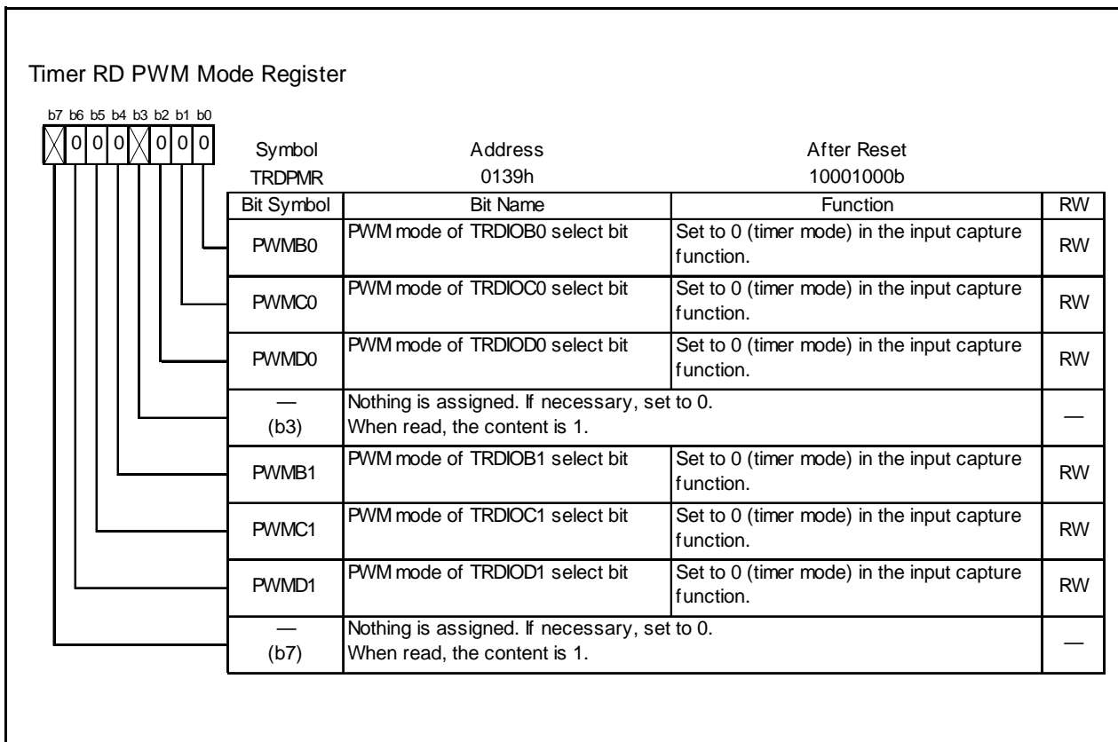
Figure 14.32 TRDPMR Register in Input Capture Function
