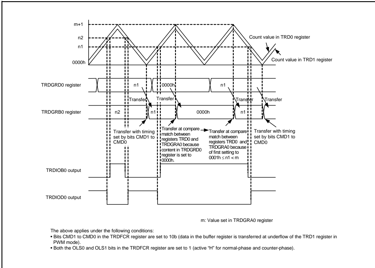
Figure 14.111 Operation when Value in Buffer Register Is Set to 0000h in Complementary PWM Mode
