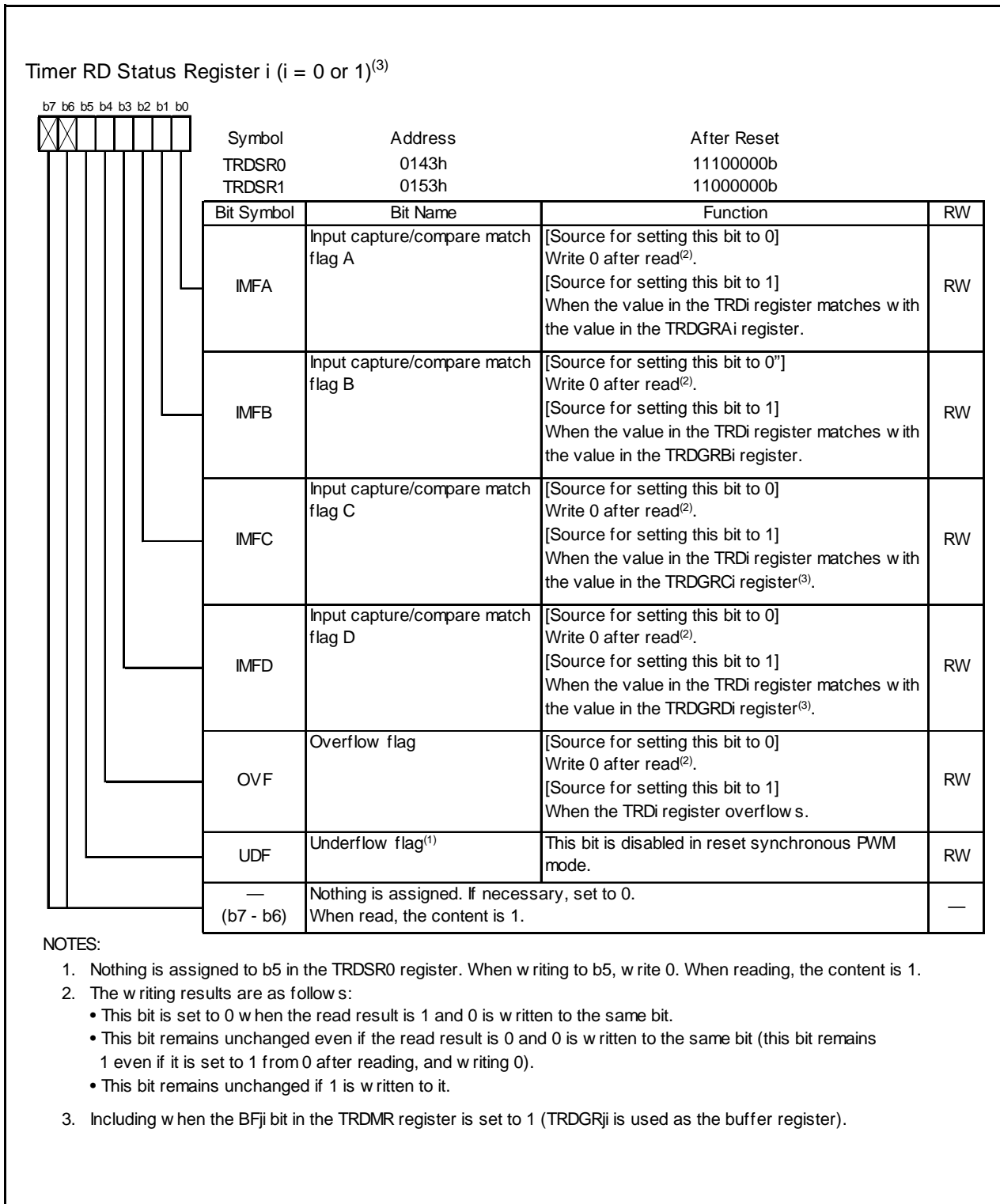
Figure 14.78 Registers TRDSR0 to TRDSR1 in Reset Synchronous PWM Mode
