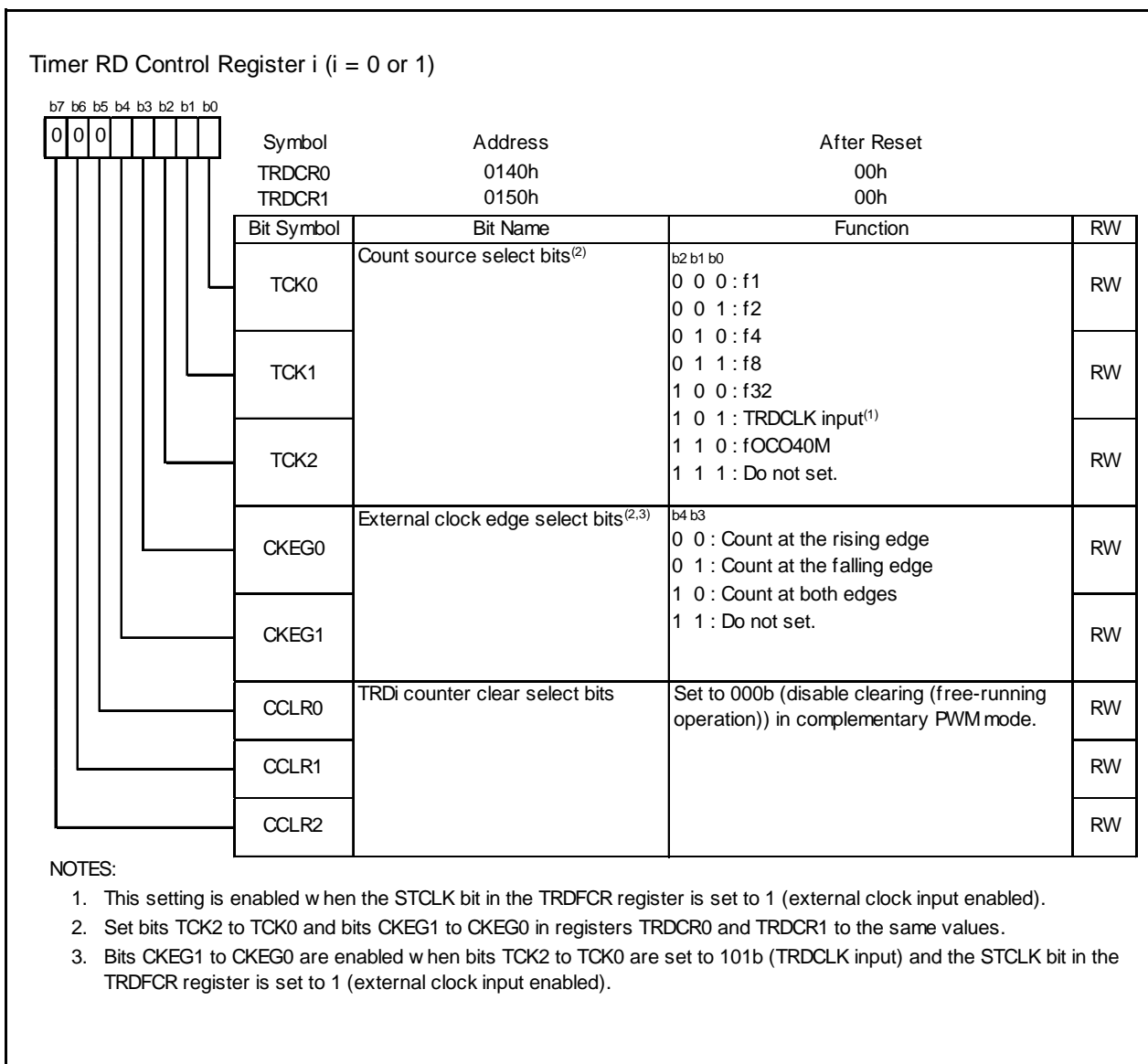
Figure 14.88 Registers TRDCR0 to TRDCR1 in Complementary PWM Mode
