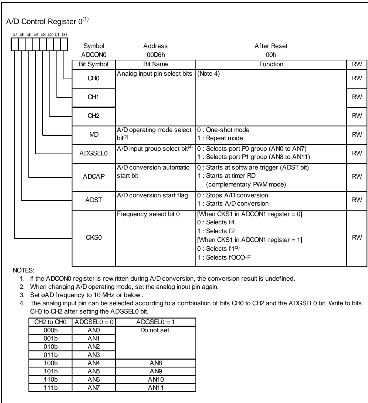
Figure 18.2 ADCON0 Register
