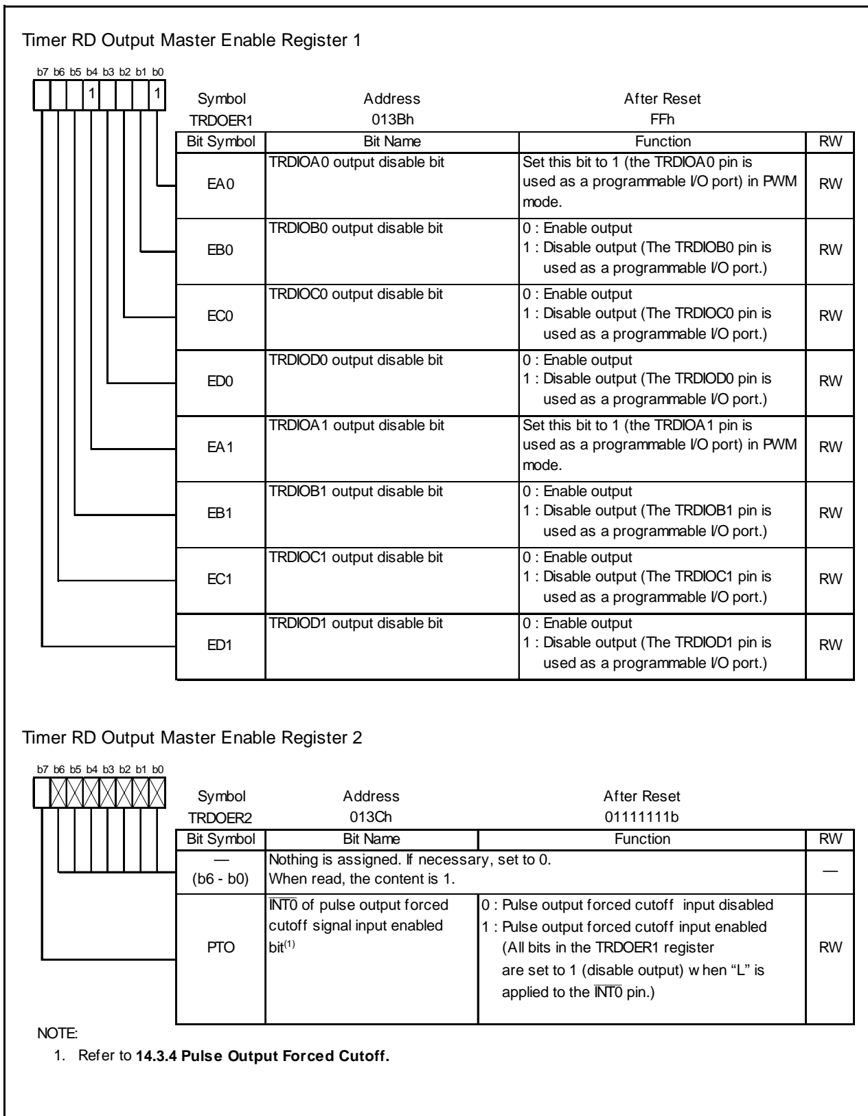
Figure 14.48 Registers TRDOER1 to TRDOER2 in Output Compare Function
