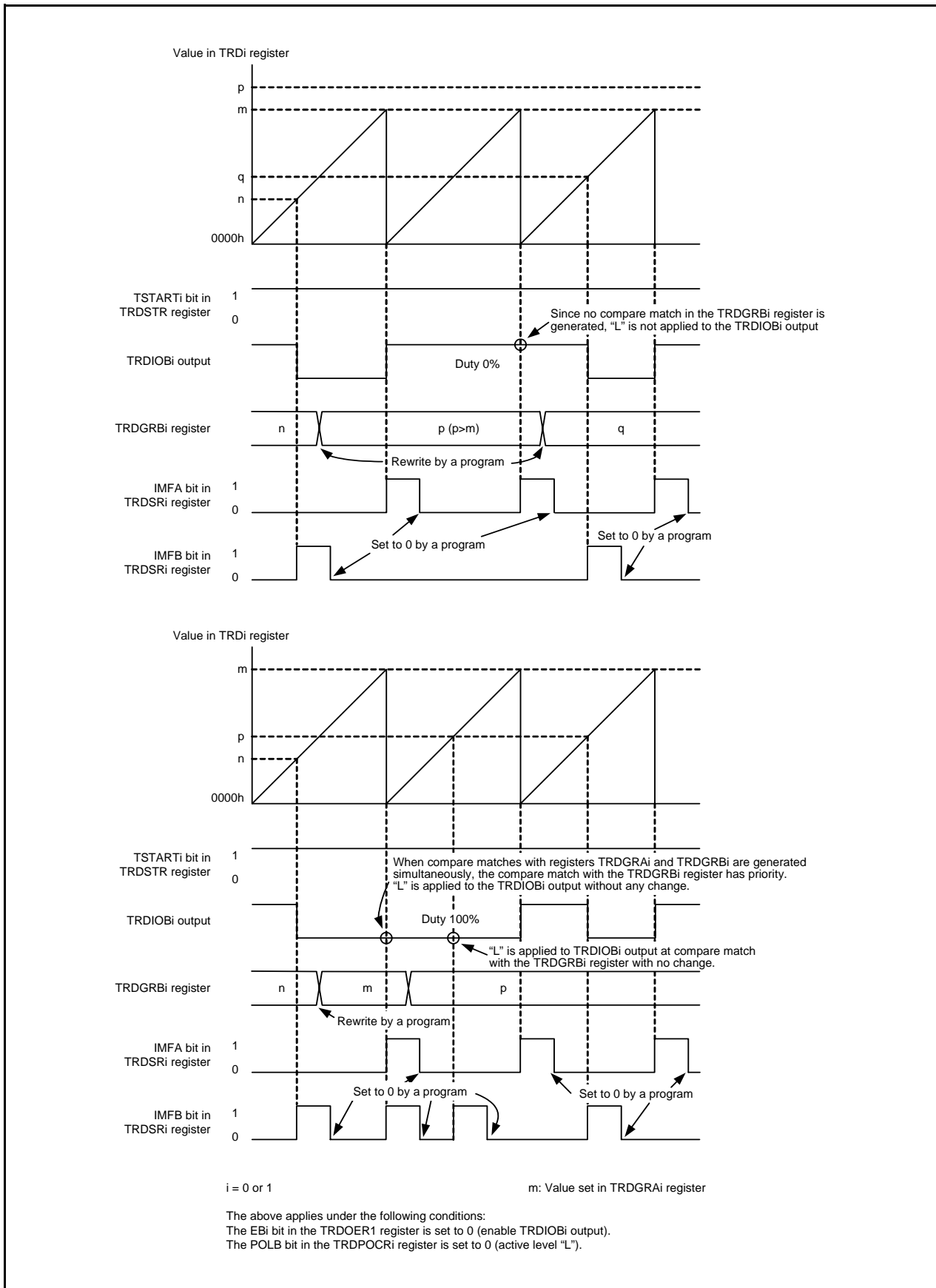
Figure 14.72 Operating Example of PWM Mode (Duty 0%, Duty 100%)
