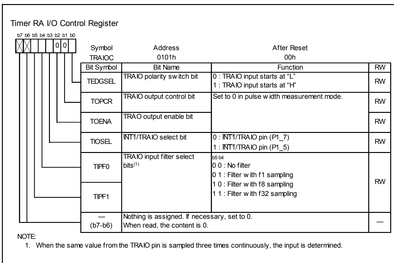
Figure 14.8 TRAI/O Register in Pulse Width Measurement Mode
