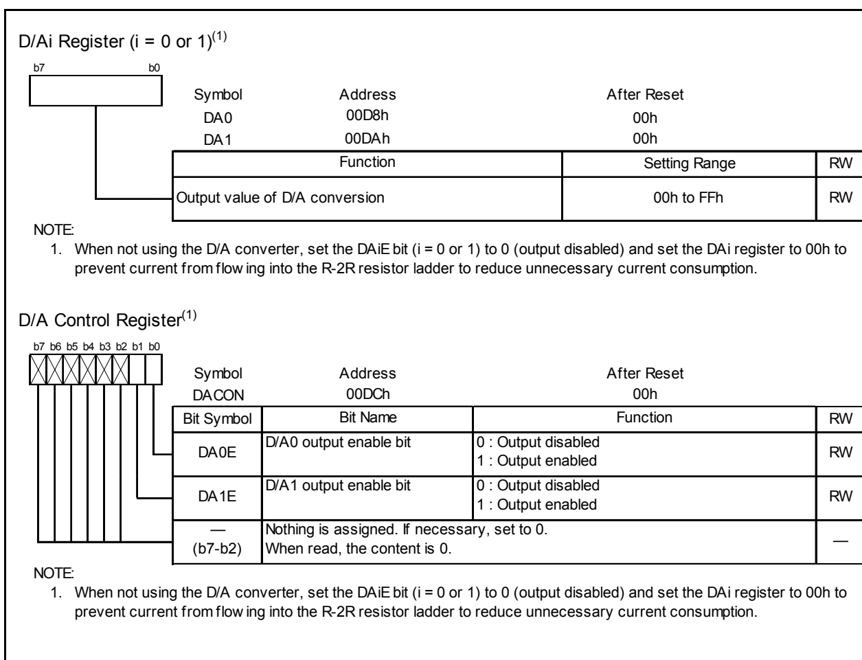
Figure 19.2 Registers DA0 to DA1 and DAON
