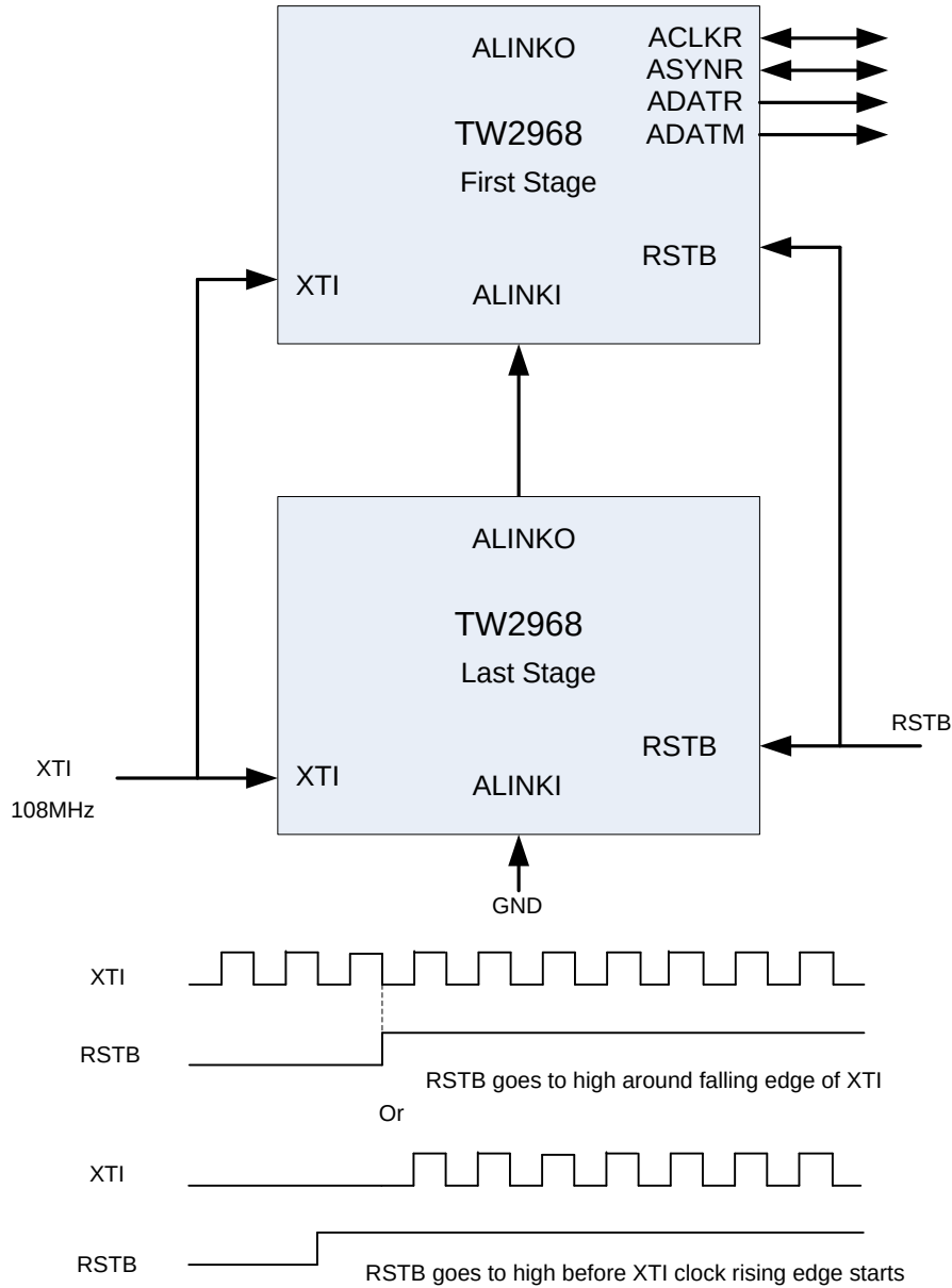
FIGURE 13. RSTB CONTROL FOR 108MHZ XT INPUT
