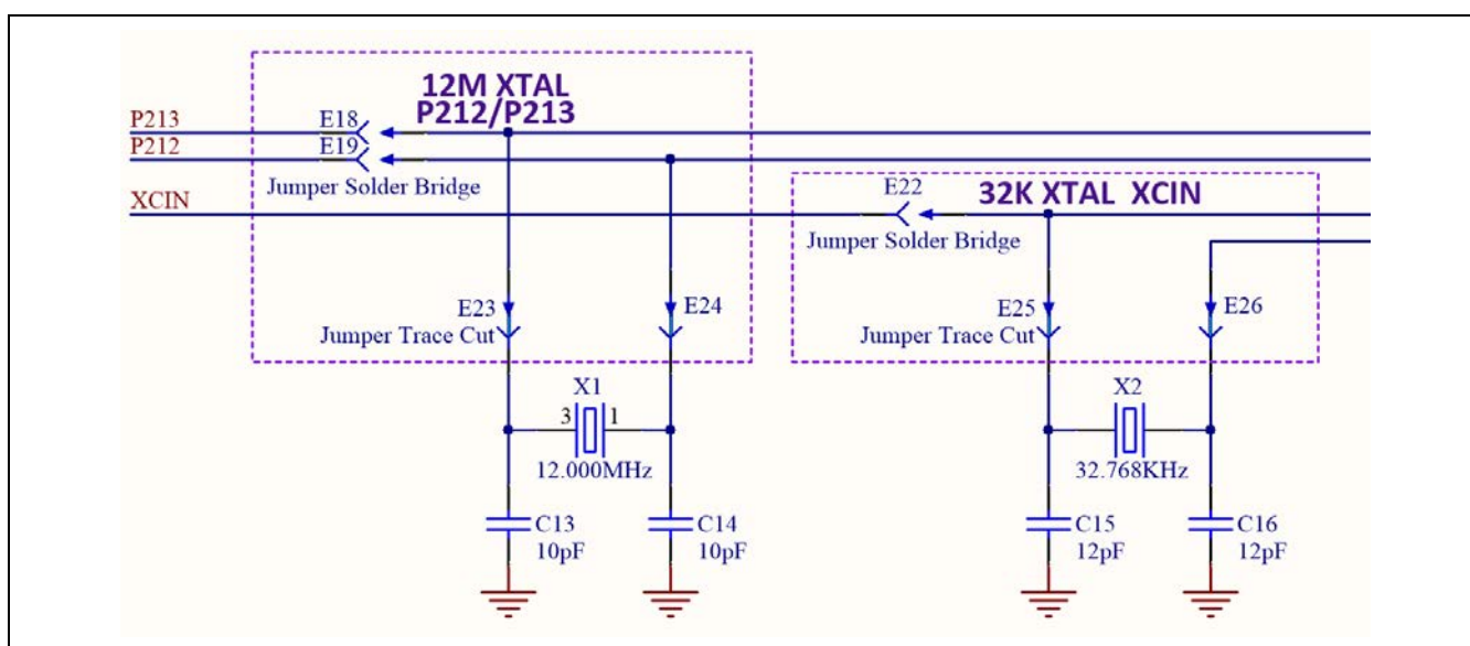
Figure 22 Crystal Clock sources
