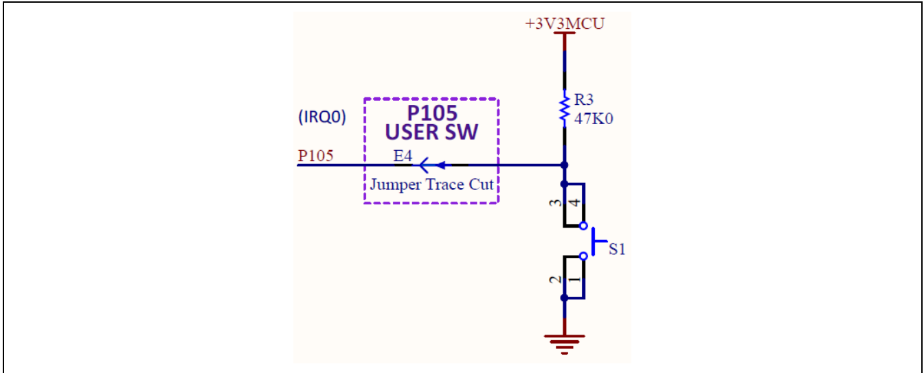
Figure 13 User Switch Circuit
