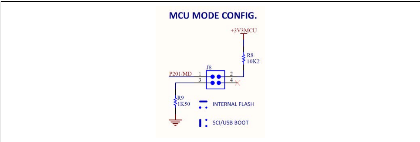
Figure 26: Boot Mode Configuration Circuit
