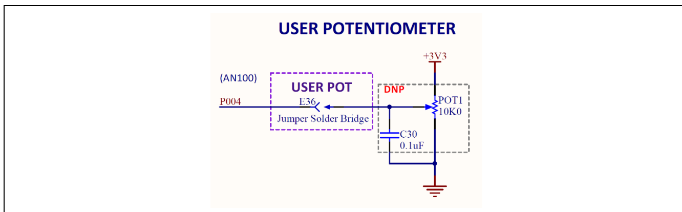
Figure 23 User Potentiometer Circuit
