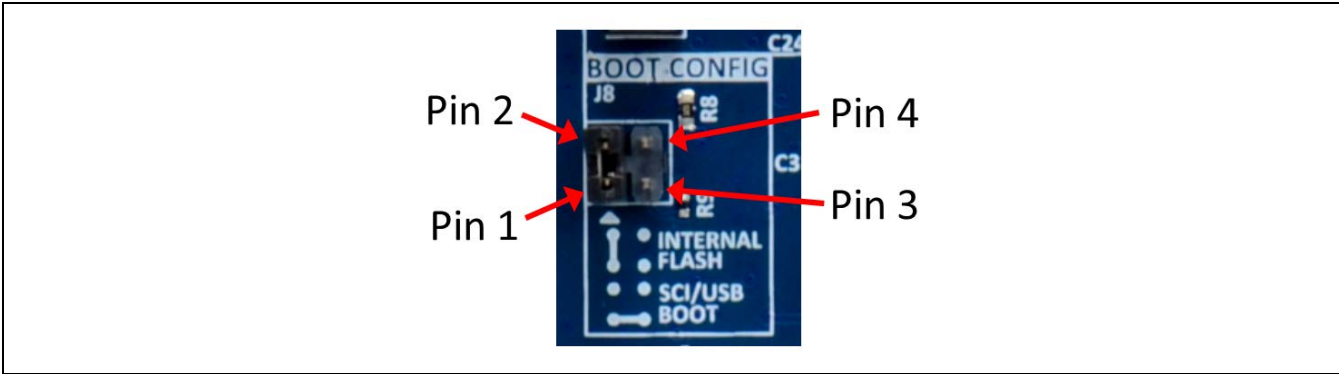
Figure 25 Boot Configuration Header
