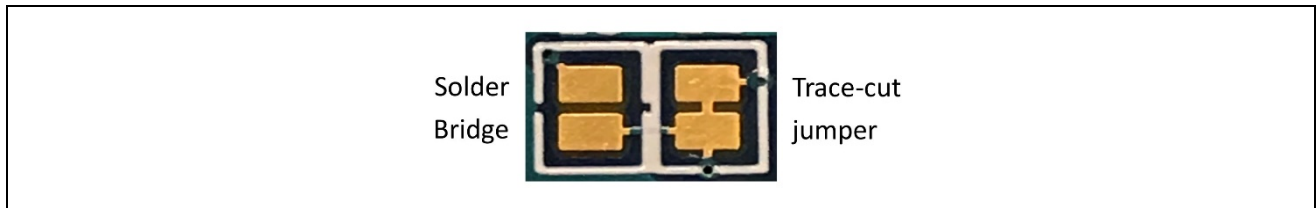
Figure 3. Copper Jumpers
