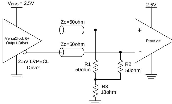
Figure 16. 2.5V LVPECL Output Termination (2)
