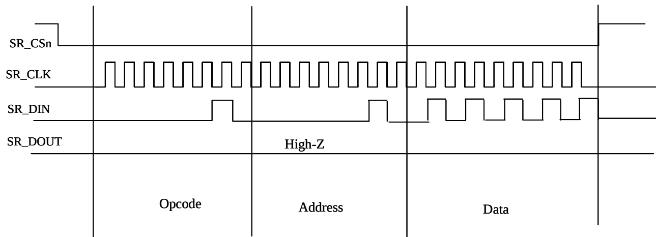
Figure 33: 9-bit EEPROM Write Timing
