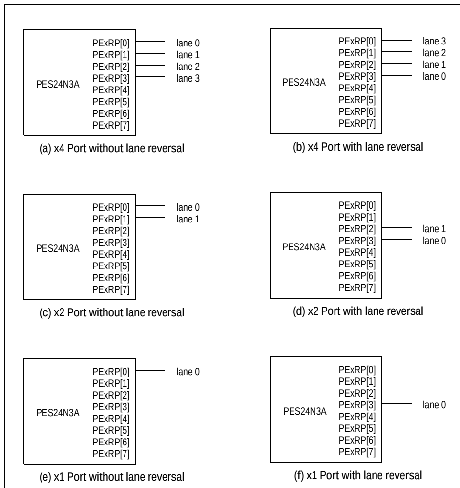
Figure 4.2 Port Lane Reversal for Maximum Link Width of x4 (MAXLNKWIDTH[5:0]=0x4)
