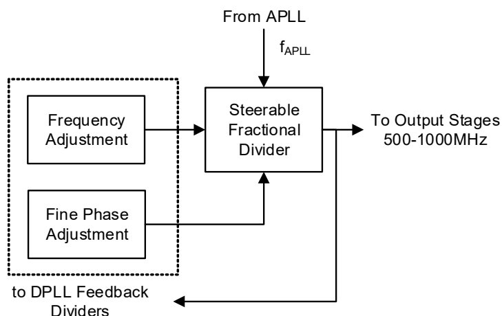
Figure 14. Steerable Fractional Divider Block
