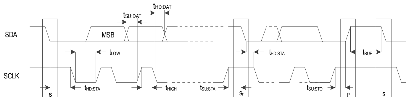
Figure 20. I 2 C Slave Timing Diagram
