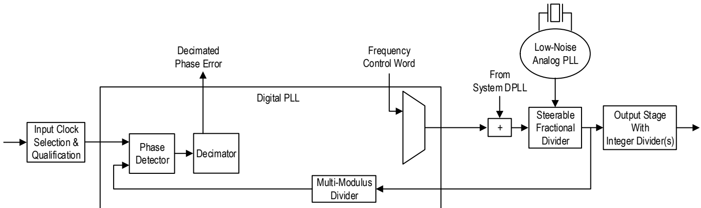
Figure 28. Jitter Attenuator Operation with External Digital Loop Filter
