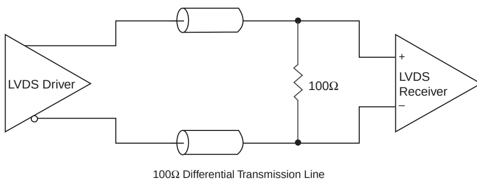
Figure 39. Standard LVDS Termination
