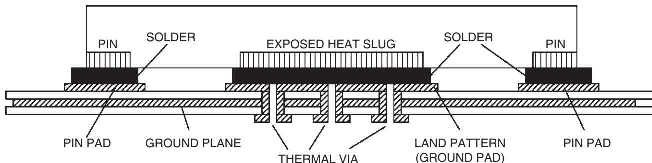
Figure 40. P.C. Assembly for Exposed Pad Thermal Release Path – Side View (Drawing Not to Scale)
