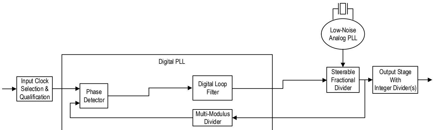
Figure 27. Jitter Attenuator Operation
