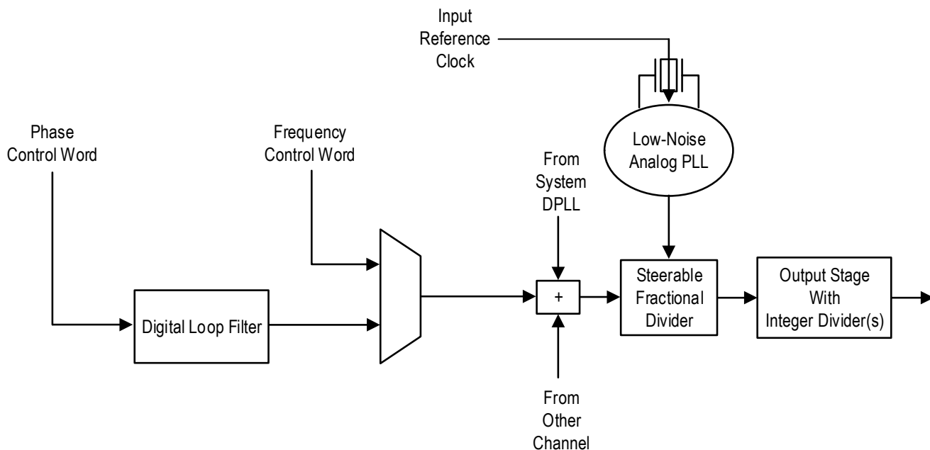
Figure 13. Satellite Channel Block Diagram
