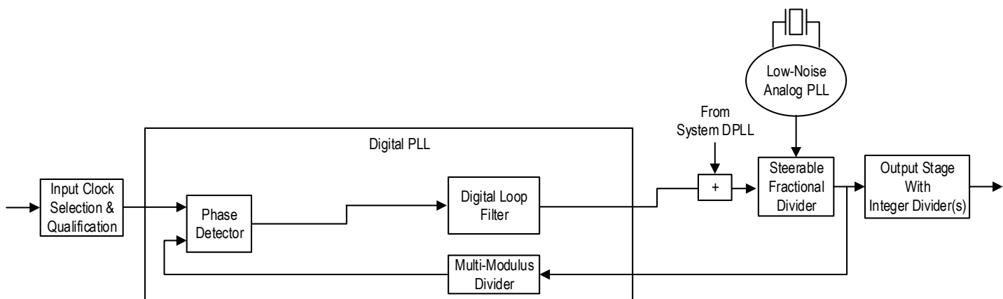
Figure 29. Jitter Attenuator Disciplined with Oscillator Operation
