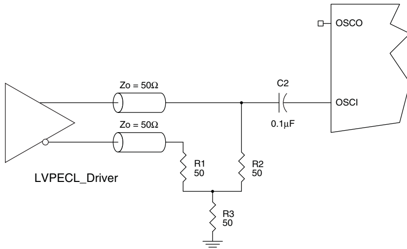
Figure 38. LVPECL Driver to XTAL Input Interface
