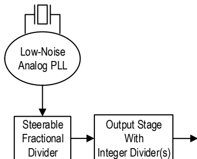
Figure 24. Free-Running Synthesizer Operation
