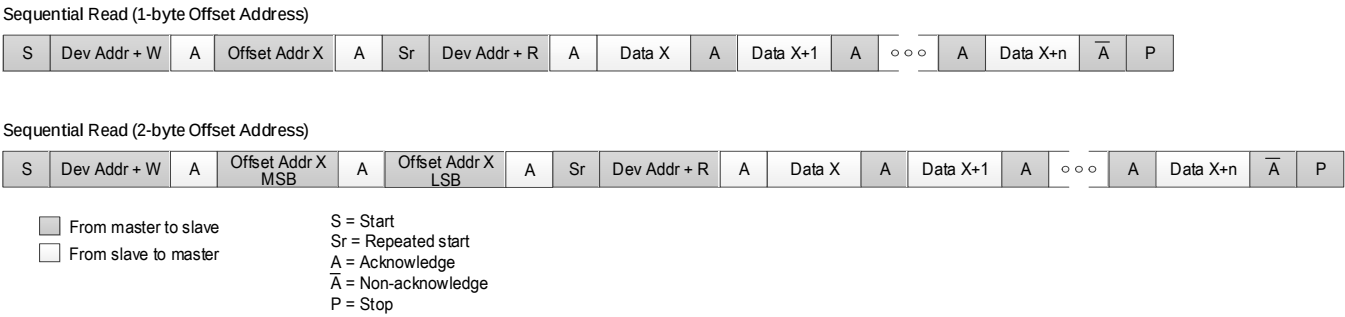
Figure 21. I 2 C Master Sequencing
