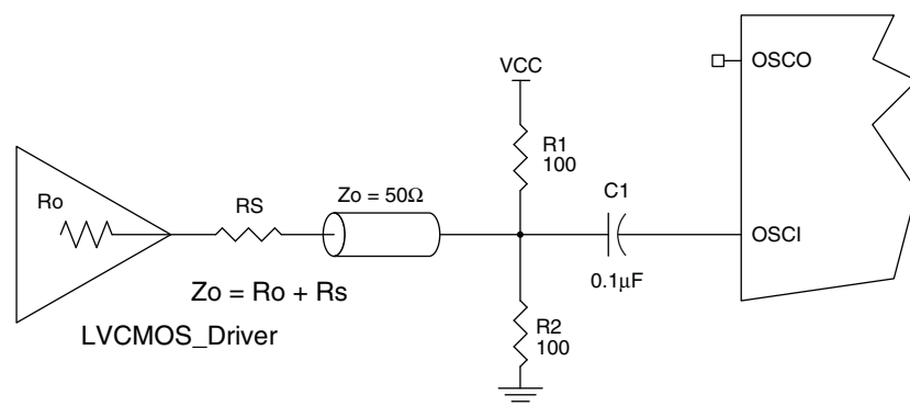
Figure 37. LVCMOS Driver to XTAL Input Interface
