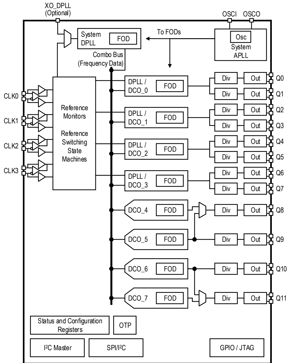
Figure 1. Block Diagram
