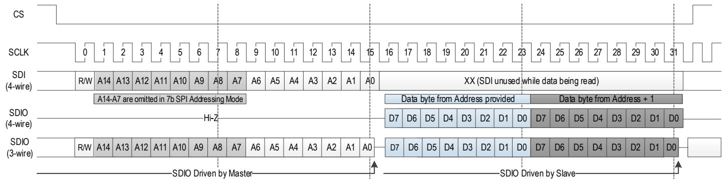
Figure 22. SPI Sequencing
