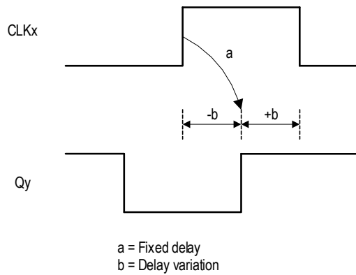
Figure 34. Input-Output Delay
