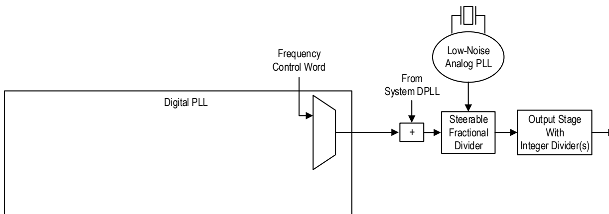
Figure 30. External DCO Control via Frequency Control Word
