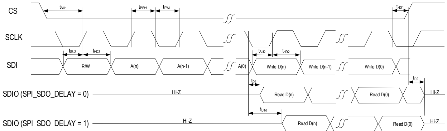
Figure 23. SPI Timing Diagram
