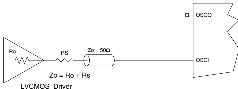
Figure 36. 1.8V LVCMOS Driver to XTAL Input Interface
