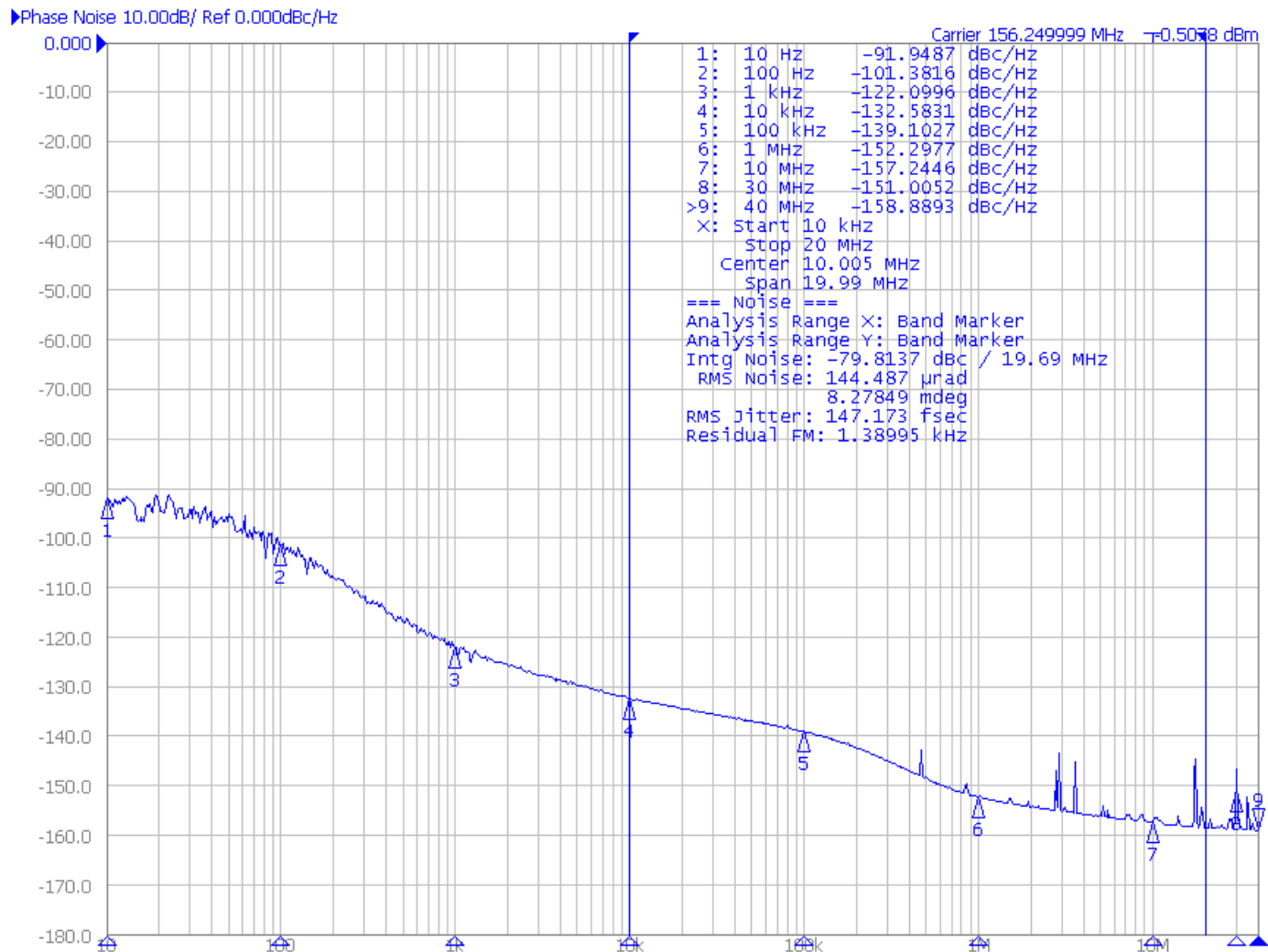
Figure 35. 156.25MHz Output Phase Noise
