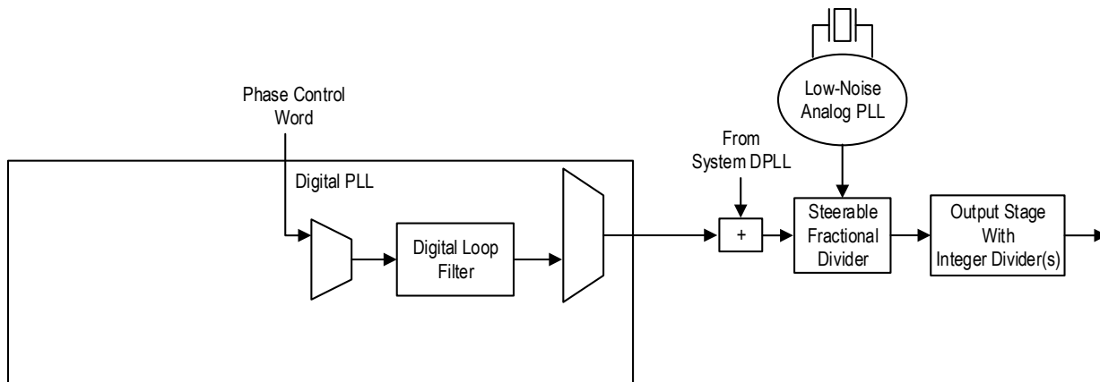
Figure 31. External DCO Control via Phase Control Word
