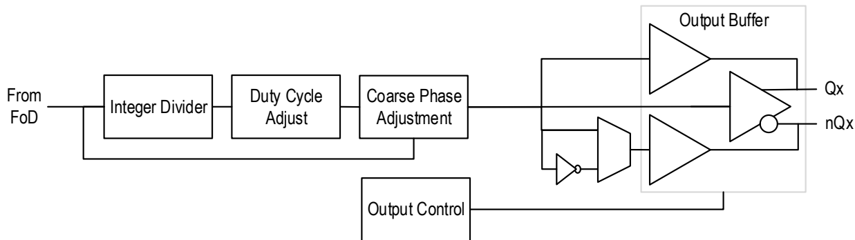
Figure 15. Single Output Stage
