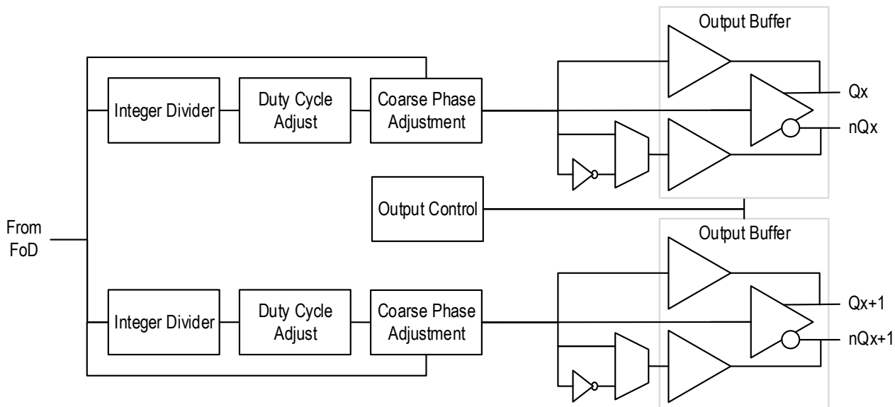
Figure 16. Dual Output Stage
