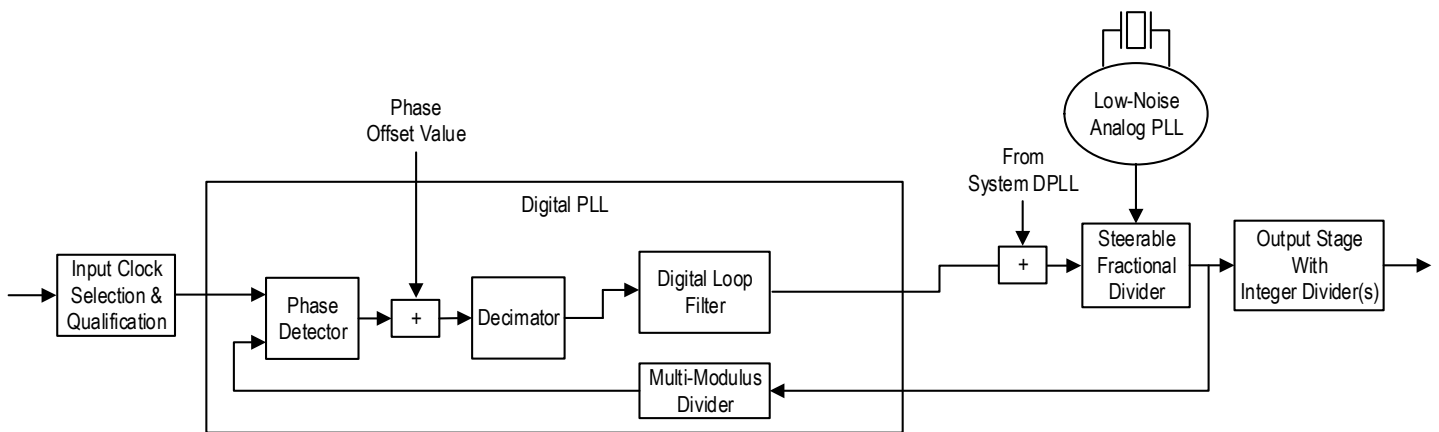
Figure 32. Phase Control in Closed Loop Operation
