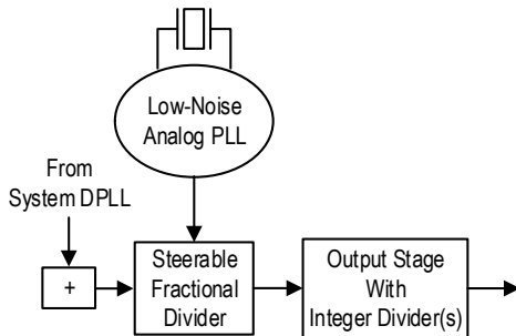
Figure 26. Synthesizer Disciplined with Oscillator Operation
