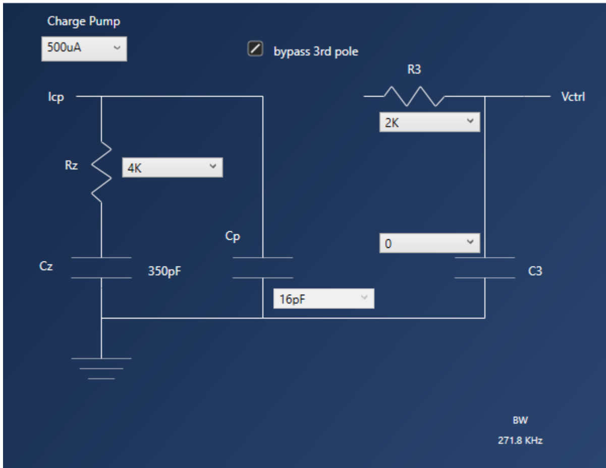
Figure 8. PLL Loop Filter Configuration Window
