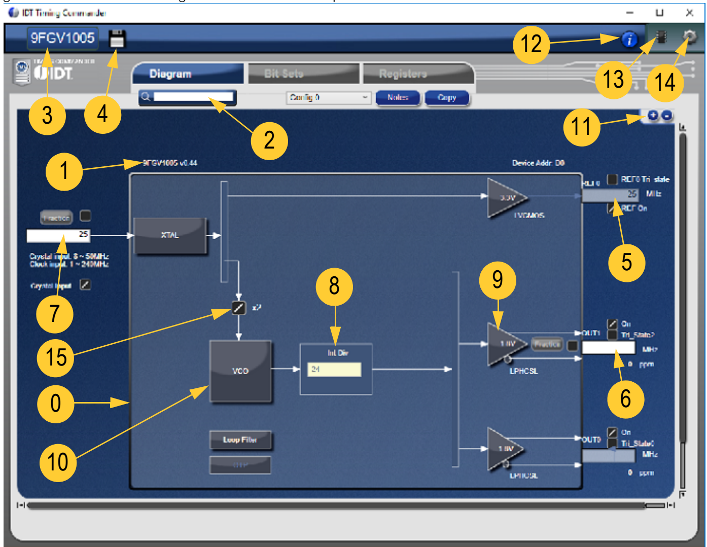
Figure 4. 9FGV1005 Settings File Window Descriptions
