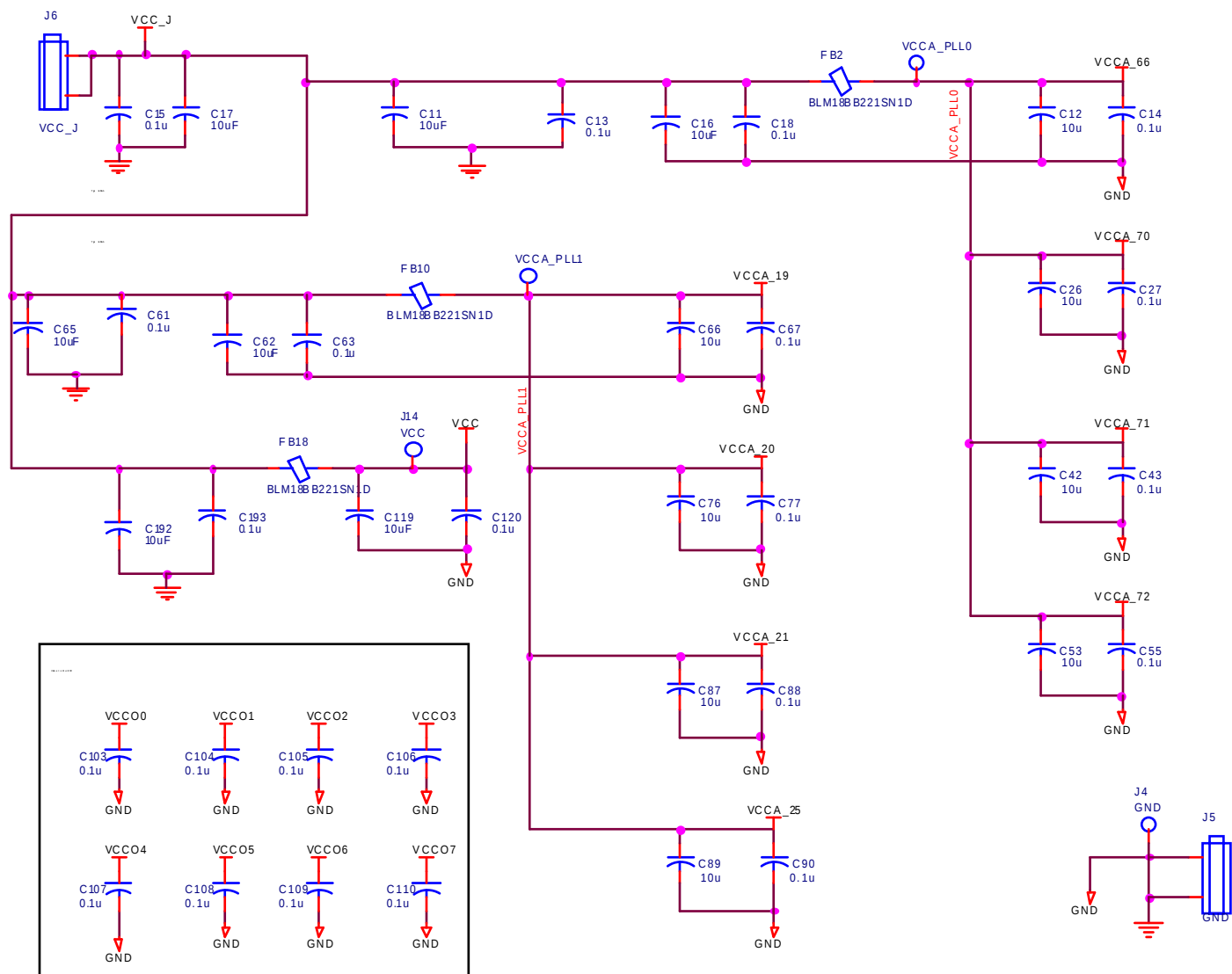
Figure 9. VCC Filtering
