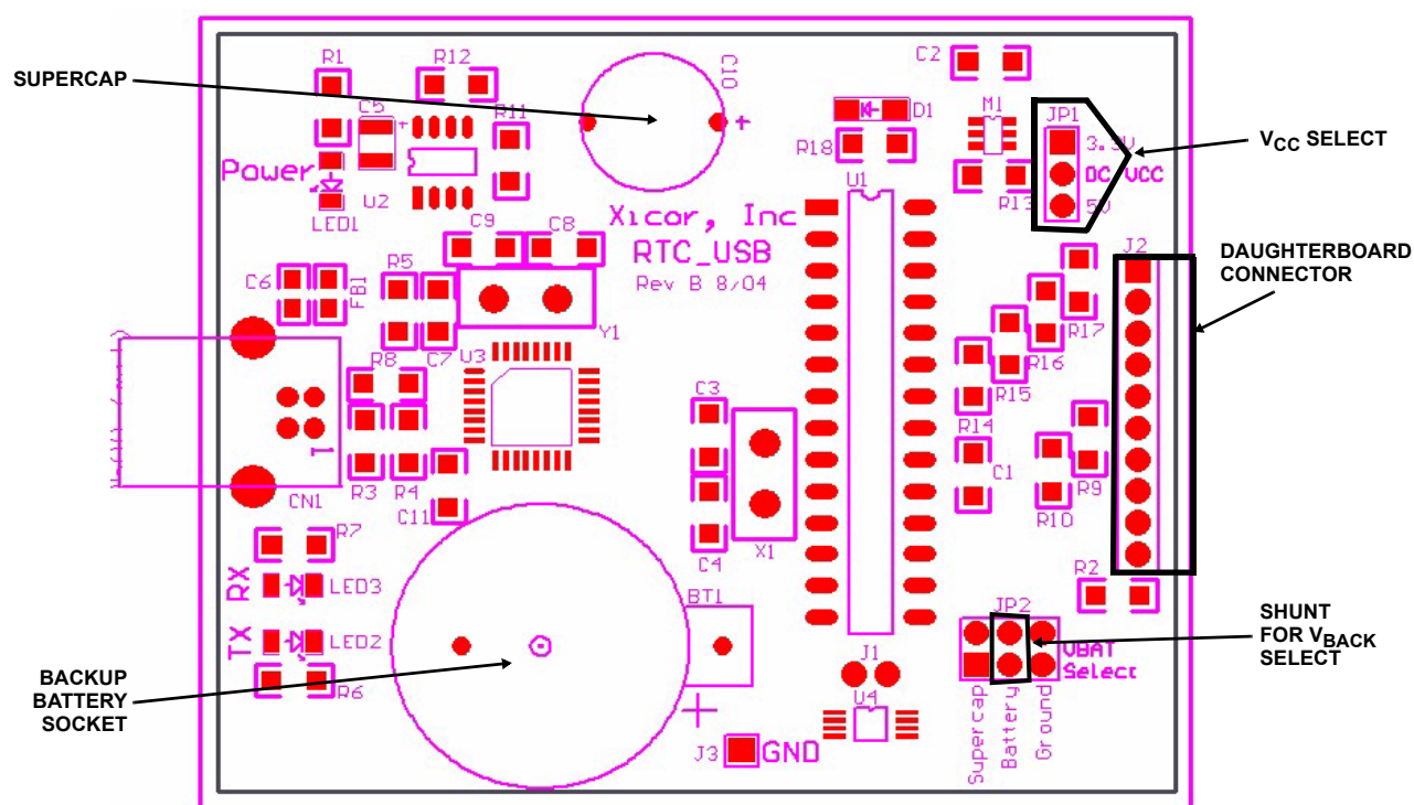
FIGURE 3. RTC-USB MOTHERBOARD LAYOUT
