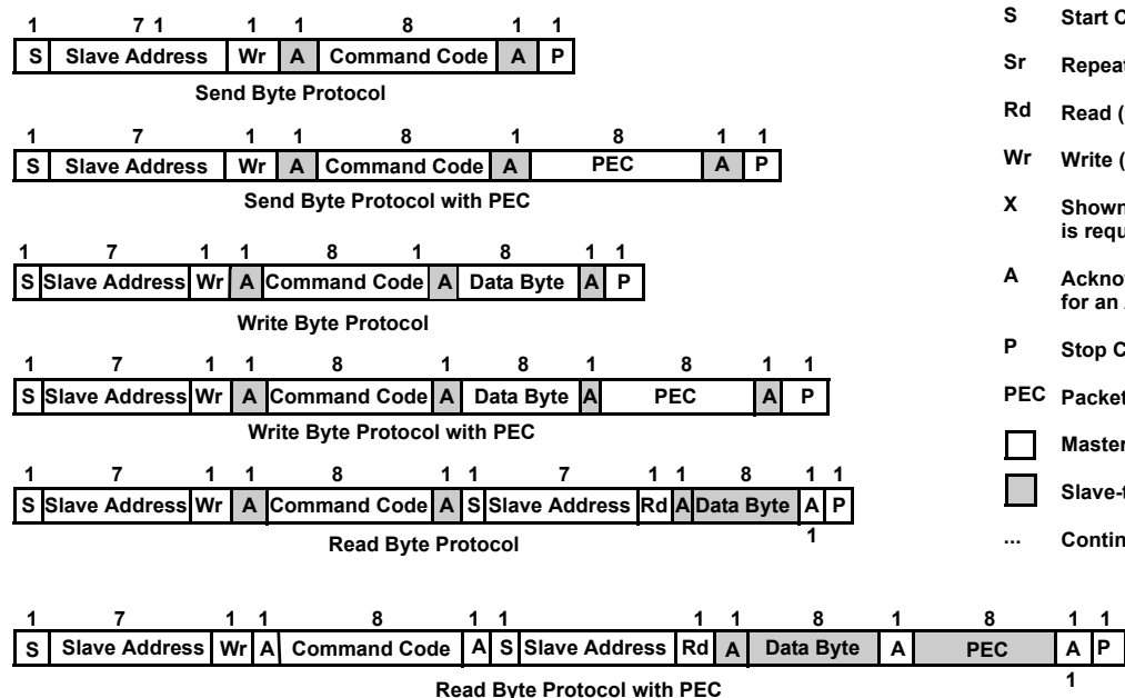
FIGURE 64. READ/WRITE SMBus PROTOCOLS WITH AND WITHOUT PEC
