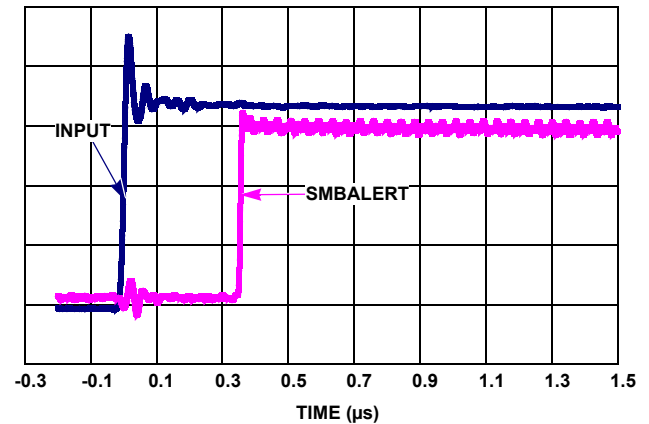
FIGURE 58. OV OR UV OR OC ALERT RESPONSE TIME
