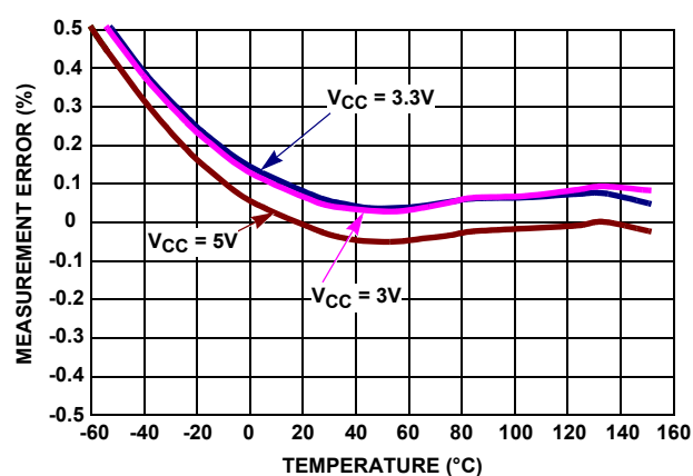
FIGURE 36. AUXILIARY V_{BUS} MEASUREMENT ERROR vs TEMPERATURE
