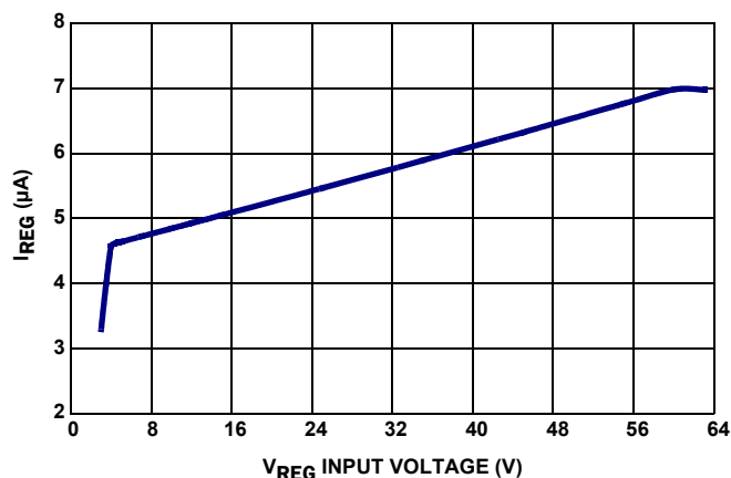
FIGURE 53. V_{REG} INPUT CURRENT vs INPUT VOLTAGE
