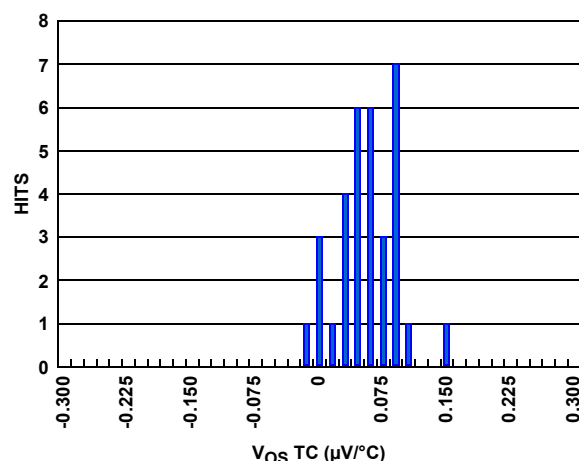
FIGURE 5. PRIMARY V_{SHUNT} V_{OS} TC ( -40^\circ\text{C} TO +125^\circ\text{C} )
