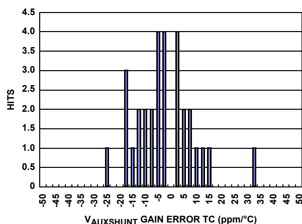
FIGURE 34. AUXILIARY V_{BUS} ADC GAIN ERROR TC
