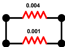
FIGURE 83. SIMPLIFIED SCHEMATIC ILLUSTRATING THE USE OF TWO SHUNT RESISTORS TO CREATE A DESIRED SHUNT VALUE
