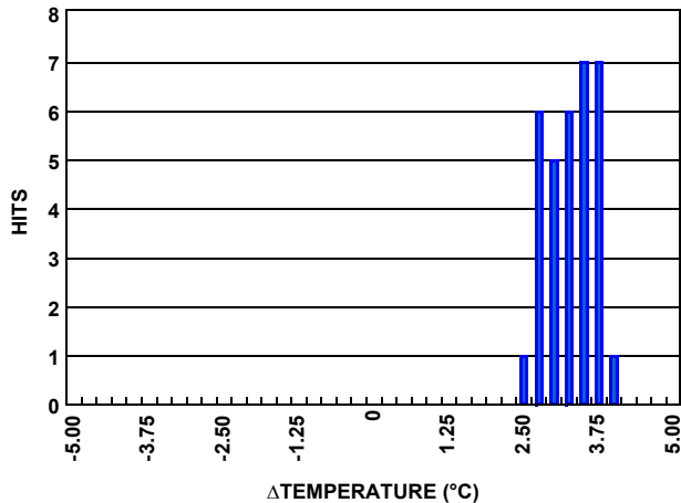
FIGURE 57. INTERNAL TEMPERATURE ACCURACY AT T = +25^\circ\text{C}
