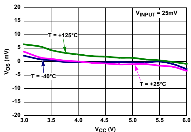
FIGURE 20. PRIMARY V_{BUS} V_{OS} vs V_{CC}
