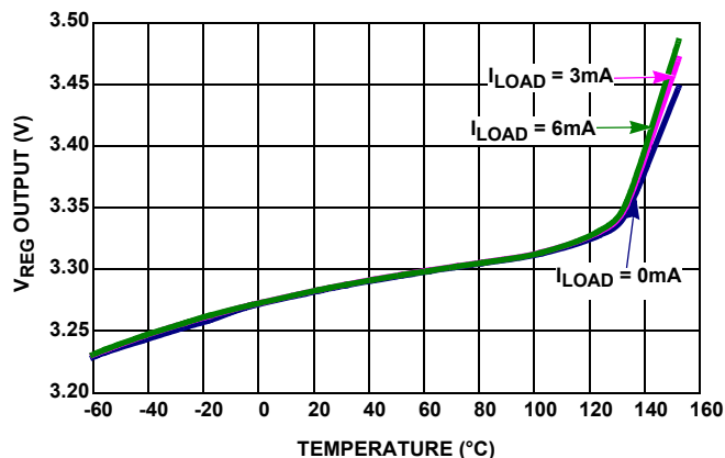
FIGURE 50. V_{REG} OUTPUT vs TEMPERATURE
