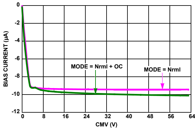
FIGURE 45. PRIMARY V_{SHUNT} BIAS CURRENT vs COMMON-MODE VOLTAGE
