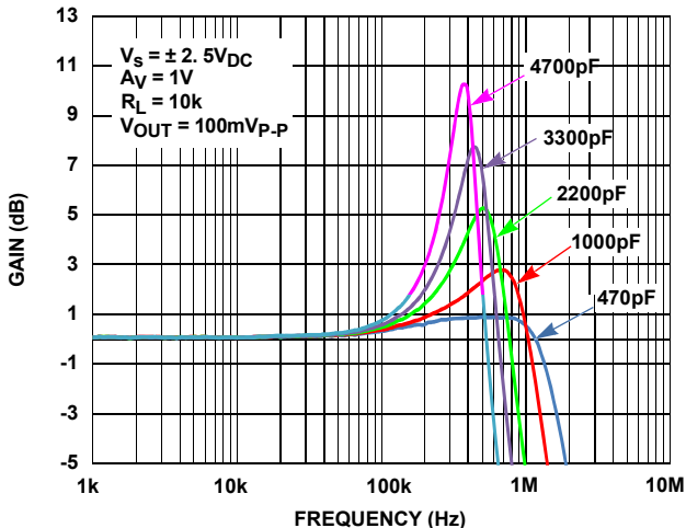
FIGURE 39. PGIA GAIN vs FREQUENCY vs CL, ISL2853x
