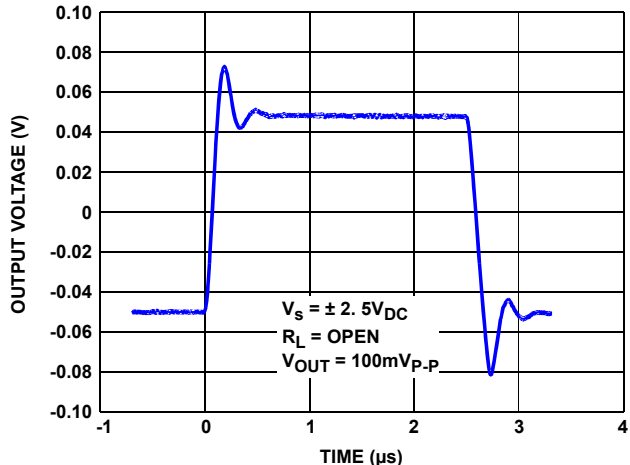
FIGURE 65. OP AMP SMALL SIGNAL TRANSIENT RESPONSE
