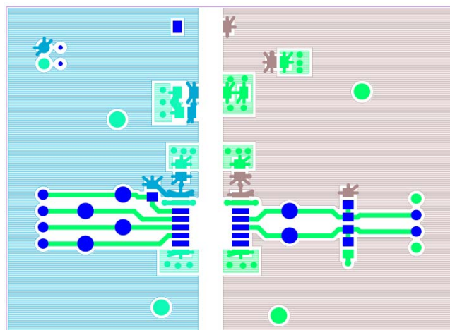
Figure 6. Top Layer
