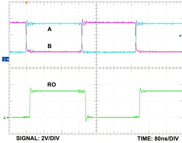
Figure 10. Receive Mode
