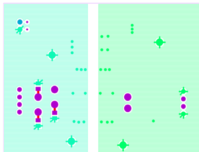
Figure 8. Bottom Layer
