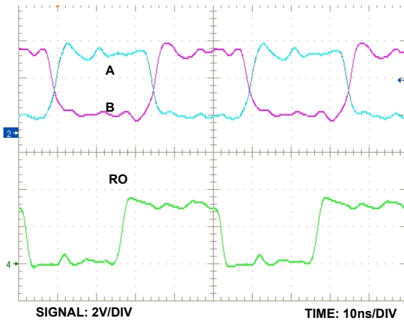
Figure 12. Receive Mode
