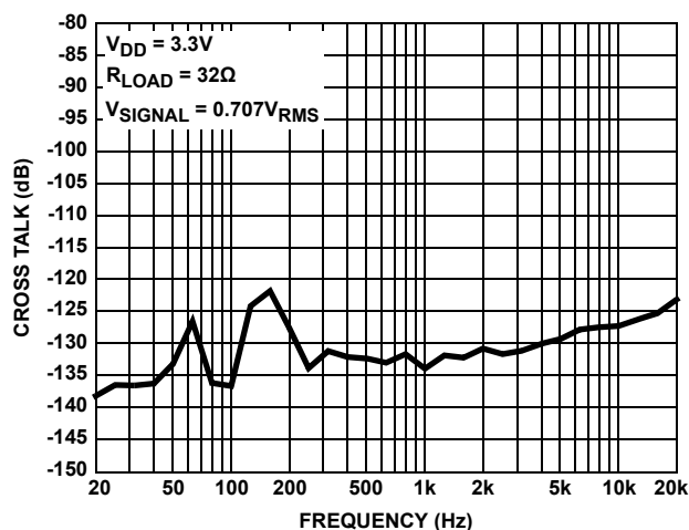
FIGURE 10. CHANNEL-TO-CHANNEL CROSSTALK
