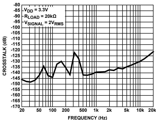
FIGURE 11. CHANNEL-TO-CHANNEL CROSSTALK
