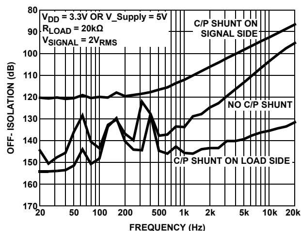
FIGURE 9. OFF-ISOLATION, 2VRMS SIGNAL, 20kΩ LOAD
