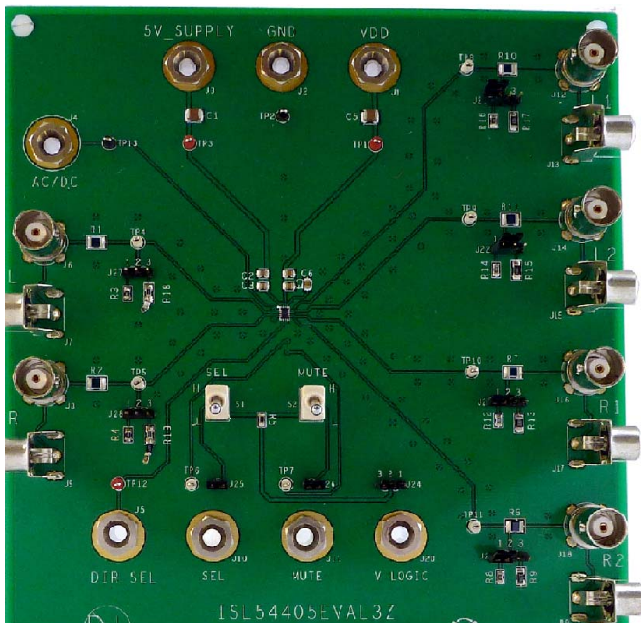
FIGURE 4. TOP SIDE
