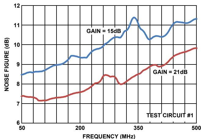
FIGURE 6. NOISE FIGURE
