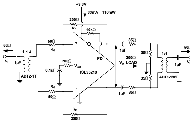
FIGURE 28. TEST CIRCUIT #1
