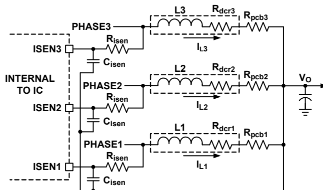
FIGURE 17. CURRENT BALANCING CIRCUIT
