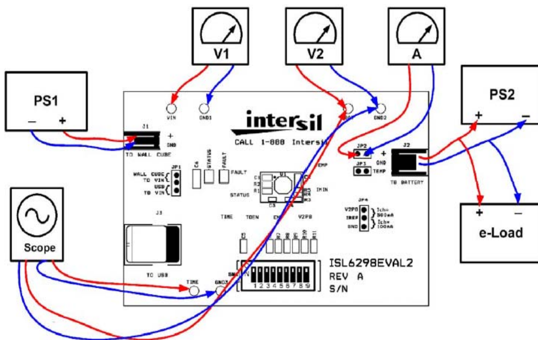
FIGURE 2. CONNECTION OF INSTRUMENTS
