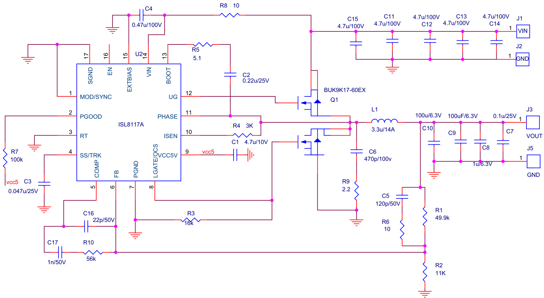
FIGURE 6. ISL8117ADEMO1Z SCHEMATIC
