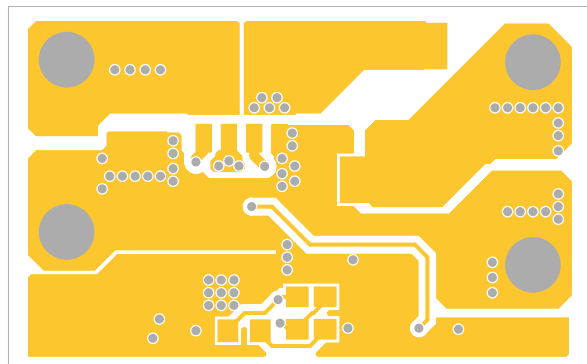
FIGURE 11. BOTTOM LAYER
