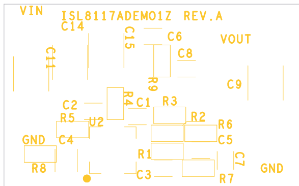
FIGURE 7. SILKSCREEN TOP
