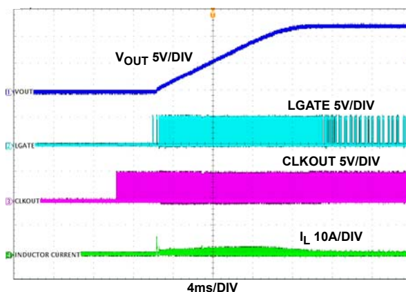
FIGURE 17. DEM START-UP WAVEFORMS: V_{IN} = 48V , I_O = 0A
