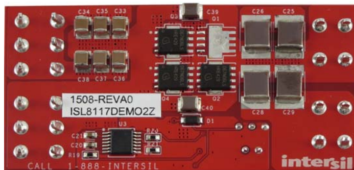
FIGURE 2. ISL8117DEMO2Z DEMONSTRATION BOARD BOTTOM
