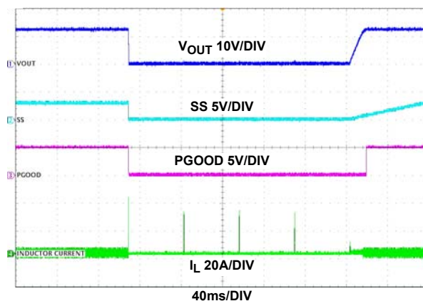
FIGURE 23. SHORT-CIRCUIT WAVEFORMS, V_{IN} = 48V
