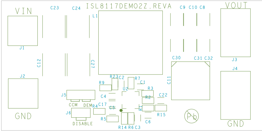
FIGURE 29. SILKSCREEN TOP
