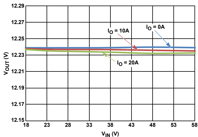
FIGURE 11. CCM MODE LINE REGULATION
