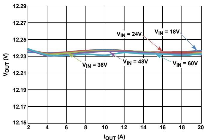
FIGURE 10. CCM MODE LOAD REGULATION
