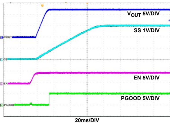
FIGURE 19. DEM START-UP WAVEFORMS: V_{IN} = 48V , I_O = 0A
