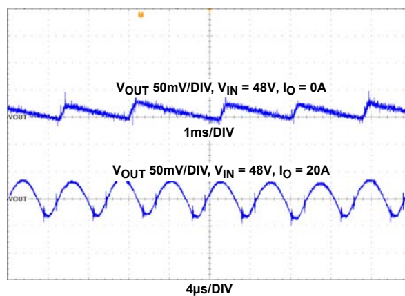
FIGURE 15. OUTPUT RIPPLE, DEM MODE
