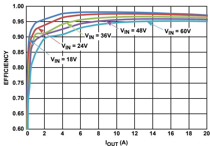
FIGURE 9. DEM EFFICIENCY vs LOAD
