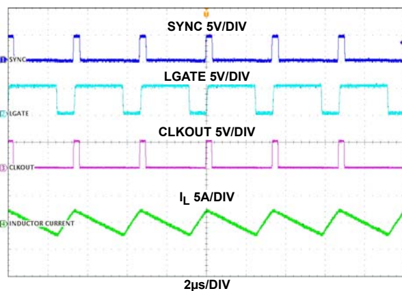
FIGURE 21. FREQUENCY SYNCHRONIZATION WAVEFORMS, V_{IN} = 48V , I_O = 0A
