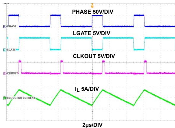
FIGURE 13. PHASE, LGATE, CLKOUT AND INDUCTOR CURRENT WAVEFORMS, V_{IN} = 48V , I_O = 0A
