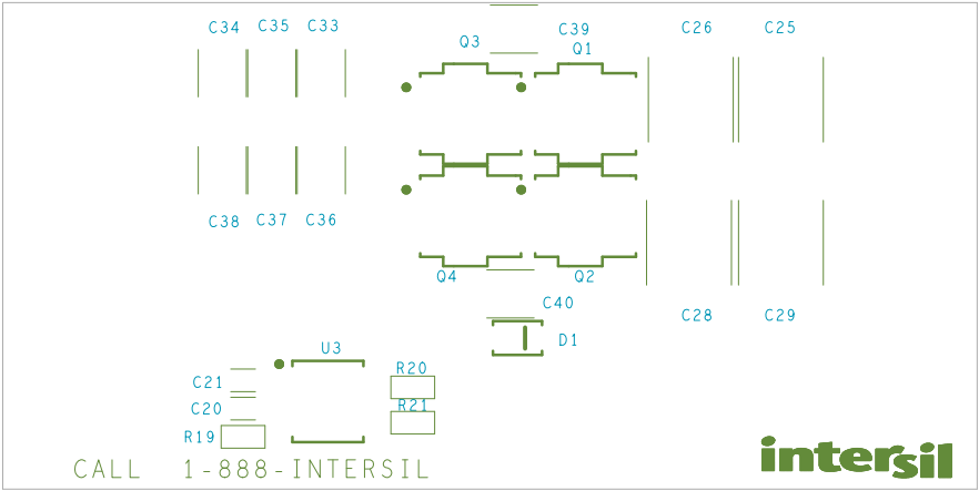
FIGURE 30. SILKSCREEN BOTTOM
