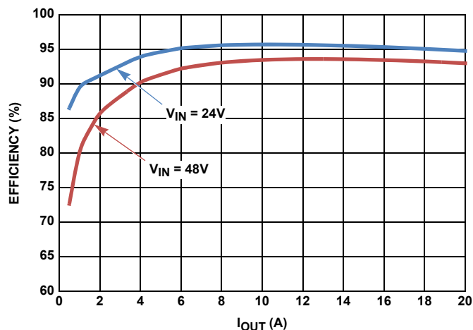
FIGURE 6. DEM EFFICIENCY vs LOAD, V_{OUT} = 5V
