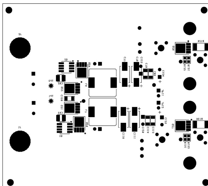
FIGURE 10. BOTTOM SILKSCREEN
