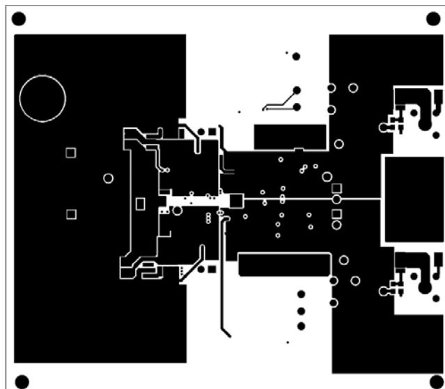
FIGURE 8. BOTTOM LAYER
