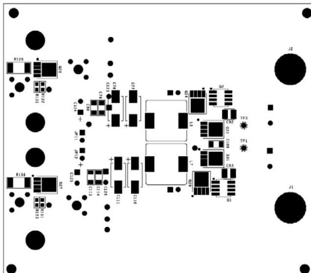
FIGURE 9. BOTTOM SILKSCREEN (MIRRORED)
