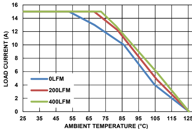
Figure 14. Derating Curve, V_{OUT} = 3.3V , C_{OUT} = 4 \times 100\mu F Ceramic + 1 \times 470\mu F POSCAP
