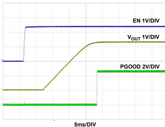
Figure 12. Start-Up Waveform, V_{OUT} = 3.3V , I_{OUT} = 15A , C_{OUT} = 4 \times 100\mu F Ceramic + 1 \times 470\mu F POSCAP
