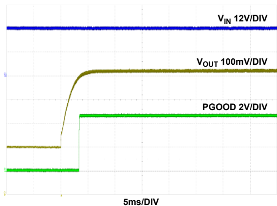
Figure 13. Prebiased Power-Up Waveform, Prebiased Voltage = 3.0V , V_{OUT} = 3.3V , I_{OUT} = \text{No Load} , C_{OUT} = 4 \times 100\mu F Ceramic + 1 \times 470\mu F POSCAP
