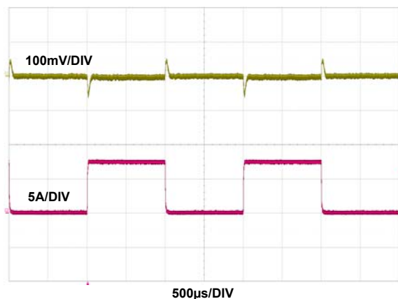
Figure 11. Transient Response, V_{OUT} = 3.3V , 0A to 7.5A , 2.5A/\mu s Step Load, C_{OUT} = 4 \times 100\mu F Ceramic + 1 \times 470\mu F POSCAP
