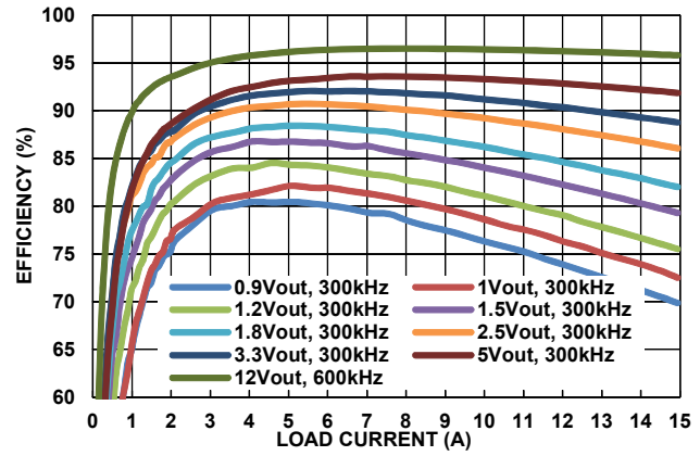
Figure 6. Efficiency vs Load Current at V_{IN} = 24V , CCM Mode
