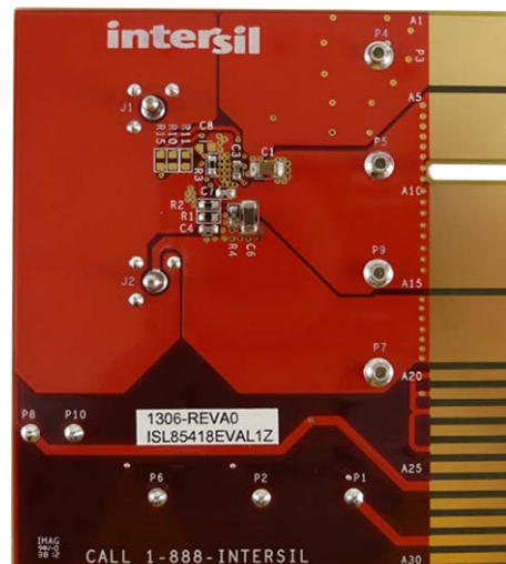
FIGURE 7. BACK OF EVALUATION BOARD ISL85418EVAL1Z
