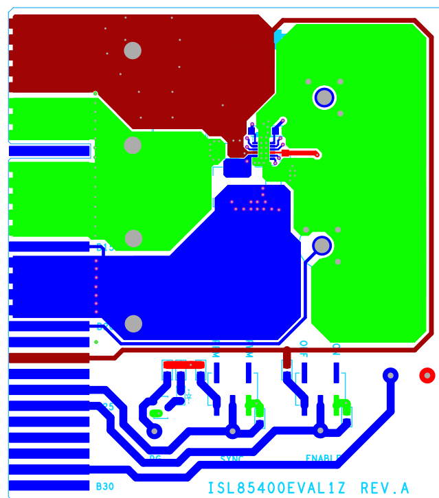
FIGURE 12. LAYER 1
