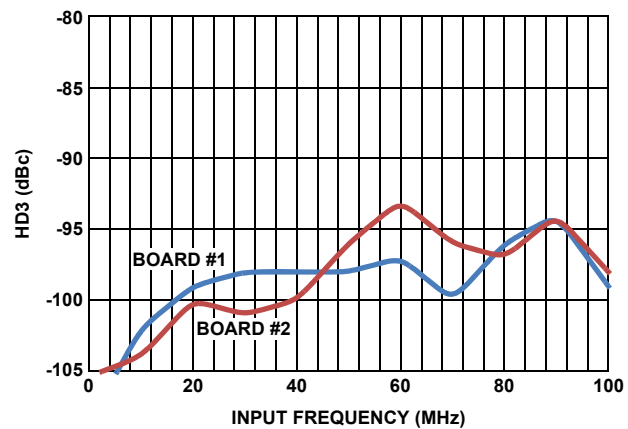
FIGURE 36. 350MSPS HD3
