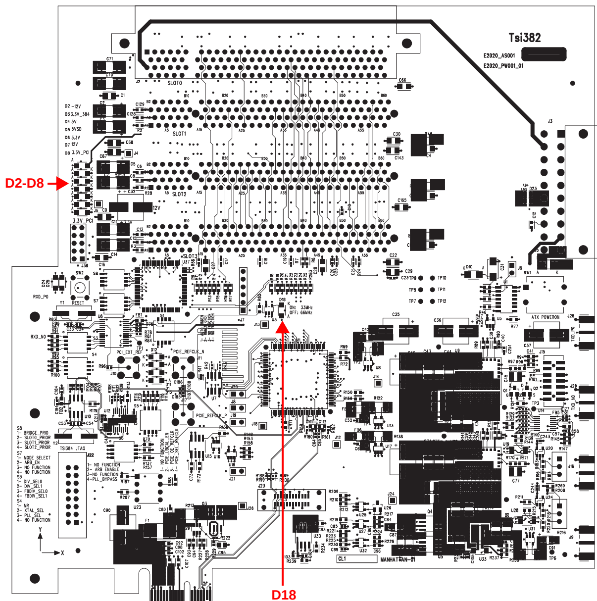
Figure 10: LED Locations
