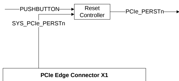
Figure 4: Board Reset
