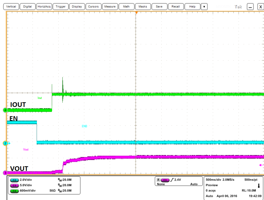
Figure 14. 600mA Full Load Start-up by Rx Enable Signal (Ch2=EN, Ch3=Vout, Ch4=Iout)
