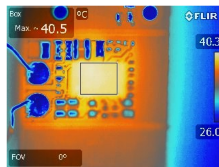
P9027LP-R: 40.5 Degree C
