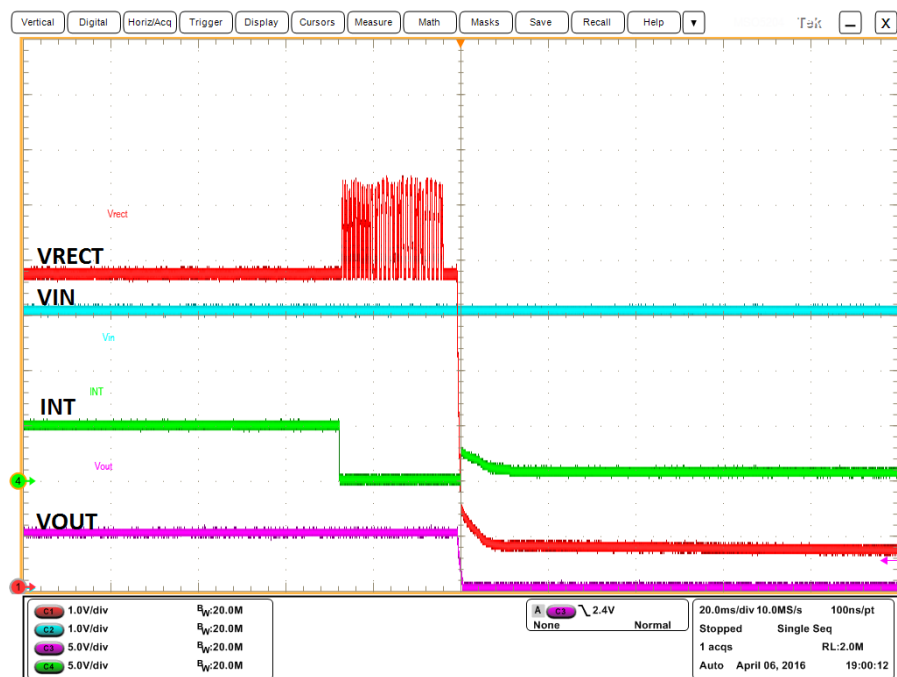
Figure 15. Rx Over Temperature Protection (Ch1=Vrect, Ch2=Vin, Ch3=Vout, Ch4=INT)
