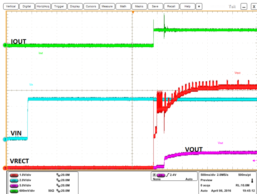
Figure 12. 600mA Full Load Start-up by Tx Input Power (Ch1=Vrect, Ch2=VIN, Ch3=Vout,Ch4=Iout)
