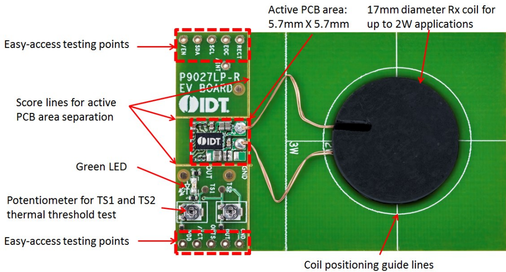
Figure 2. P9027LP-R-EVK Reference Board Illustration Top Layer
