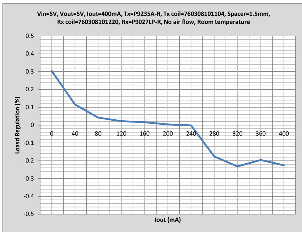
Figure 8. Load Regulation for 20mm Coil
