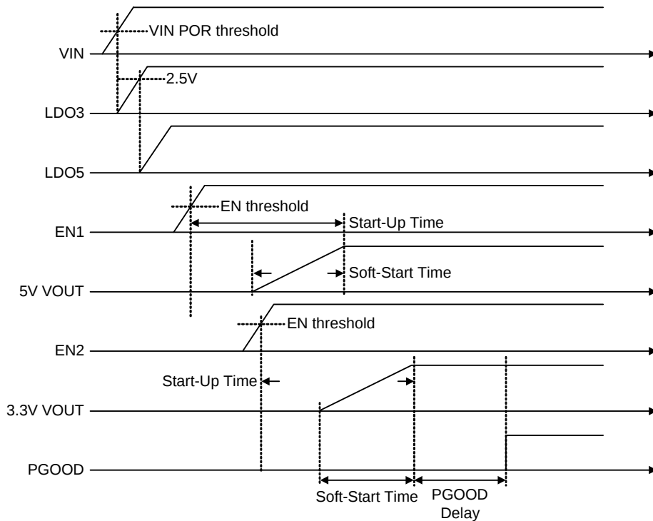
Figure 6. RT6576B Timing
