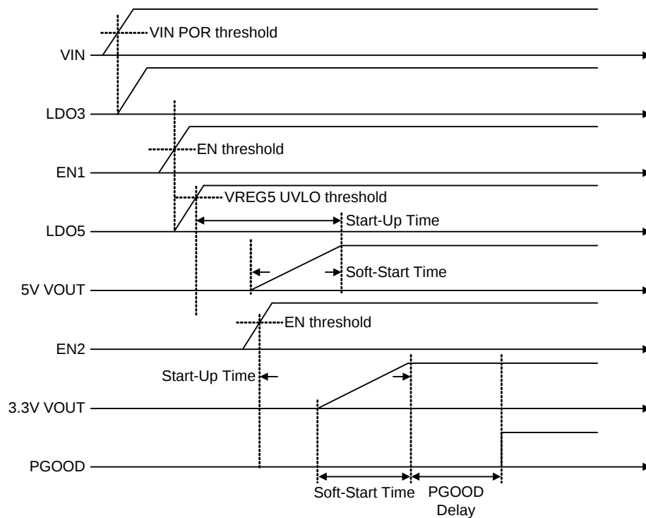
Figure 5. RT6576A Timing
