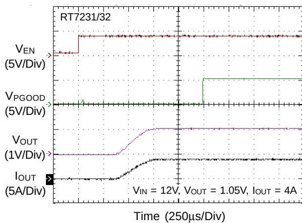
Power Good from EN Turn On
