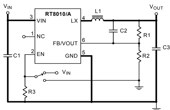
Figure 6. EVB Schematic
