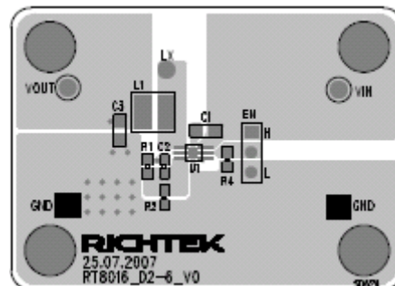
Figure 7. Top Layer
