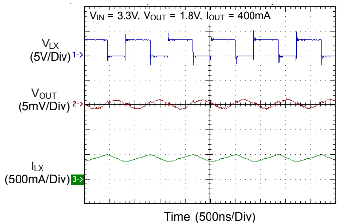
Output Ripple
