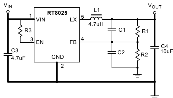
Figure 6. EVB Schematic
