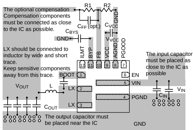
Figure 4. PCB Layout Guide
