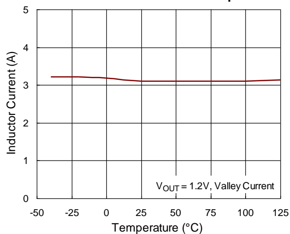
Inductor Current Limit vs. Temperature
