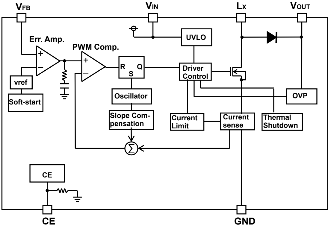
●R1207N8xxB/C
