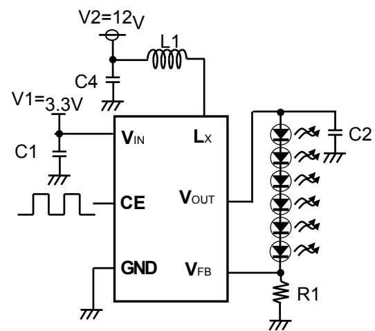
Fig 2. R1207N8xxB/C
