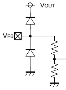
VFB Pin Equivalent Circuit Diagram (R1155x001C)
