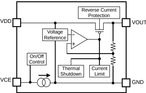
R1155xxxxB Block Diagram (Fixed Output Voltage Type)
