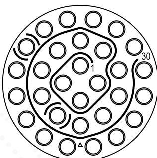
30 #16 contacts Insert 24-30
