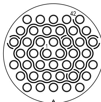
42 #16 contacts Insert 28-42
