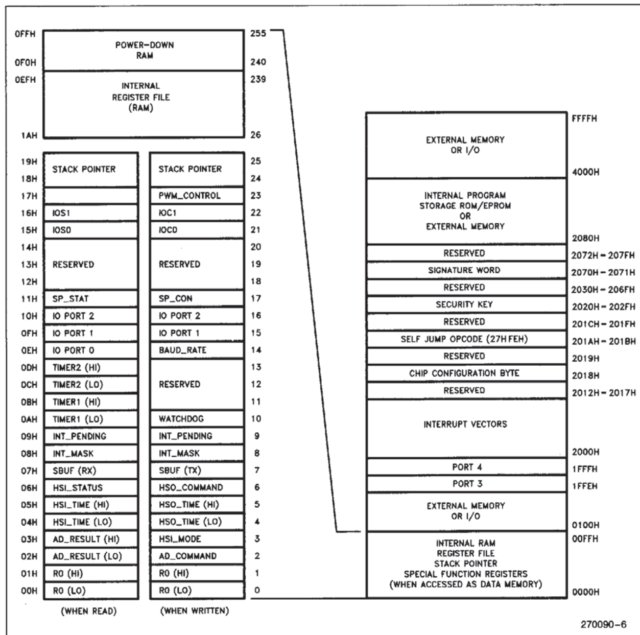
Figure 2. 8X9XBH Memory Map
