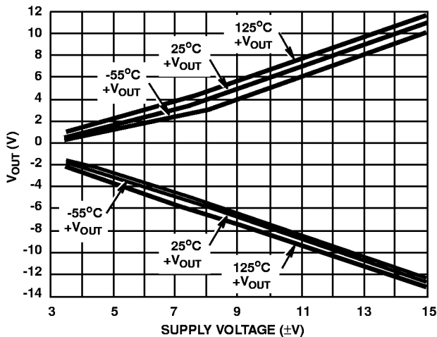
FIGURE 9. OUTPUT VOLTAGE SWING vs SUPPLY VOLTAGE
