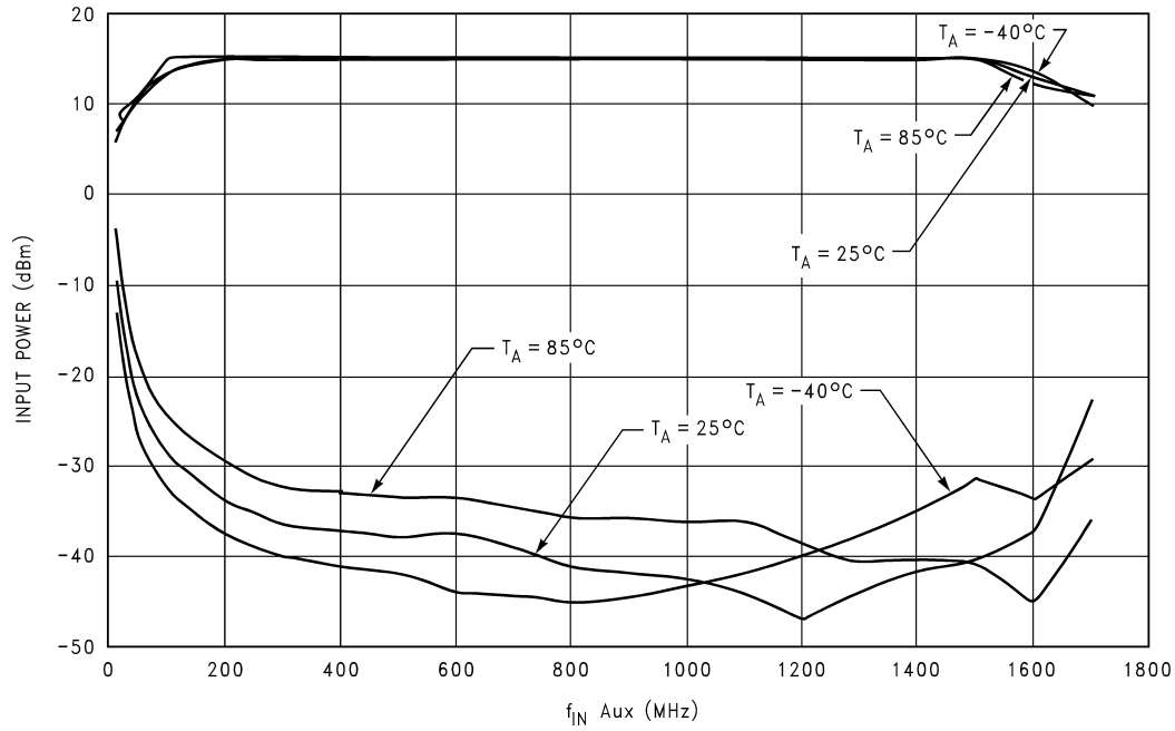
LMX2377U f_{IN} Aux Input Power Vs Frequency V_{CC} = V_P \text{ Aux} = V_{\mu C} = 3.0V
