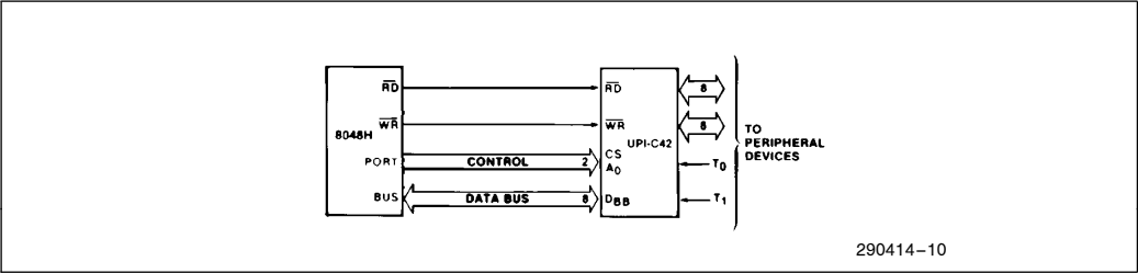
Figure 9. 8048H-UPI-C42 Interface
