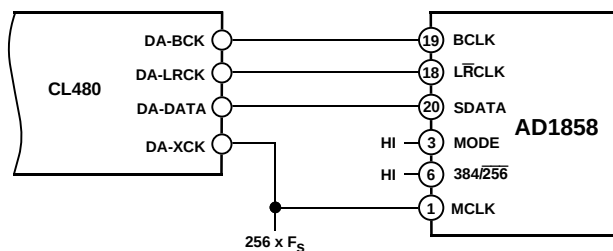
Figure 20. Interface to CL480
