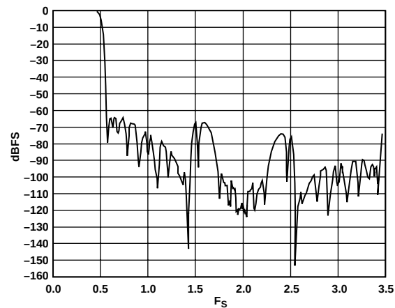
Figure 7. Digital Filter Signal Transfer Function to 3.5 × F S
