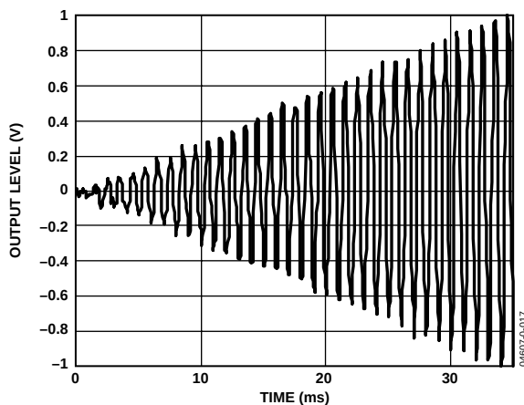
Figure 15. Slew RAM—Linear Update Increasing Ramp
