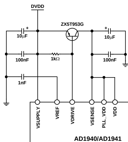
Figure 29. Voltage Regulator Design
