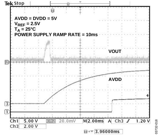
Figure 18. Power-Up Transient
