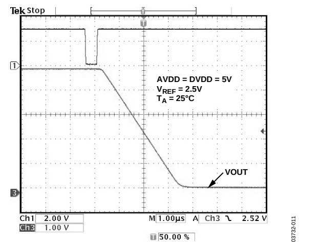
Figure 11. Slew Rate with Boost Off
