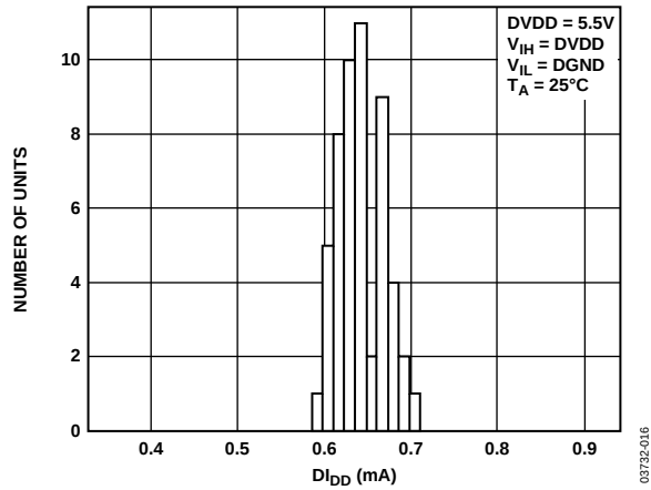
Figure 16. I_{DD} Histogram
