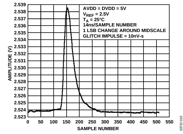
Figure 10. AD5381-5 Glitch Impulse
