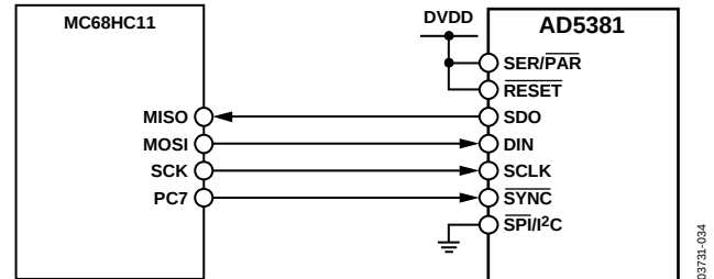
Figure 34. AD5381-to-MC68HC11 Interface
