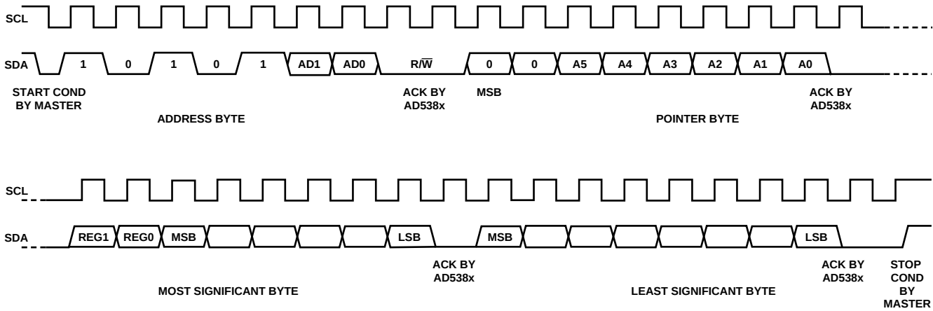
Figure 31. 4-Byte AD5381, I 2 C Write Operation
