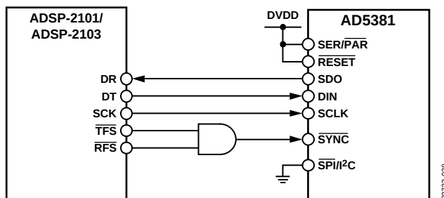
Figure 38. AD5381-to-ADSP-2101/ADSP-2103 Interface
