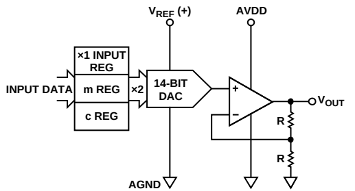
Figure 26. Single-Channel Architecture
