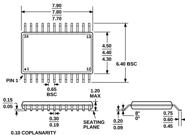
Figure 50. 24-Lead Thin Shrink Small Outline Package [TSSOP] (RU-24)
