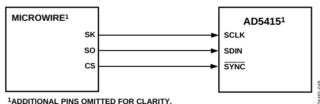
Figure 48. MICROWIRE-to-AD5415 Interface
