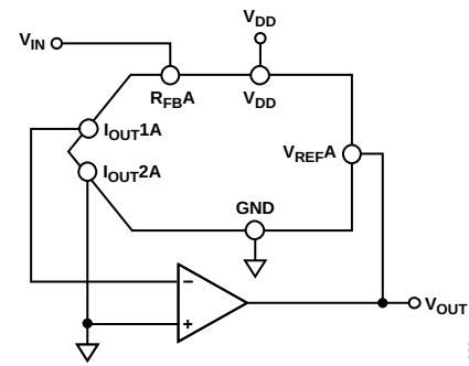
Figure 39. Current-Steering DAC Used as a Divider or Programmable Gain Element
