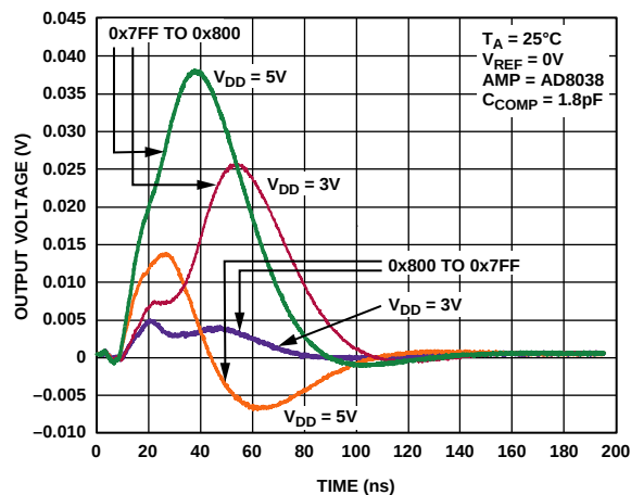
Figure 19. Midscale Transition, V_{REF} = 0V
