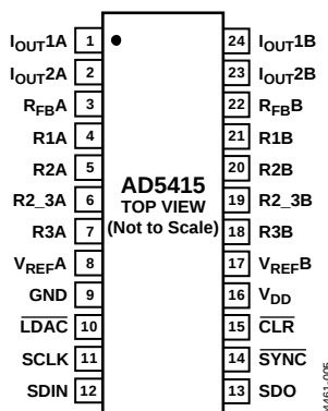
Figure 6. Pin Configuration
