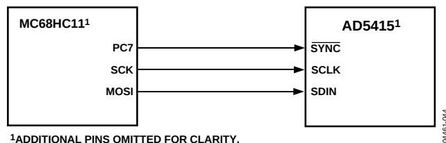
Figure 47. MC68HC11-to-AD5415 Interface
