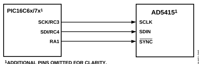
Figure 49. PIC16C6x/7x-to-AD5415 Interface
