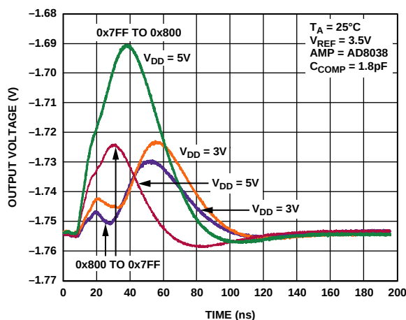
Figure 20. Midscale Transition, V_{REF} = 3.5V
