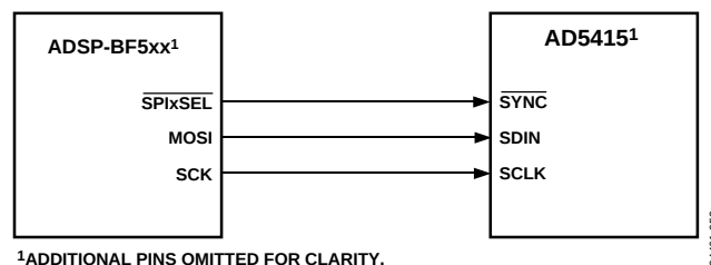
Figure 44. ADSP-BF5xx-to-AD5415 Interface
