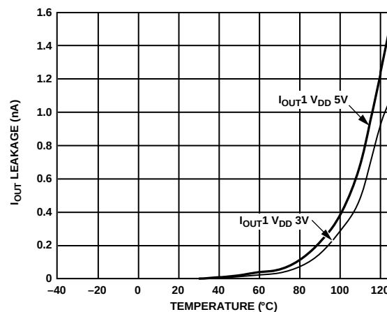
Figure 22. IOUT1 Leakage Current vs. Temperature
